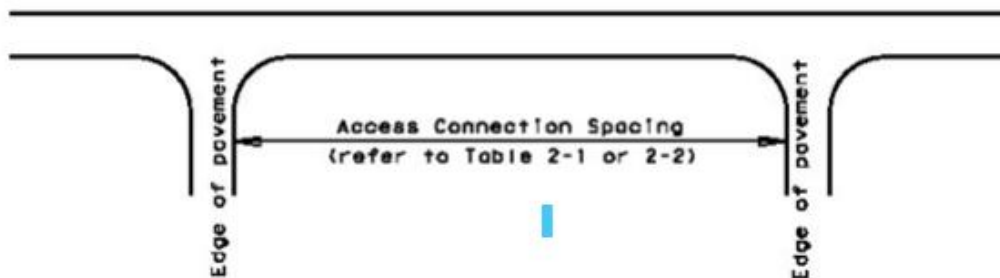
Figure 4. Access Connection Spacing Diagram (Source: TxDot Manuals)
