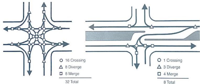
Figure 2. Vehicular Conflict Points at a Typical Four-Way Intersection v. a Directional Median Opening
