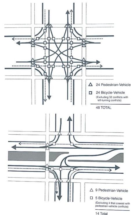
Figure 3. Bicycle and Pedestrian Conflict Points
