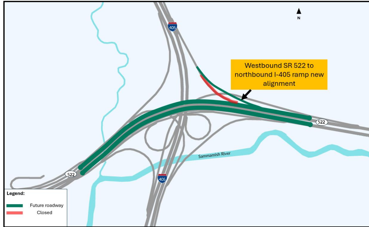
Future alignment for SR 522 general purpose lanes and westbound SR 522 ramp to northbound I-405.
