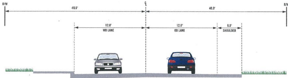
EXISTING ROADWAY SECTION—NE 153RD PL
