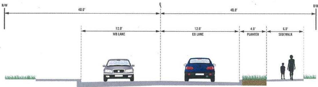
PROPOSED ROADWAY SECTION—NE 153RD PL
