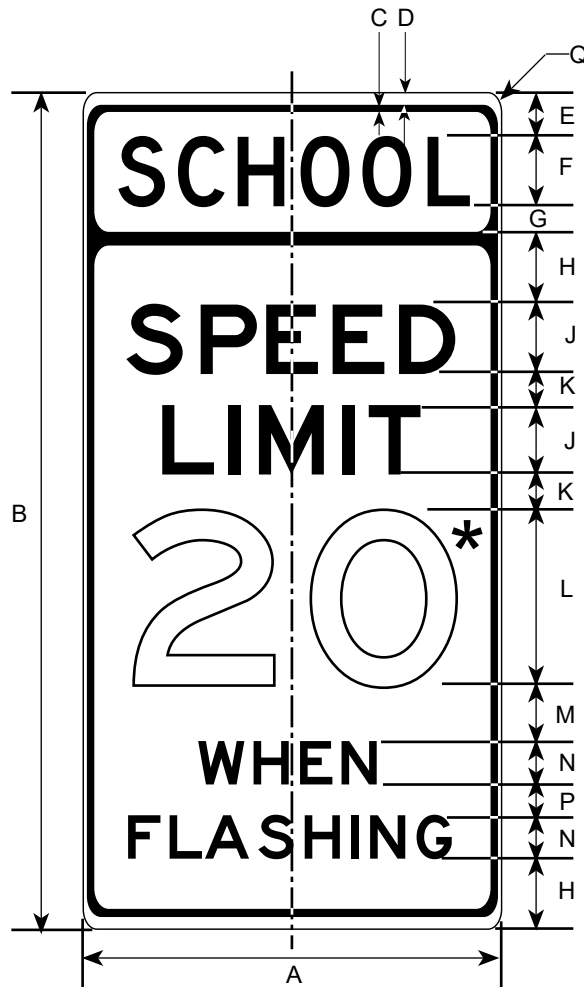
SCHOOL SPEED LIMIT SIGN (FOR USE WITH FLASHING BEACON)
