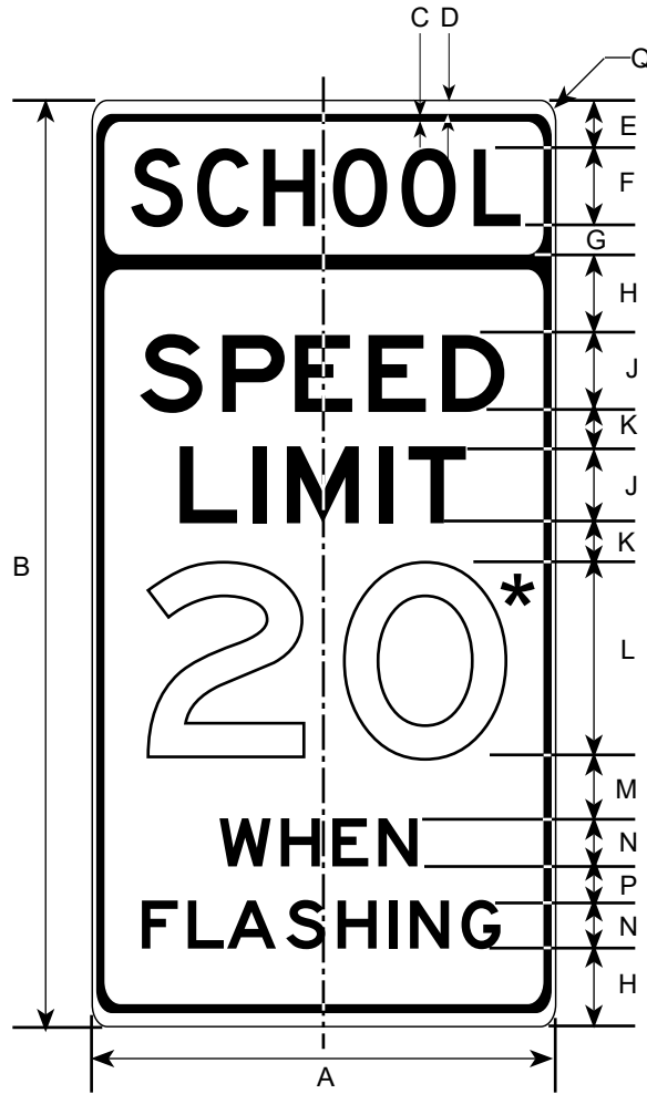
SCHOOL SPEED LIMIT SIGN (FOR USE WITH FLASHING BEACON)
