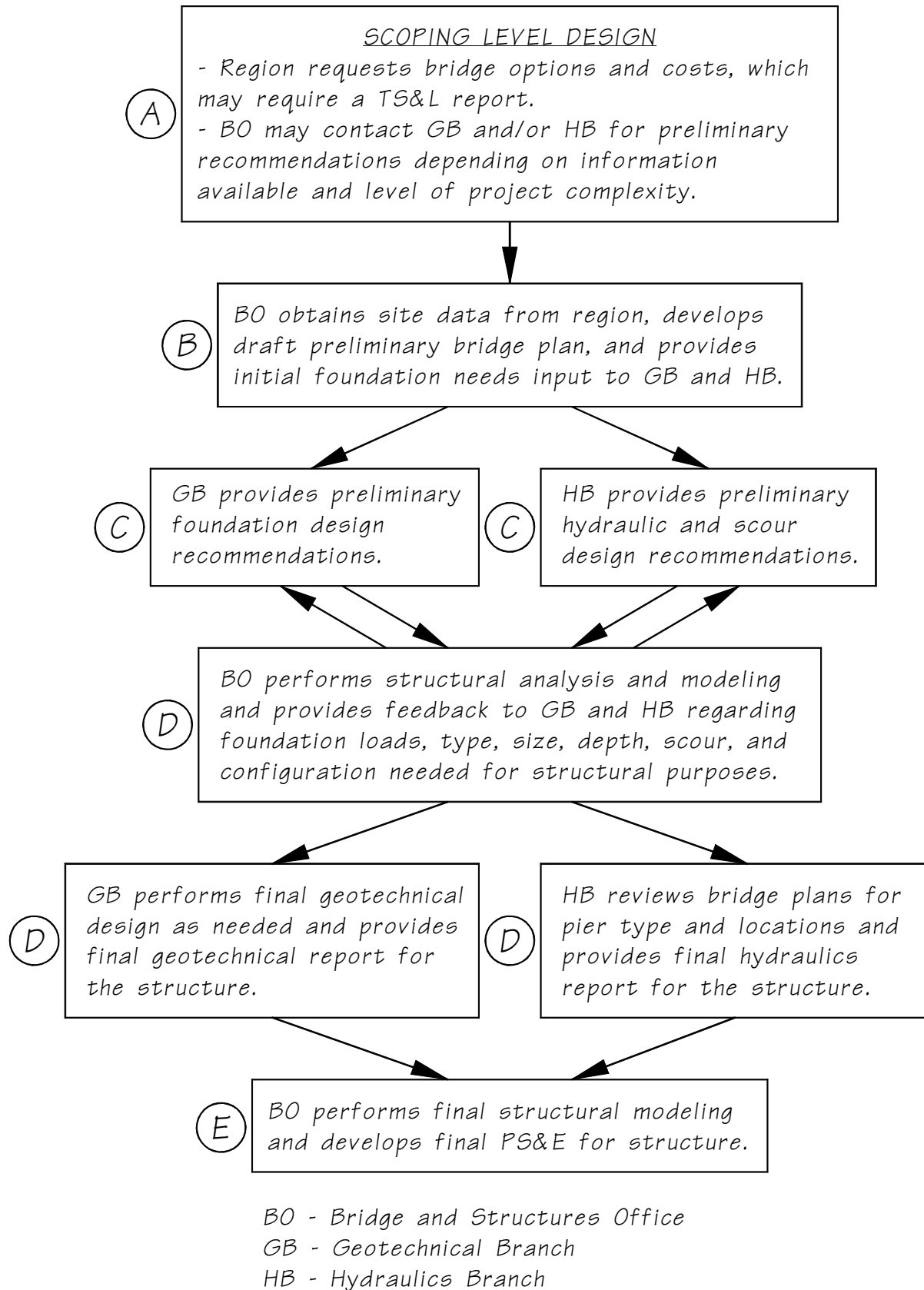
Figure 7.1.1-1 Overall Design Process for LRFD Foundation Design
