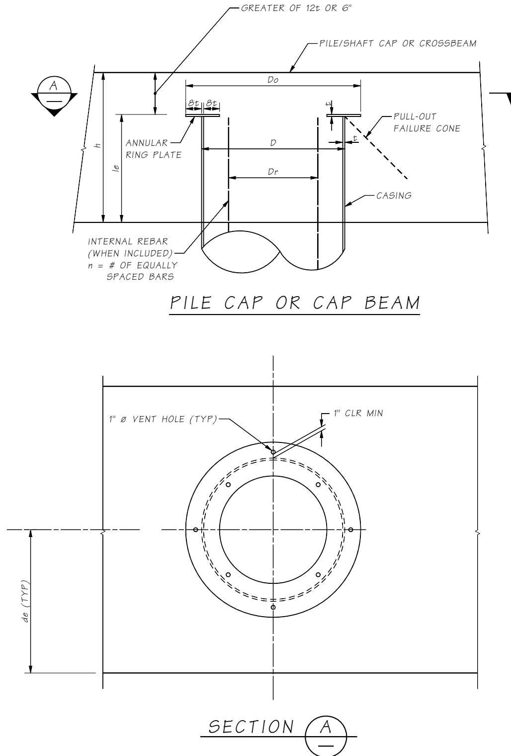
Figure 7.10.3-1 Annular Ring Connections
