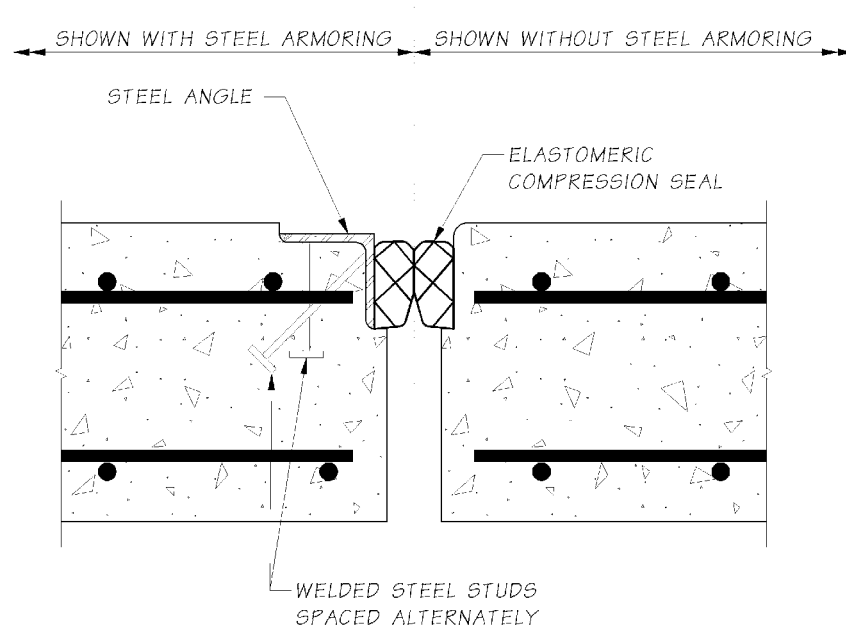
Figure 9.1.3-1 Compression Seal Joint
