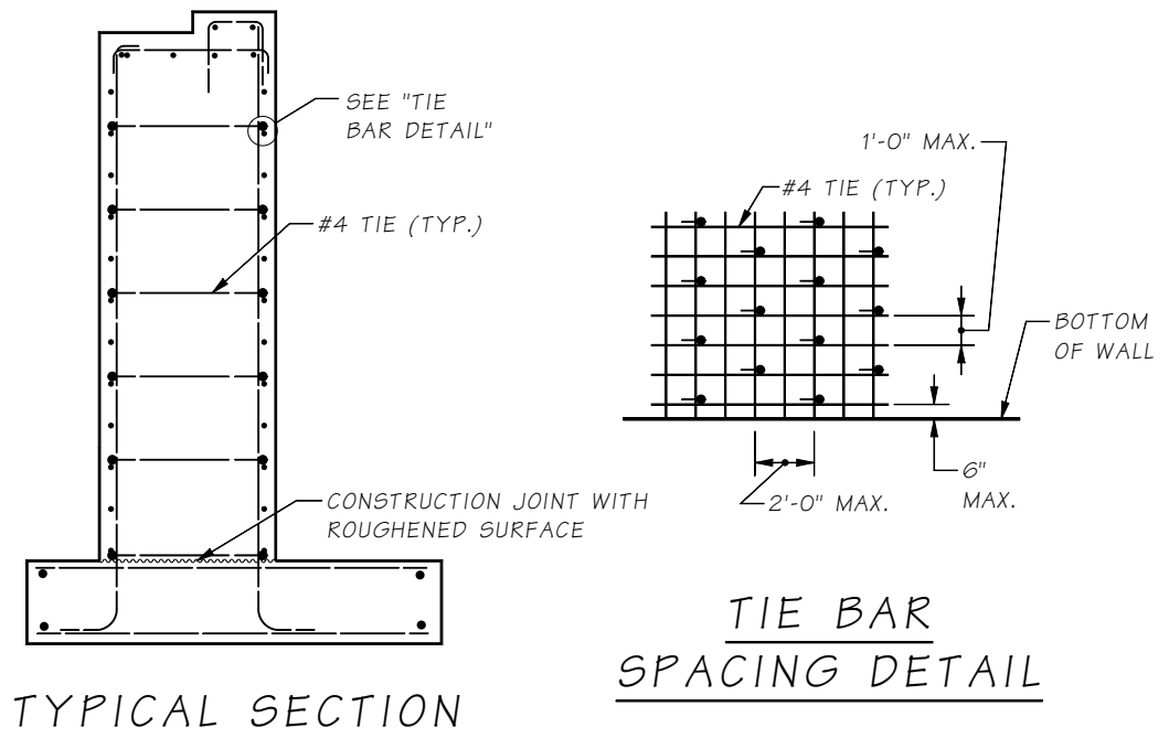
Figure 7.5.10-1 Cross Tie Details
