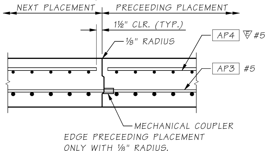
Figure 10.6.6-3 Alternate Longitudinal Joint Detail
