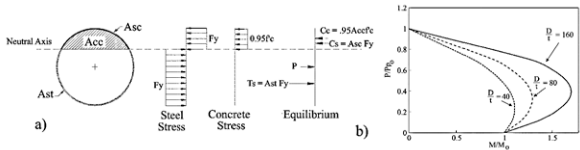
Figure 7.10.2-2 Plastic Stress Distribution for CFST
