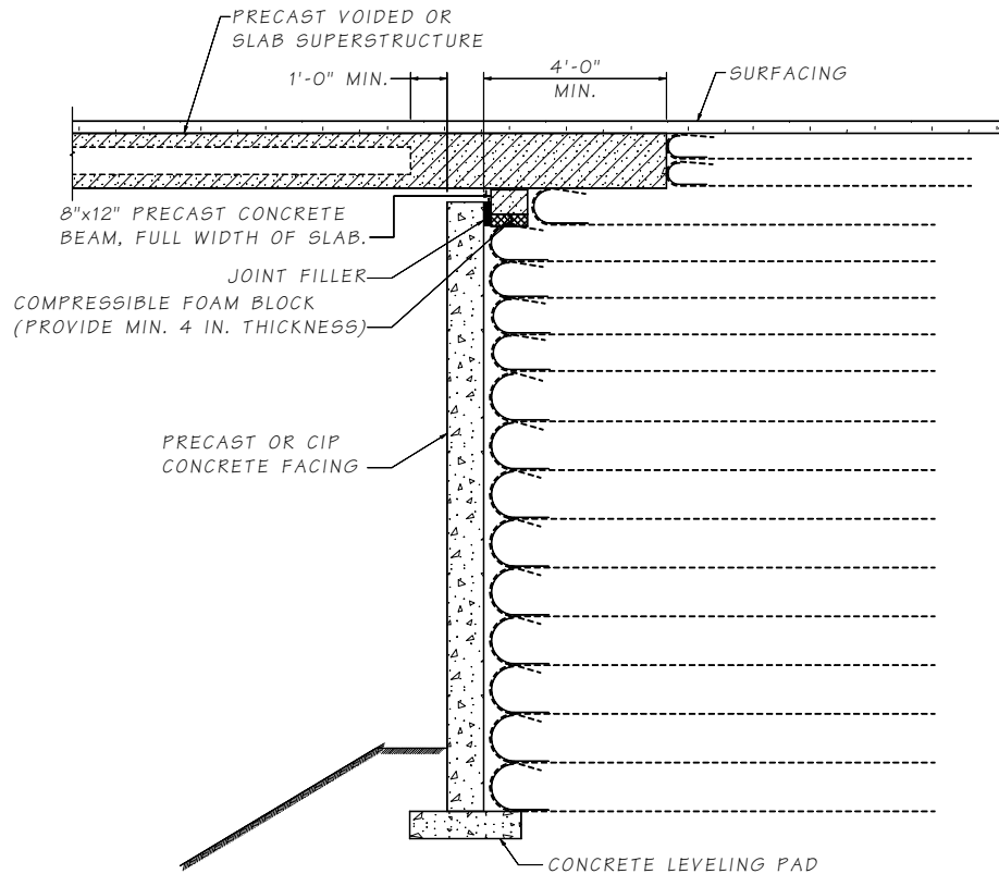
Figure 7.5.2-2 Reinforced Soil Abutment with Full-Height Concrete Facing
