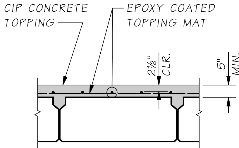
Figure 5.7.4-4 Type 4 Protection System
