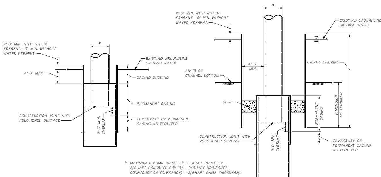
Figure 7.8.2-2 Shaft Casing Details
