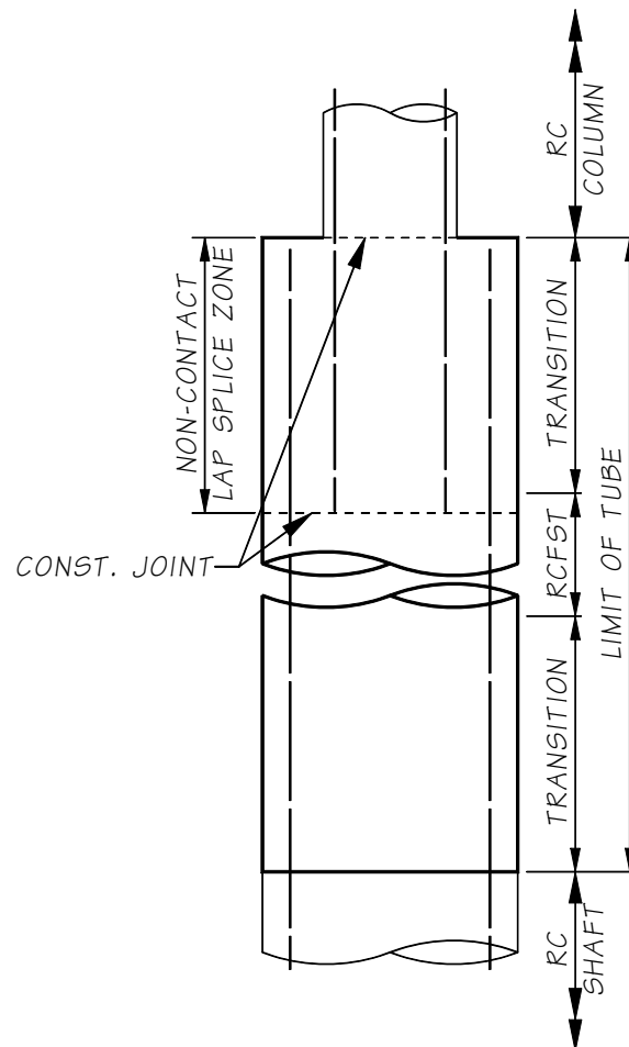
Figure 7.10.5-1 RCFST-to-Column Connection
