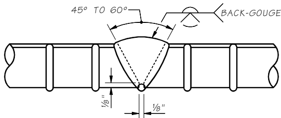
SINGLE V-GROOVE WELD AWS D1.4 FIGURE 3.2(A)
