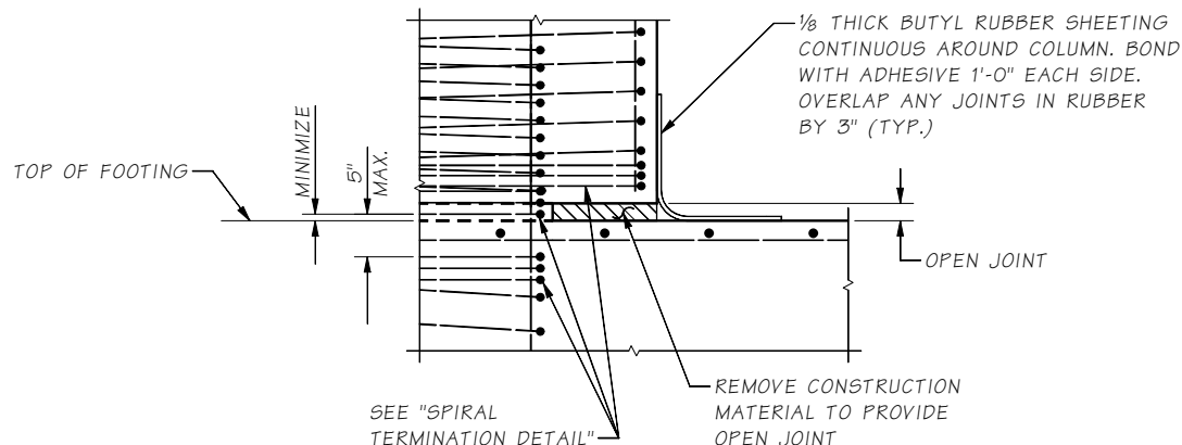
Figure 7.3.7-2 Open Gap Detail
