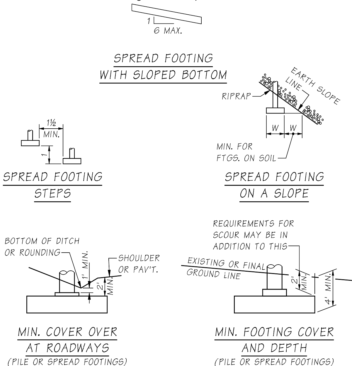
Figure 7.7.1-1 Guidelines for Footing Cover and Depth
