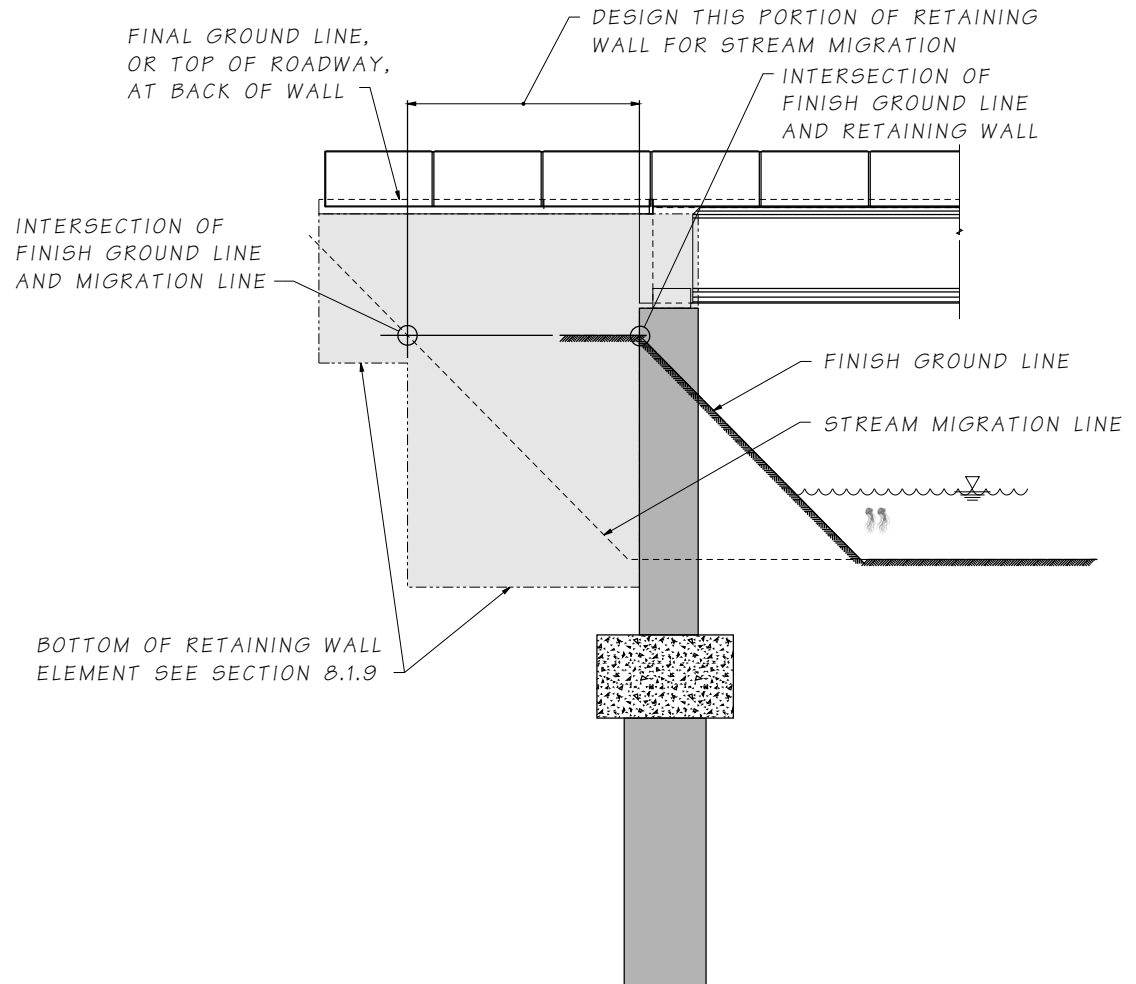
Figure 8.1.9-2 Stream Migration without Scour
