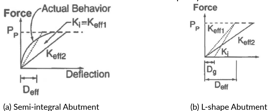
Figure 4.2.11-2 Characterization of Abutment Capacity and Stiffness
