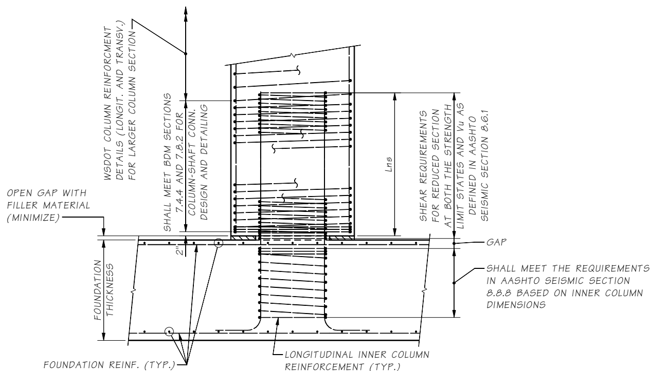
Figure 7.3.7-1 Reduced Column Section at Bottom of Column
