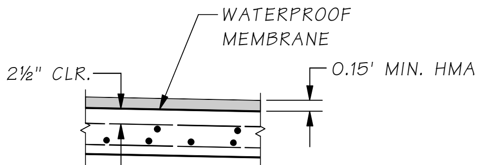
Figure 5.7.4-3 Type 3 Protection System
