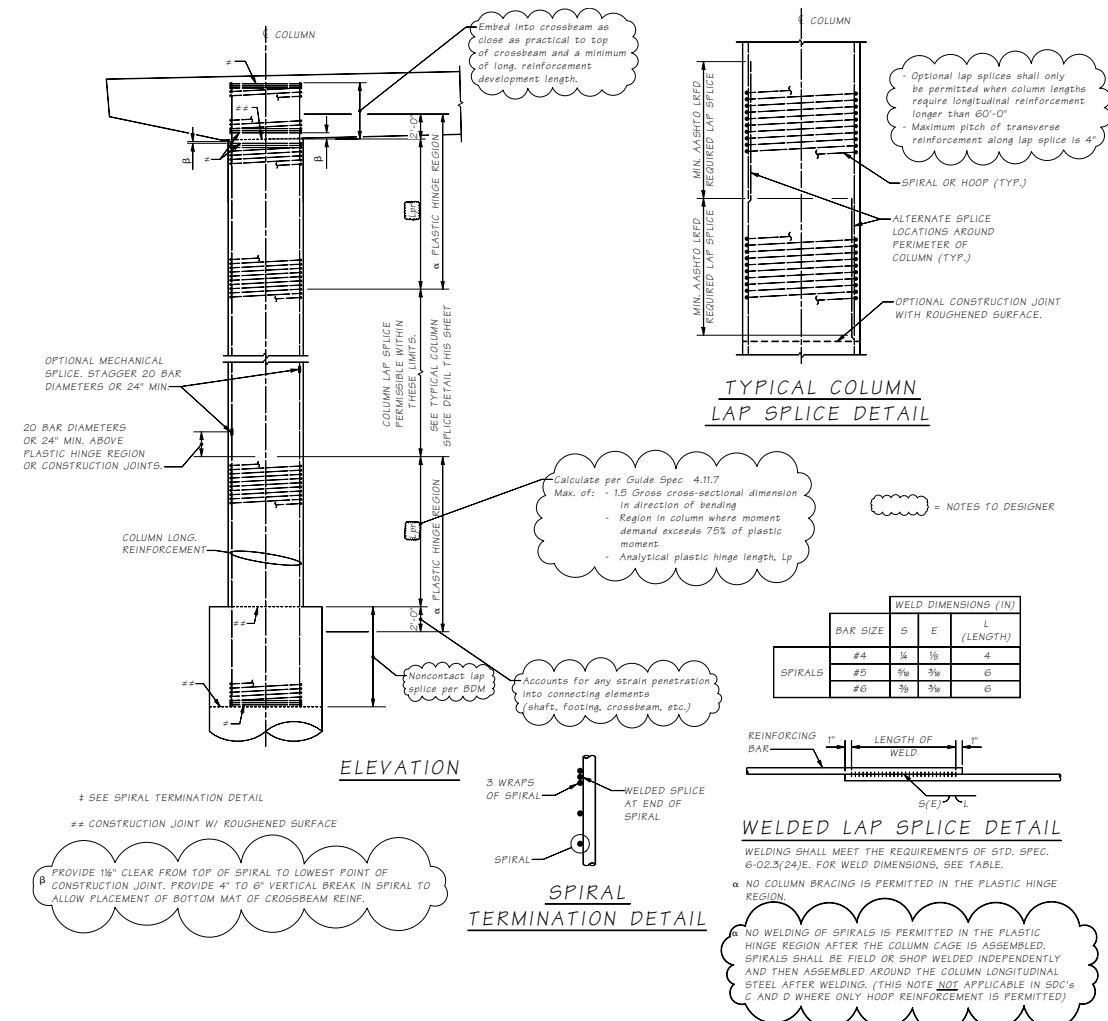
Figure 7.3.5-1 Column Splice and Plastic Hinge Region Details
