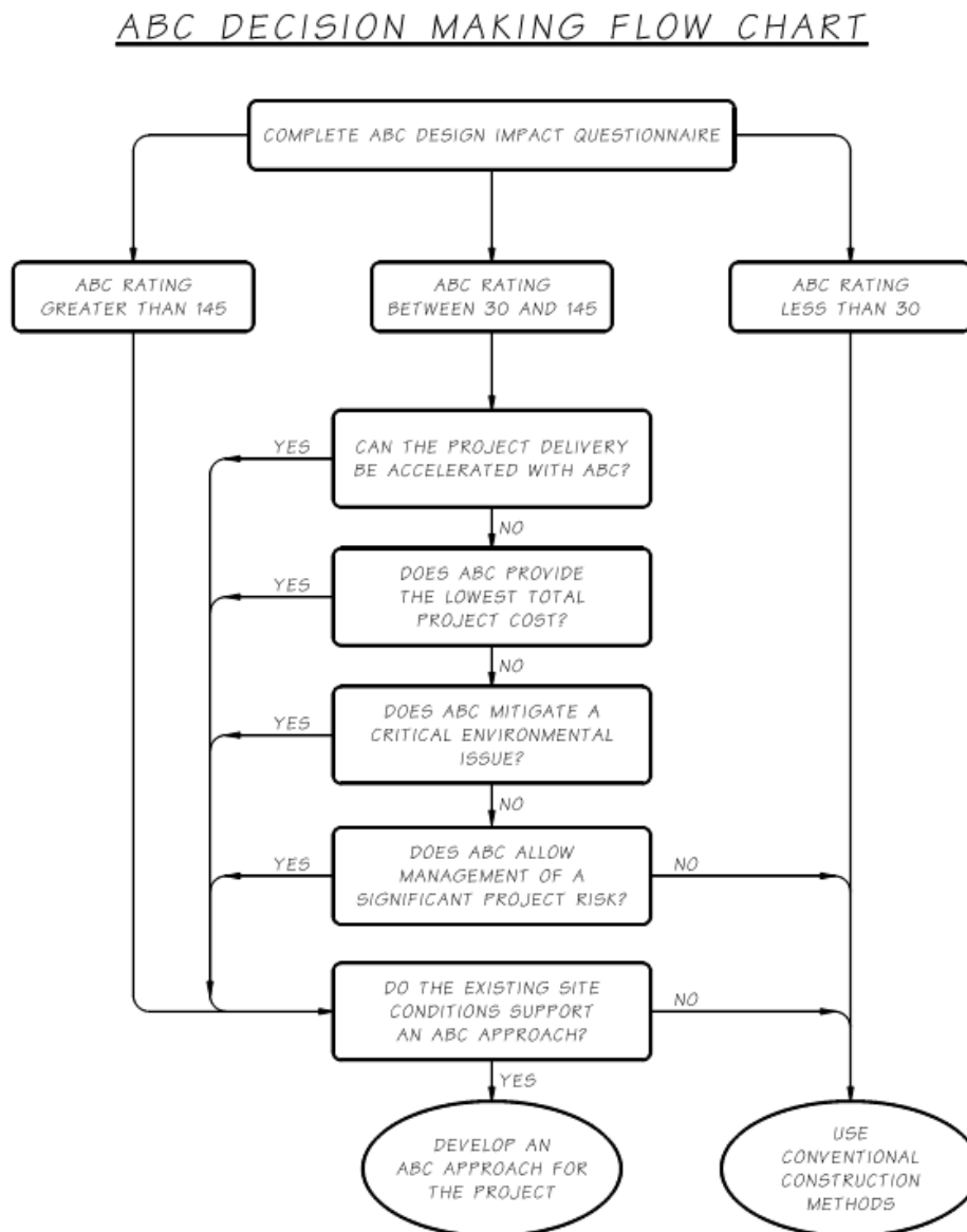
Figure 14.2.6-2 ABC Flow Chart
