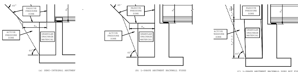
Figure 4.2.11-1 Abutment Stiffness and Passive Pressure Estimate
