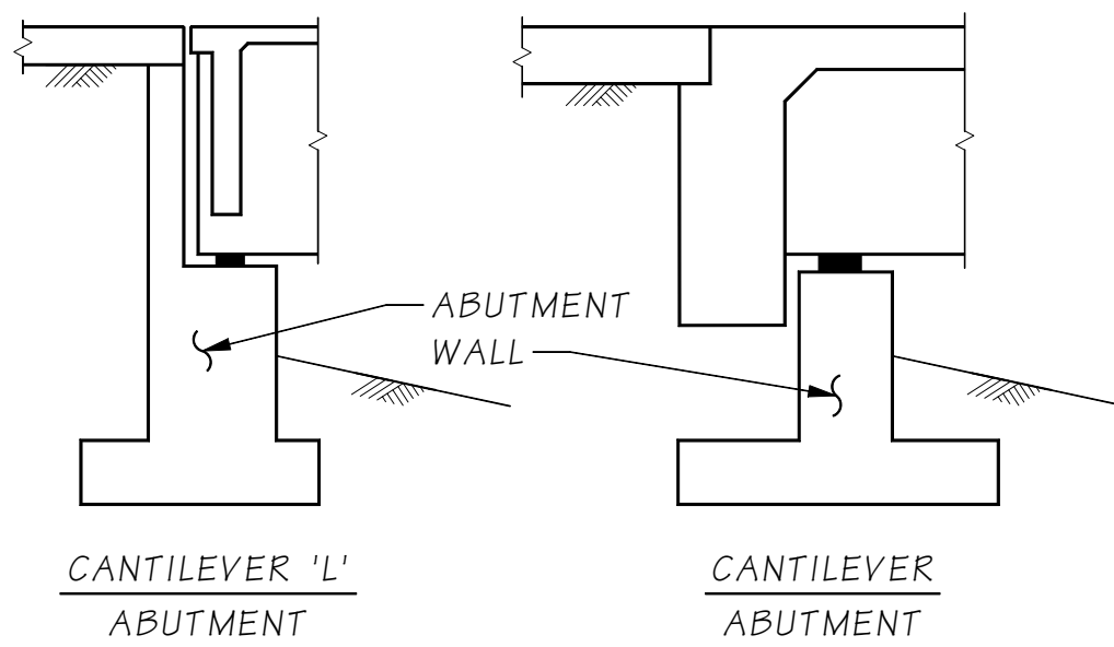
Figure 7.5.1-2 Cantilever Abutments
