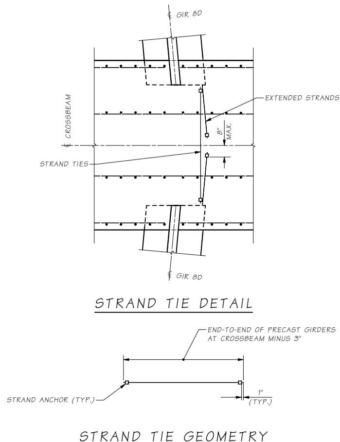
Figure 5.1.3-4 Strand Ties
