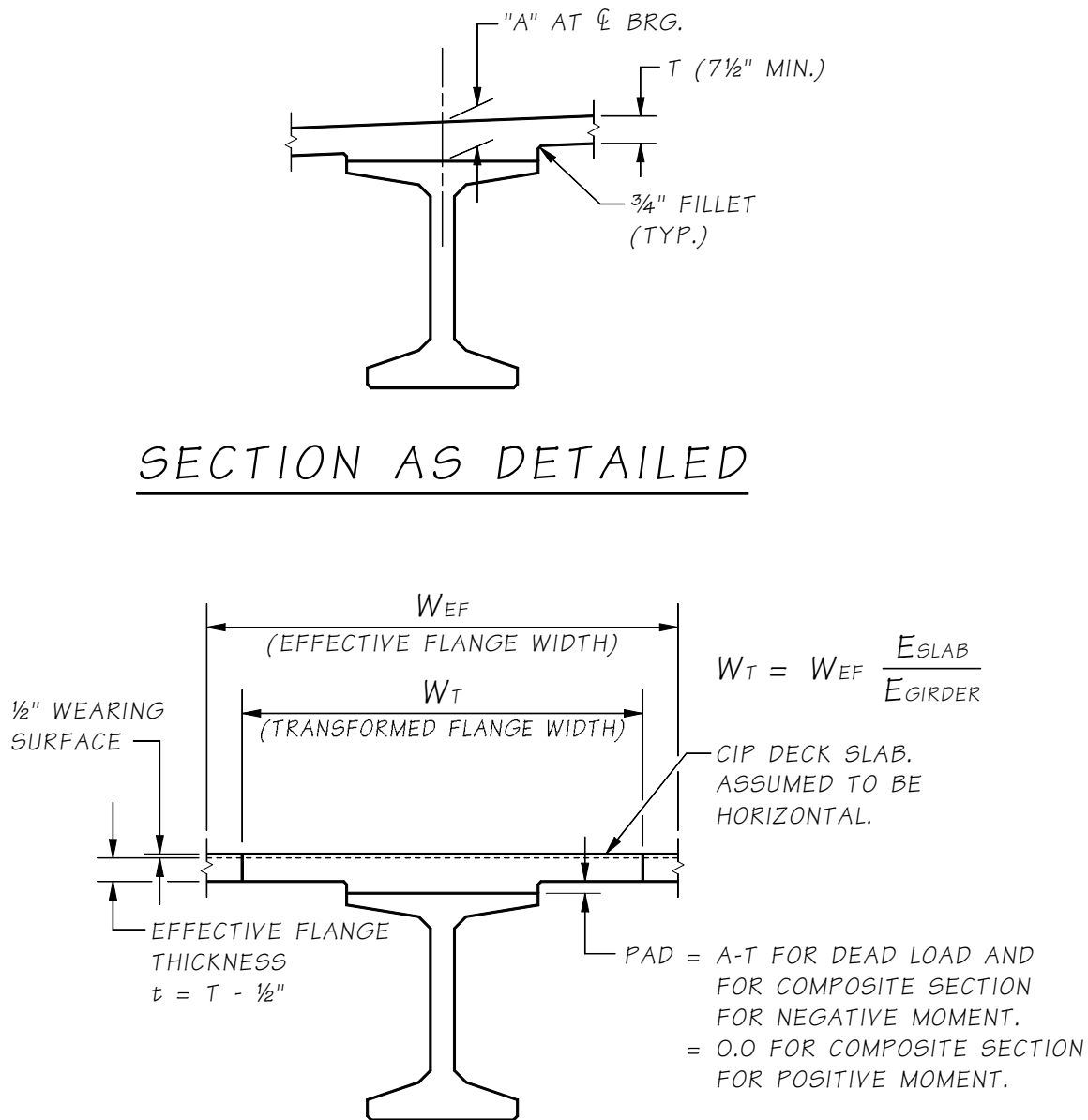
Figure 5.6.2-1 Typical Section for Computation of Composite Section Properties
