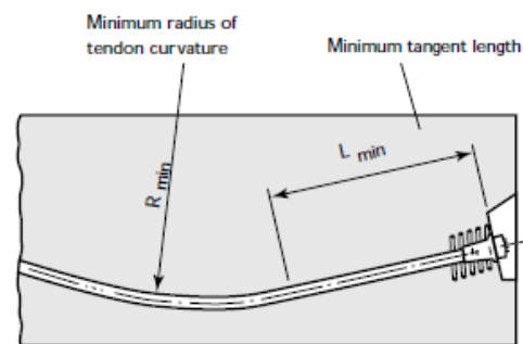
Figure 5.8.1-5 Tangent Length and Tendon Radii
