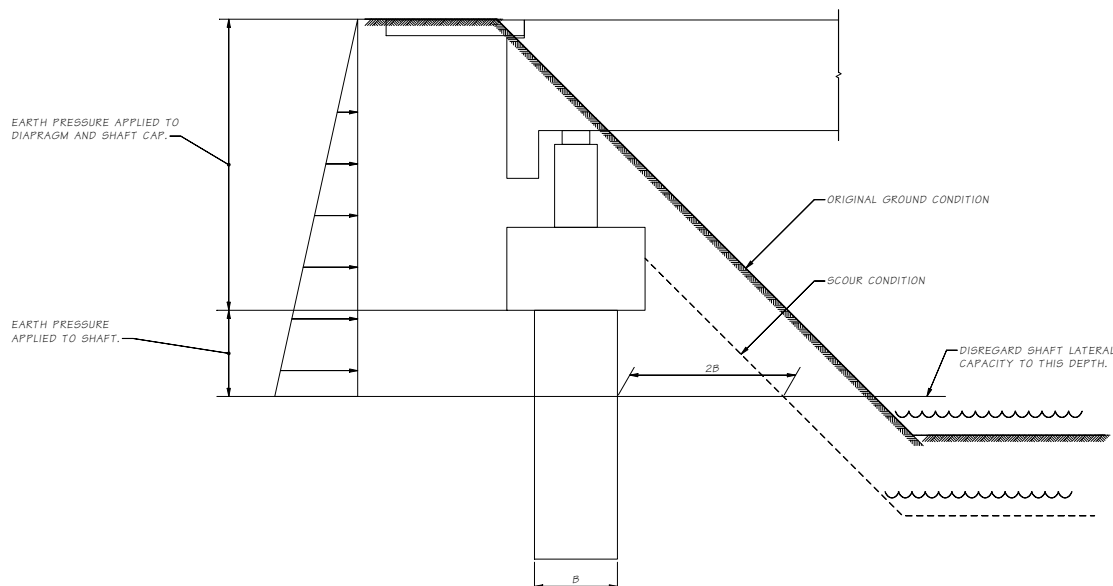
Figure 7.1.7-1 Scour effects when all or a portion of a shaft cap is exposed
