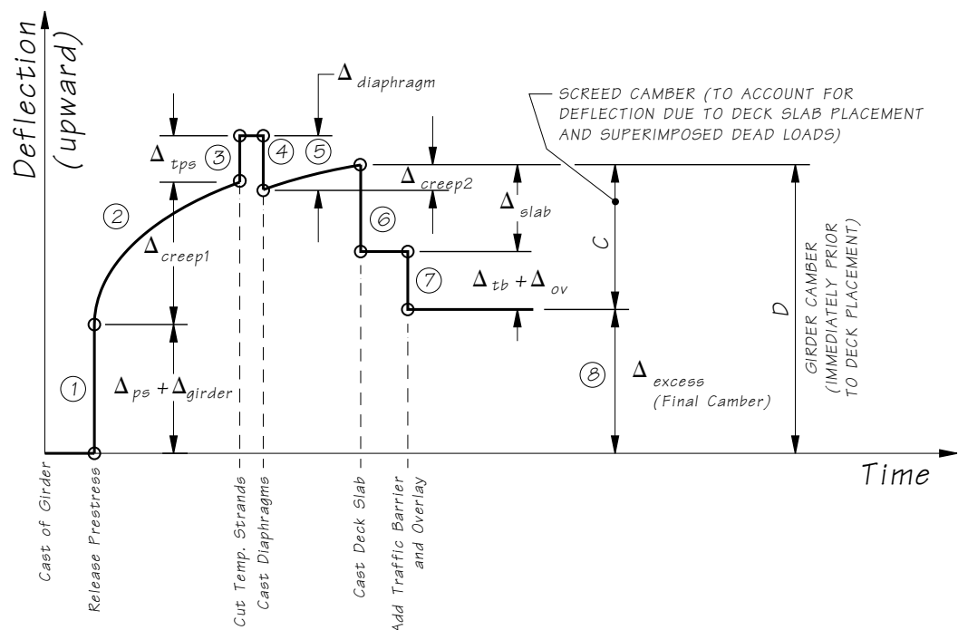
Figure 5.2.4-1 Prestressed Concrete Girder Camber
