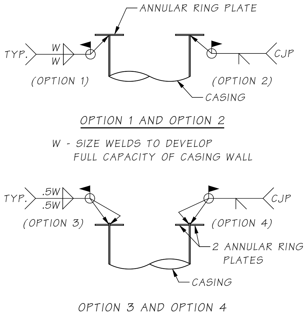
Figure 7.10.3-2 Annular Ring Weld Detail
