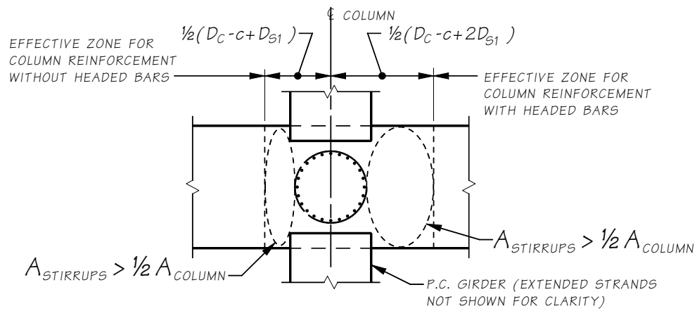
Figure 7.3.5-2 Longitudinal Development Into Crossbeams
