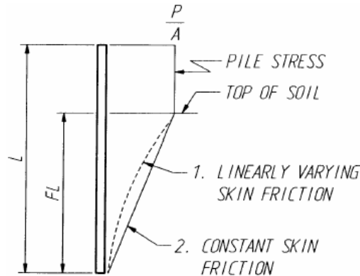
Figure 7-B1-4 Pile Stress
