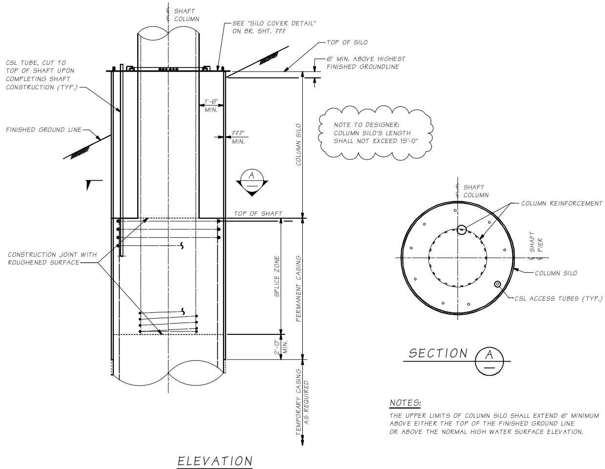
Figure 7.3.4-1 Column Silo on Shaft Foundation
