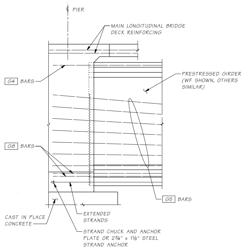
Figure 5.2.2-2 End Connection for Continuous Span Girder
