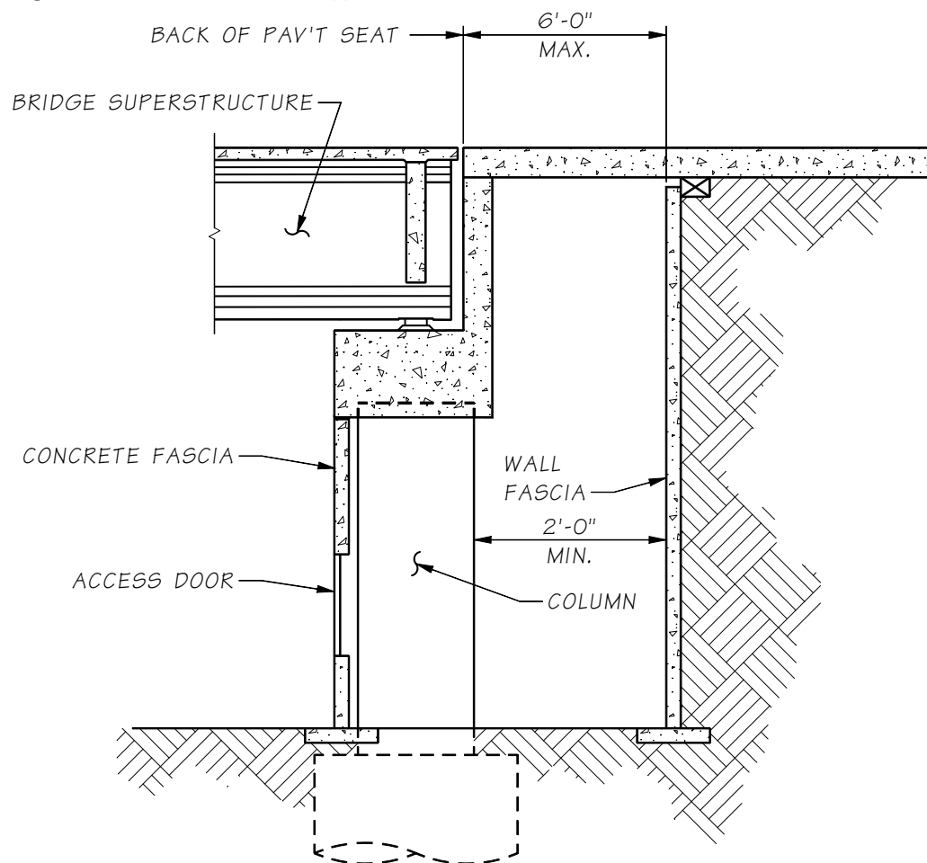
Figure 7.5.1-4 Bent-Type Abutment
