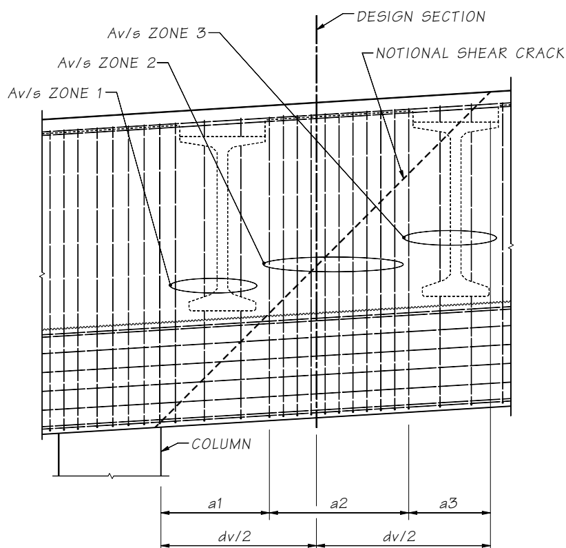
Figure 7.4.1-1 Effective Crossbeam Shear Reinforcement
