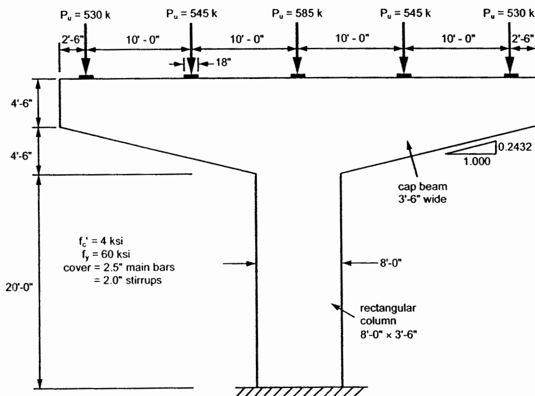
Figure 5.1. Details of hammerhead pier.
