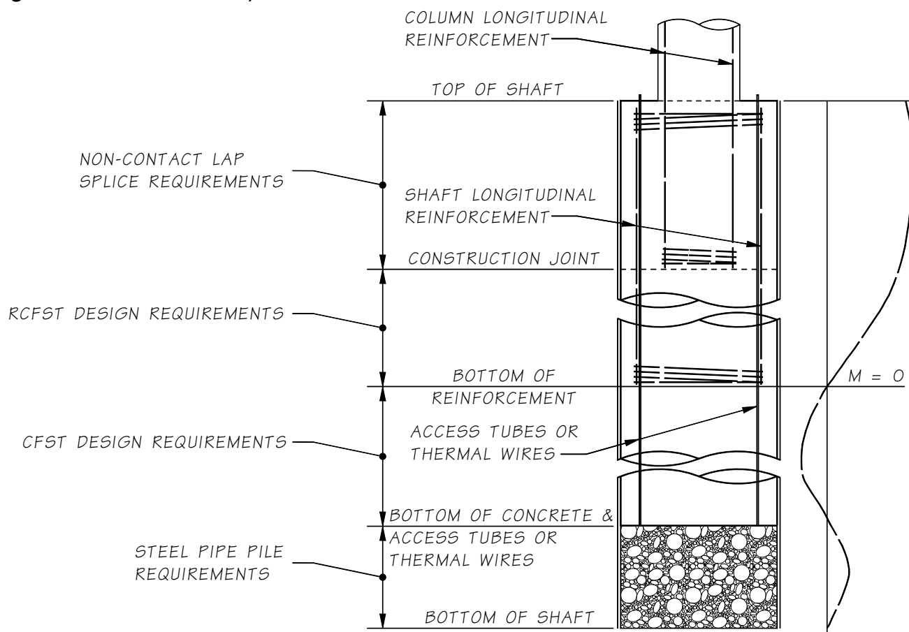
Figure 7.10.6-1 Partially-filled CFST
