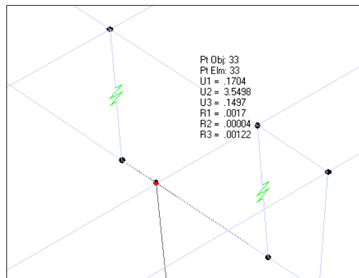
Joint Displacement at Joint 33 for Load Case "EY"
