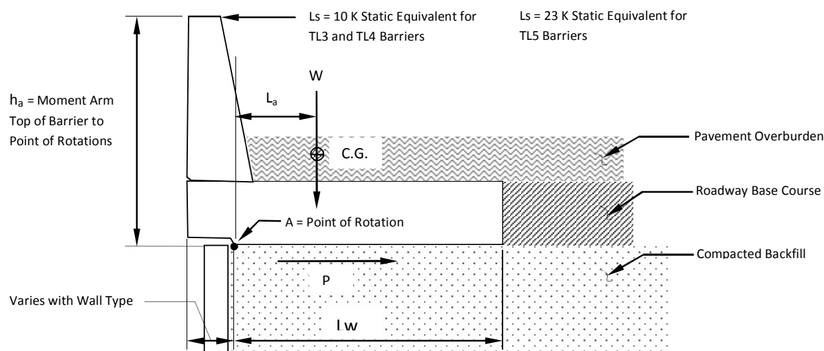
Figure 10.3.2-1 Global Stability of Barrier–Moment Slab System
