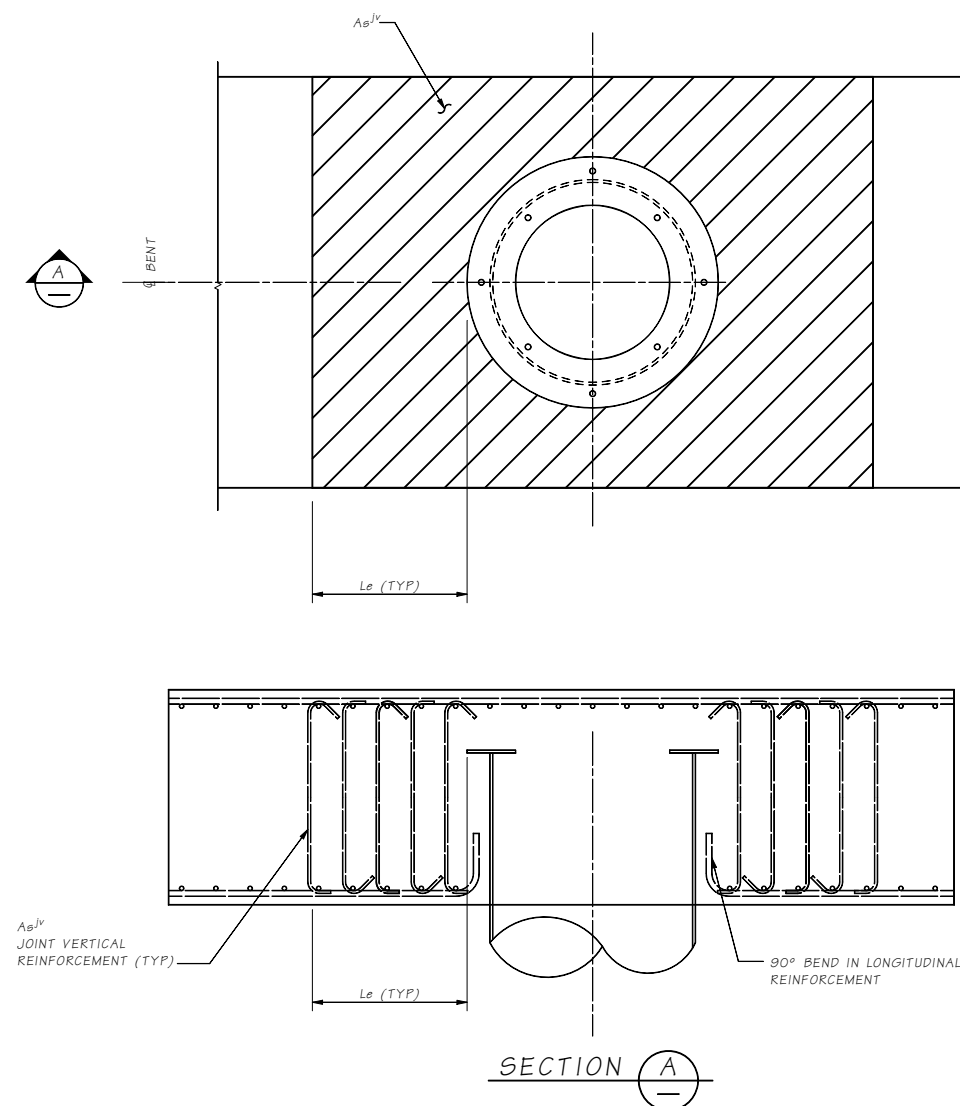
Figure 7.10.3-3 Reinforcement Detail at Cap Connection
