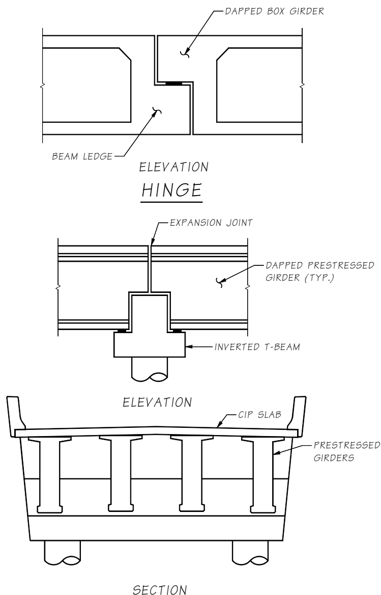
Figure 5.4-1 Hinge and Inverted T-Beam Pier Cap
