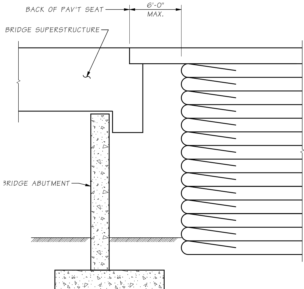
Figure 7.5.1-5 Isolated Abutment
