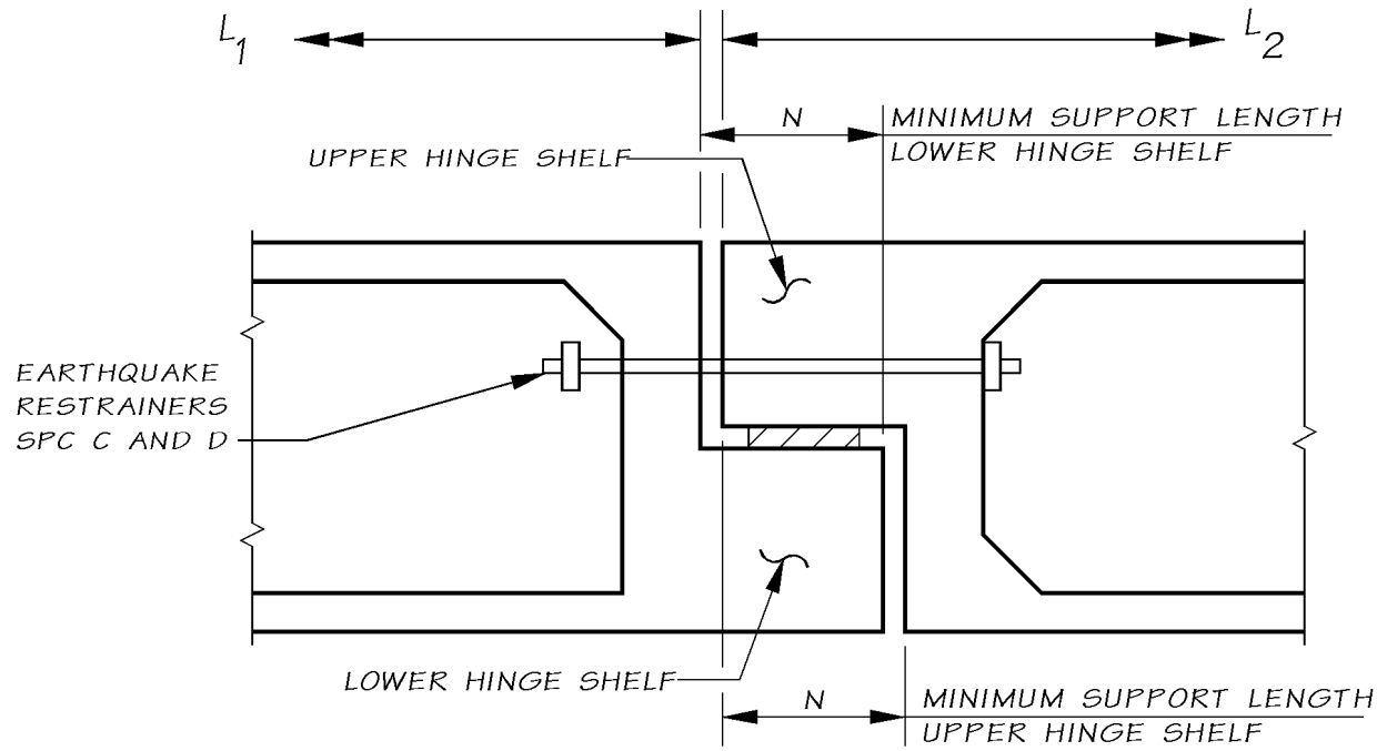
Figure 5.4-2 In-Span Hinge
