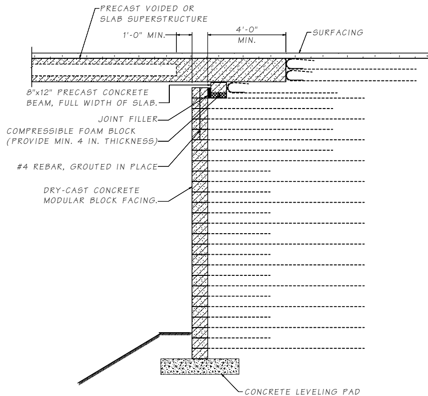
Figure 7.5.2-1 Reinforced Soil Abutment with Dry-Cast Modular Block Facing
