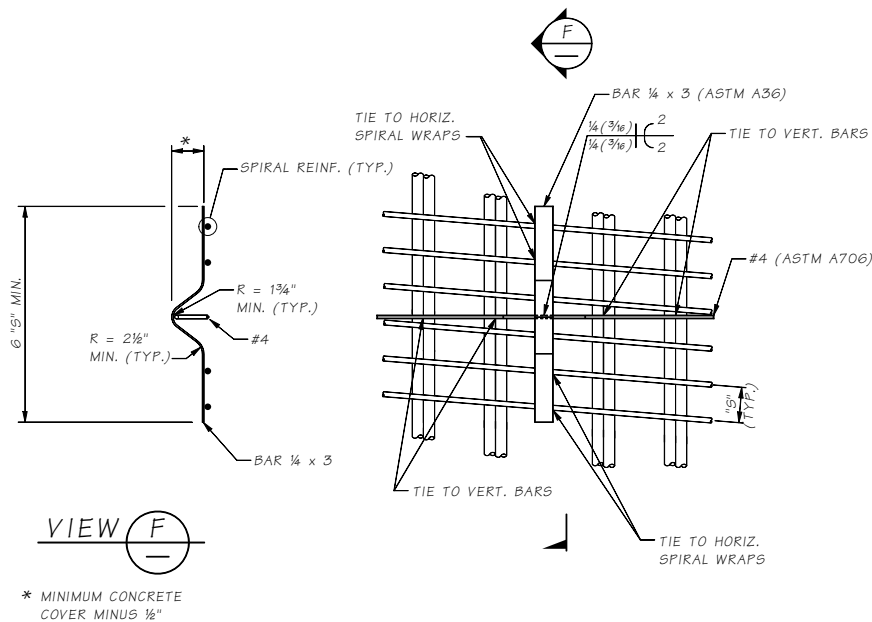
Figure 7.8.2-4 Centralizer Detail
