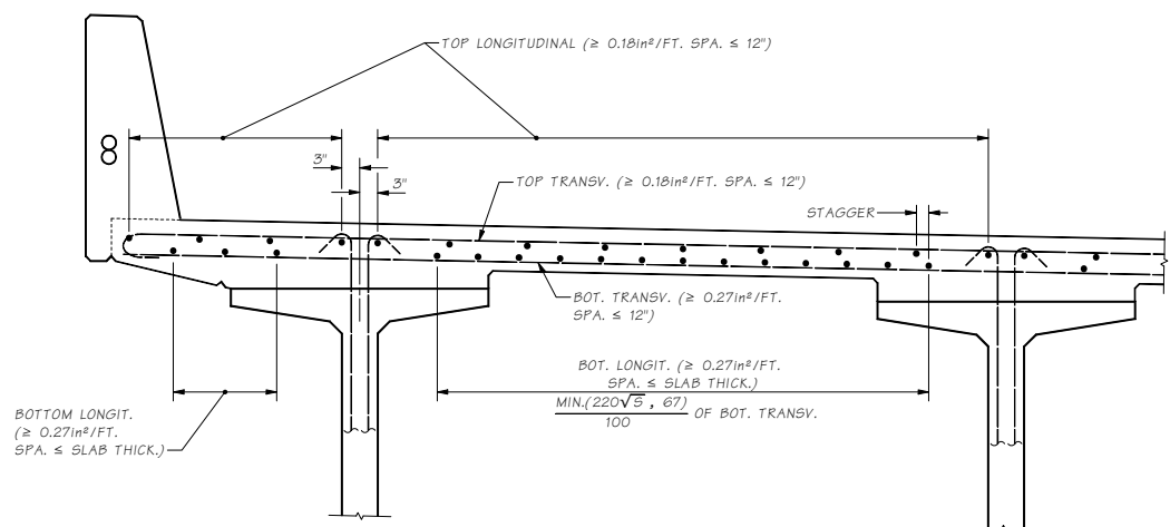
Figure 5.7.2-2 Nominal Longitudinal Bridge Deck Reinforcement
