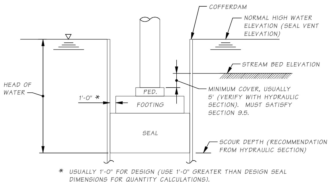
Figure 7.1.6-1 Foundation Seal
