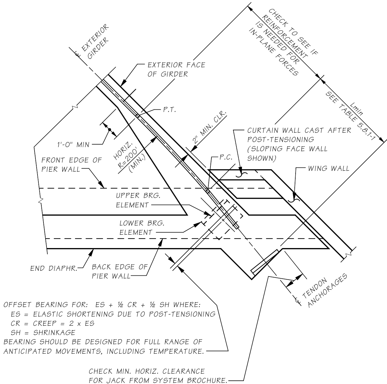
Figure 5.8.1-4 Layout of Anchorages and End Blocks
