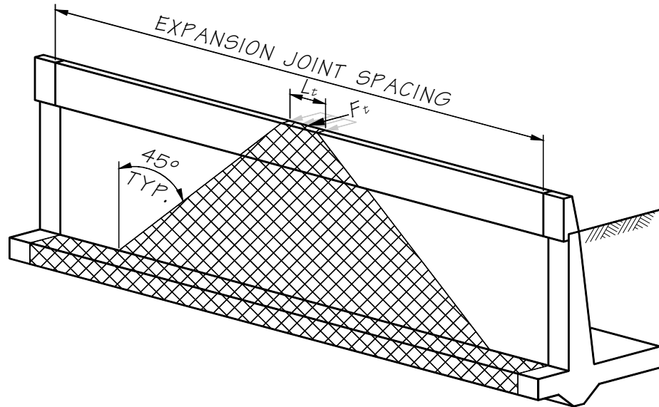
Figure 8.1.4-3 Application and Distribution of Vehicular Collision Load occurring near the midsection.
