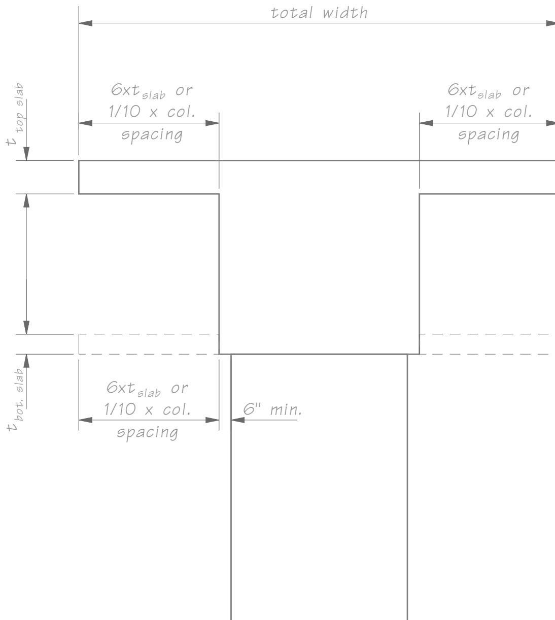
Figure 5.3.3-3 Effective Width of Crossbeam
