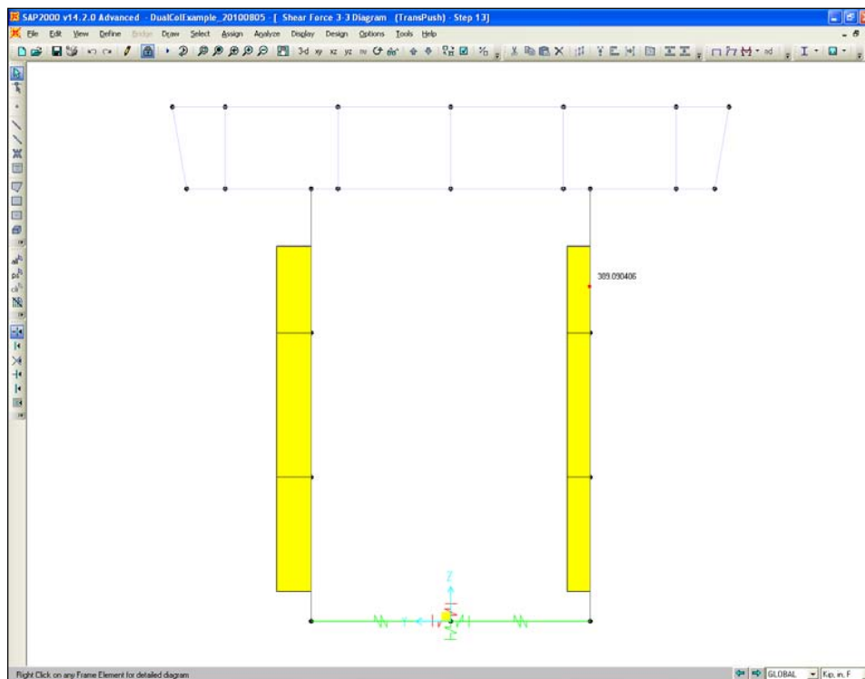
Frame Shear 3-3 Diagram for Load Case “TransPush” at Step 13
