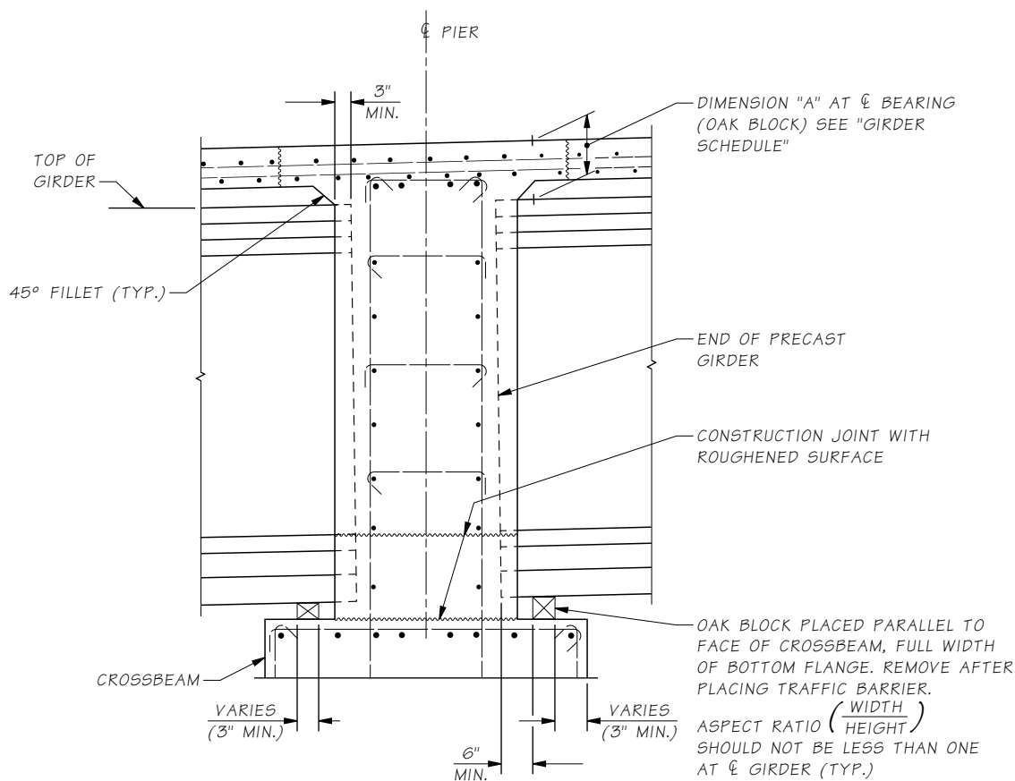
Figure 5.6.2-6 End Type D
