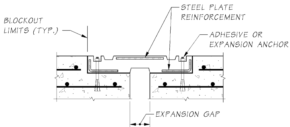
Figure 9.1.4-3 Bolt-down Panel Joint
