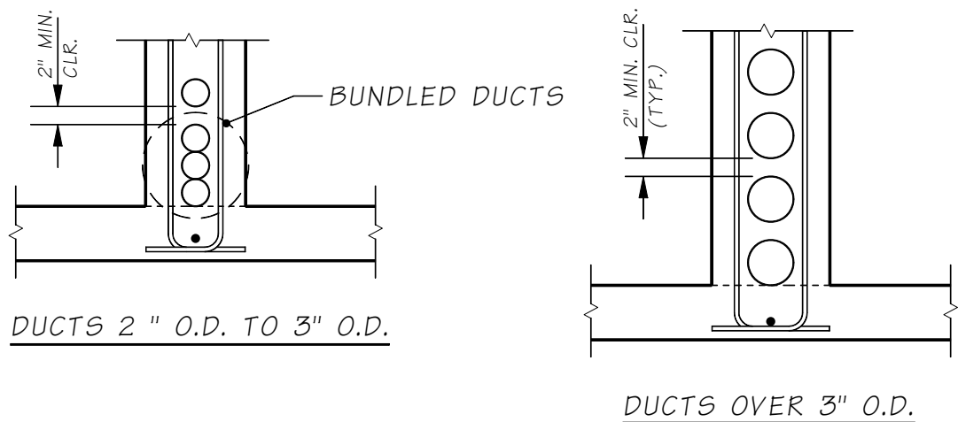
Figure 5.8.1-2 Tendon Placement Pattern for Box Girder Bridges
