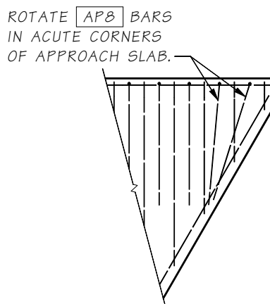
Figure 10.6.4-2 Flared Corner Steel
