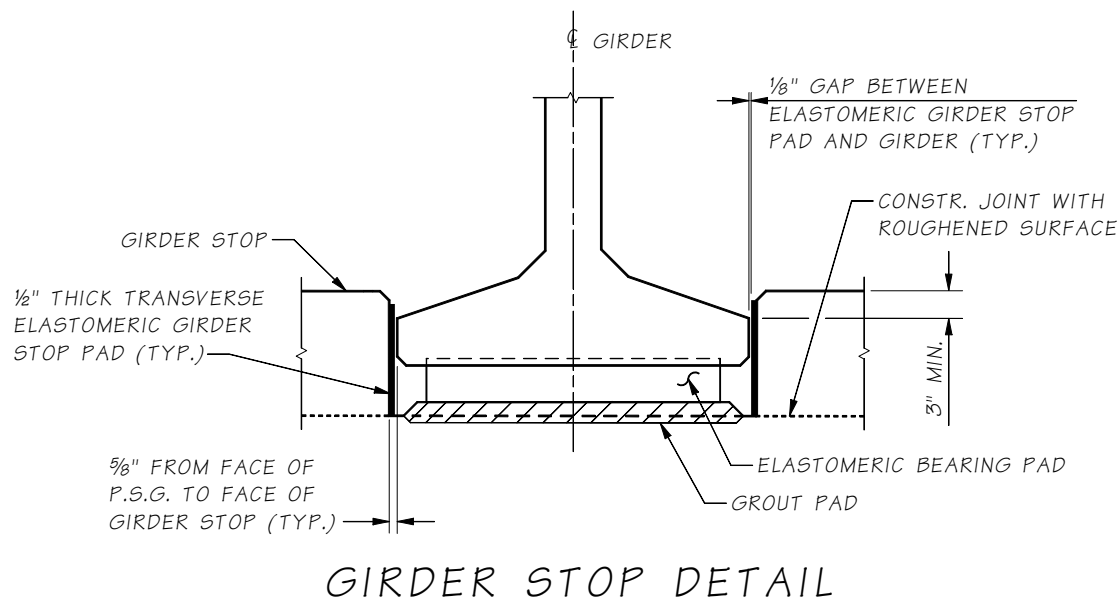
Figure 7.5.6-1 Girder Stop Details
