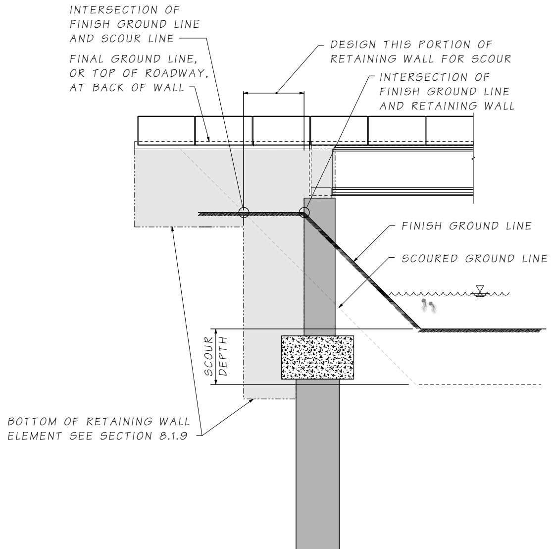
Figure 8.1.9-1 Scour without Stream Migration
