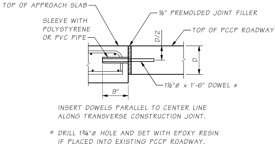
Figure 10.6.6-2 PCCP Roadway Dowel Bar Detail
