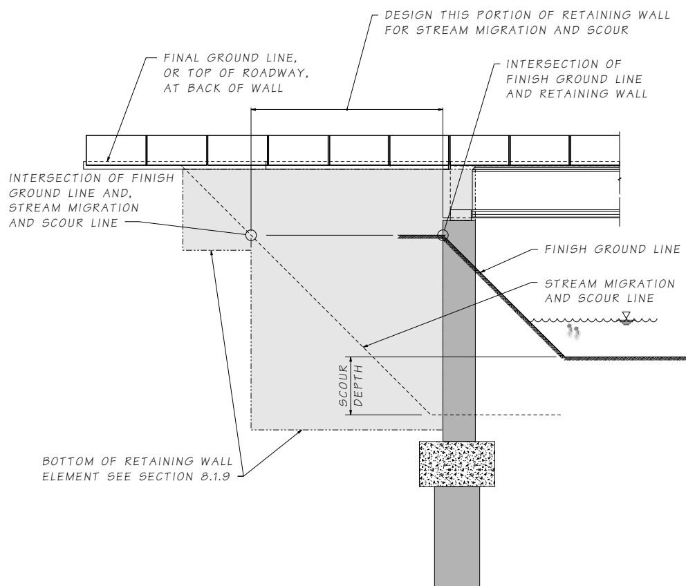
Figure 8.1.9-3 Stream migration WITH Scour
