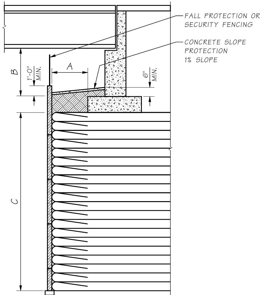
Figure 7.5.2-3 Spread Footing on SE Wall or Geosynthetic Wall
