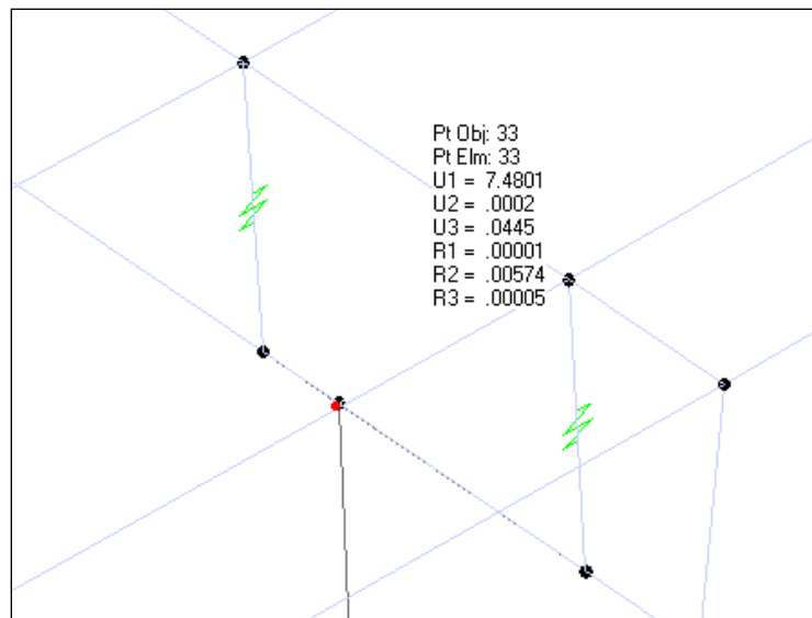
Joint Displacement at Joint 33 for Load Case "EX"
