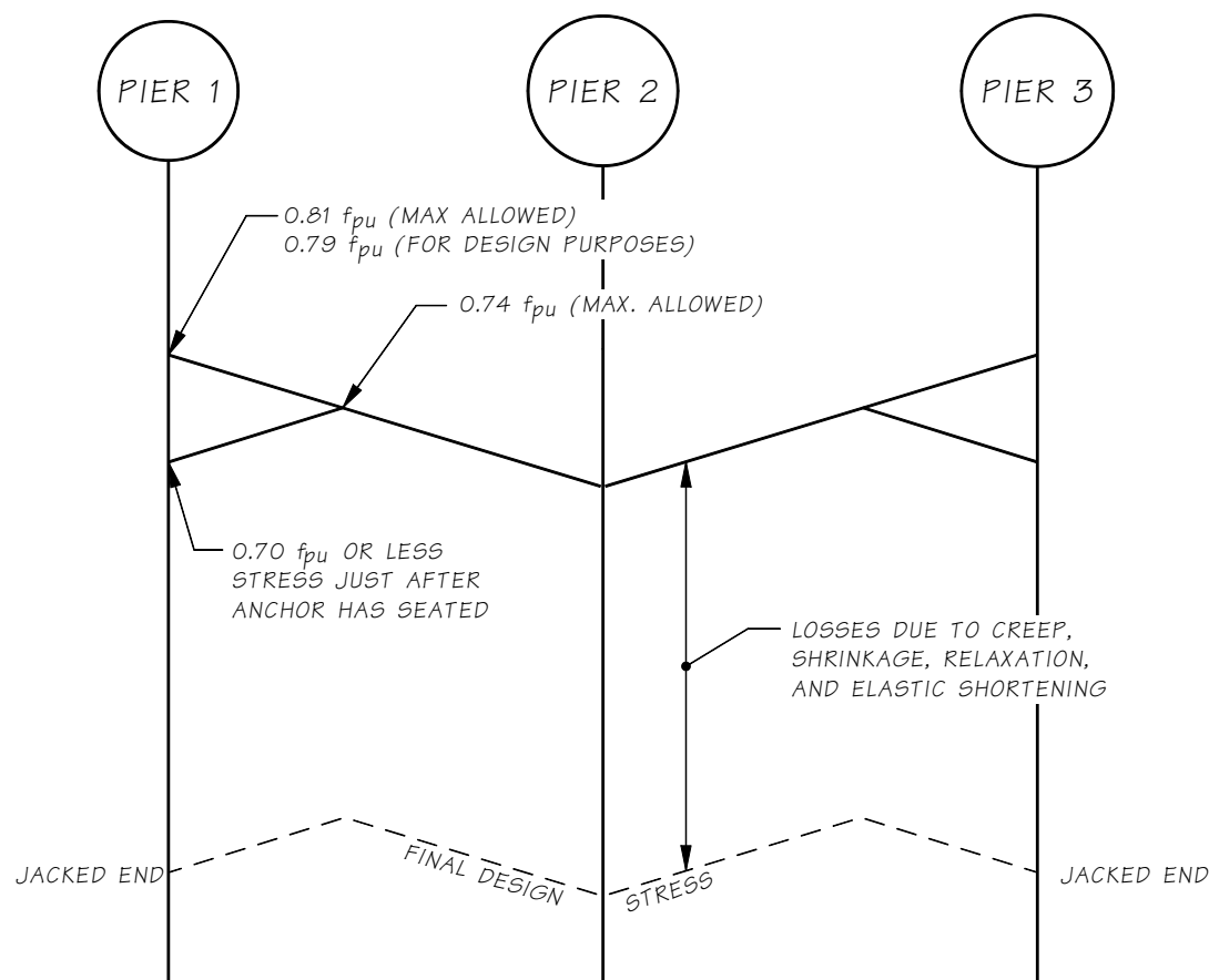
Figure 5.8.3-1 Stress Diagram for a 2-Span PT Bridge
