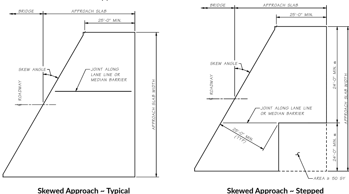
Figure 10.6.4-1 Skewed Approach
