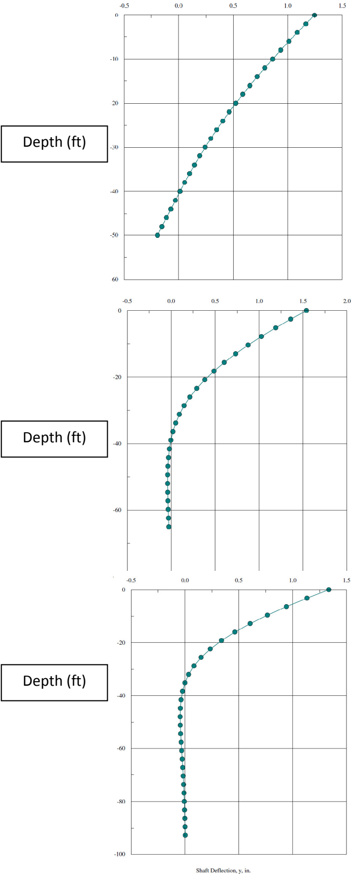
Figure 7.2.6-2 Various Shaft Deflected Shapes
