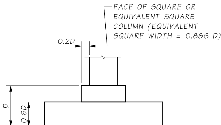
Figure 7.7.1-2 Pedestal Dimensions
