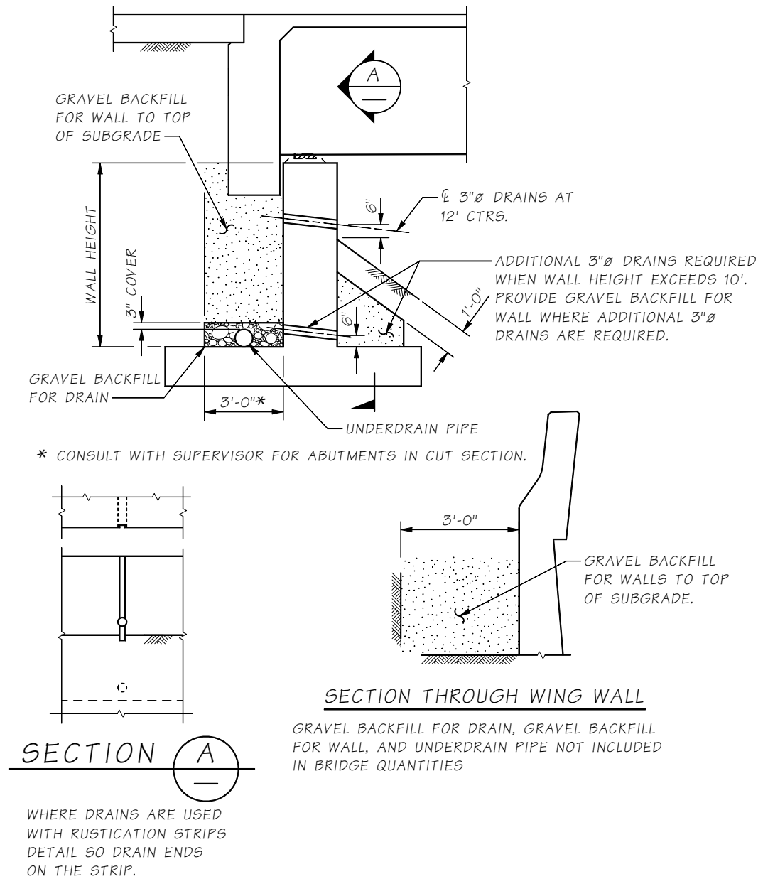
Figure 7.5.11-1 Drainage and Backfill Details
