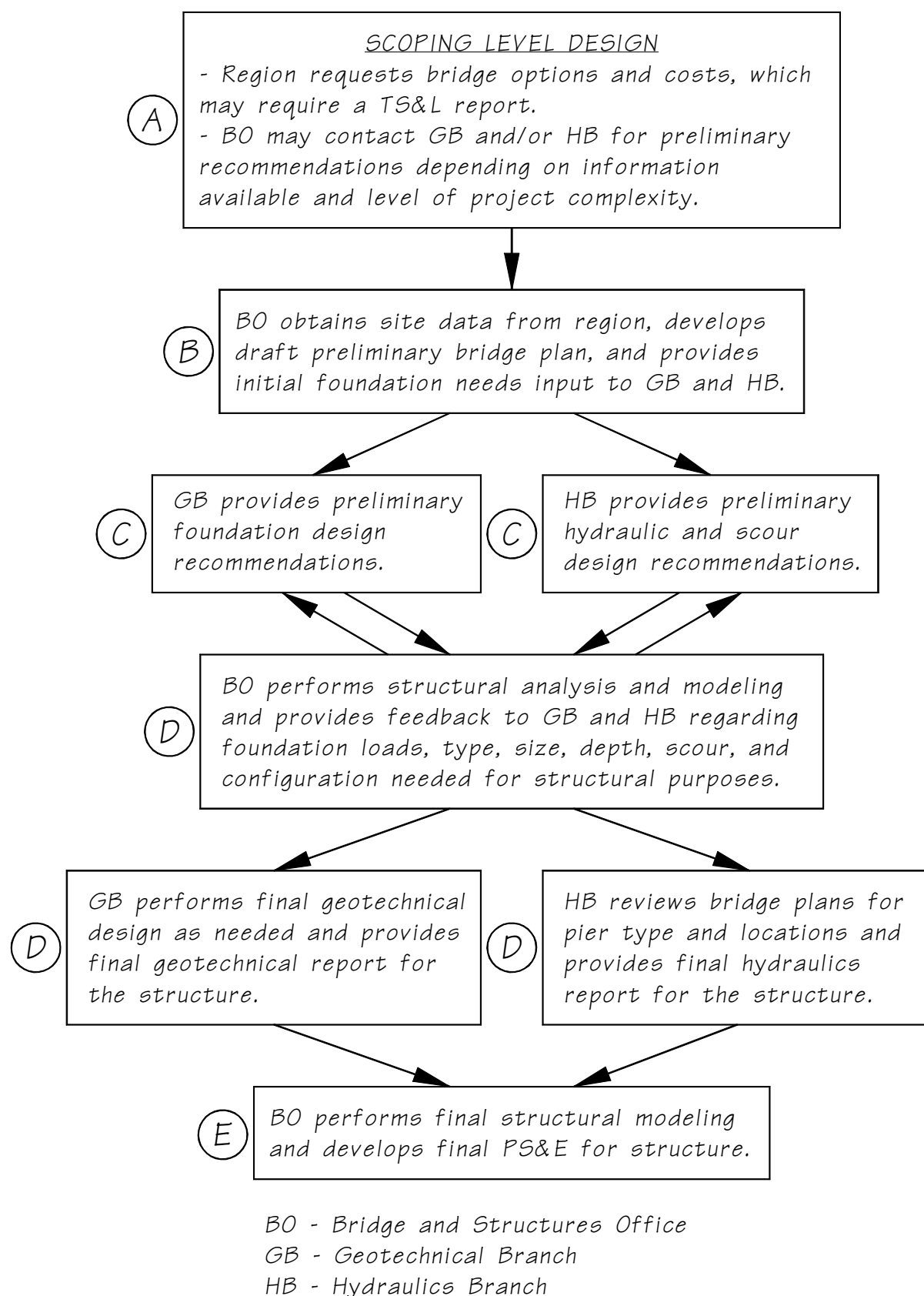
Overall Design Process for LRFD Foundation Design
