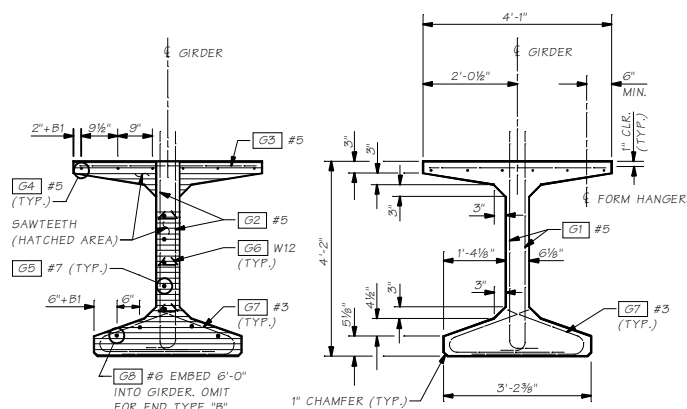
VIEW B STRANDS NOT SHOWN
