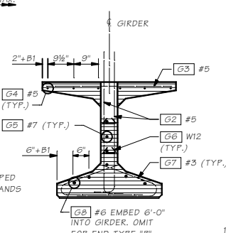
VIEW (B)
