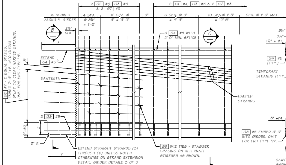
TYPICAL END ELEVATION
