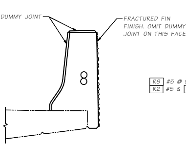
SECTION C
