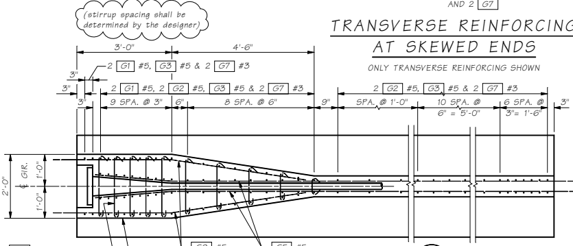
SECTION A
