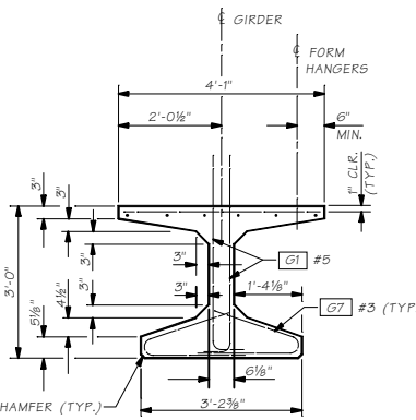
SECTION (C)
