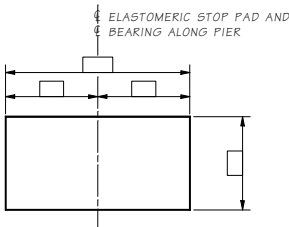
ELASTOMERIC STOP PAD
