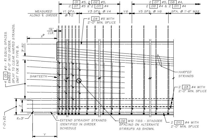
TYPICAL END ELEVATION
