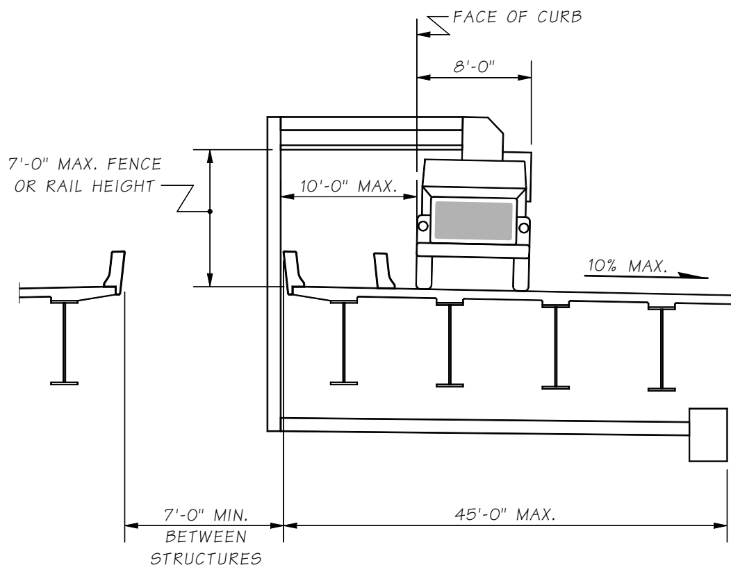
Limits of Under Bridge Inspection Truck
