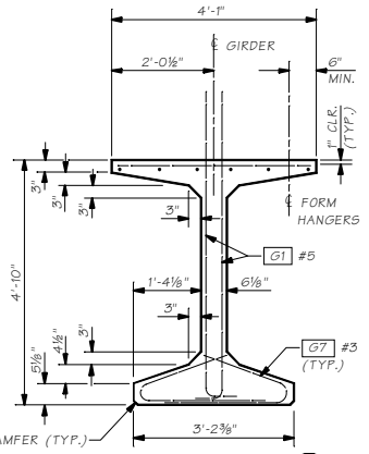
SECTION C STRANDS NOT SHOWN
