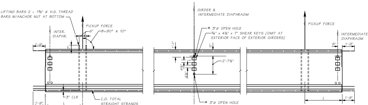
GIRDER ELEVATION ~ MID-SEGMENT
