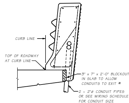
SECTION B BRIDGE
