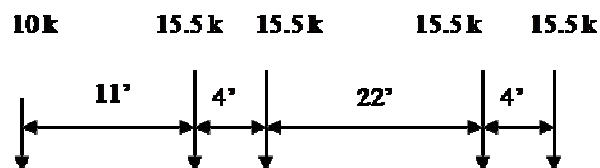
Figure 13.1-3
