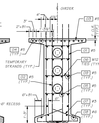
SECTION C
