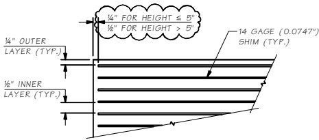
SECTION B
