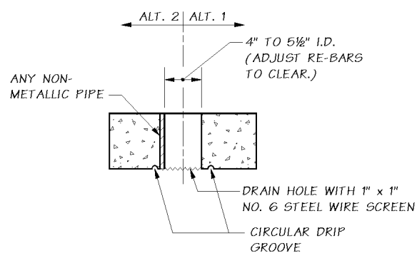
BOTTOM SLAB DRAIN HOLE DETAIL
