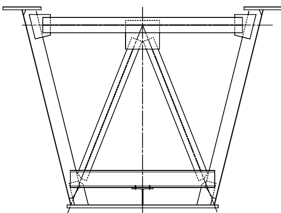
EXAMPLE CROSSFRAME REGIONS WITH FLANGE STIFFENER
