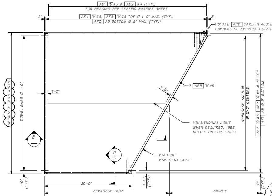
PLAN
