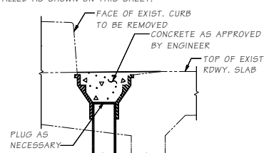
BRIDGE DRAIN PLUG DETAIL
