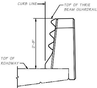
END VIEW THRIE BEAM SHOWN WITH "D" CONNECTION
