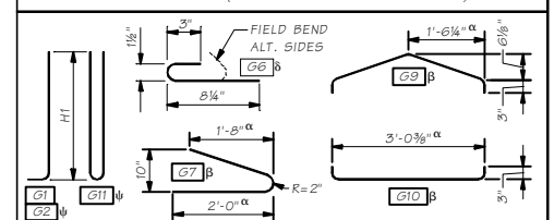
BENDING DIAGRAM (ALL DIMENSIONS ARE OUT TO OUT)
