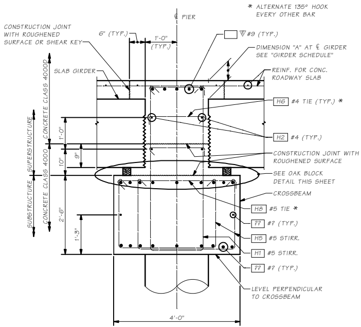
SECTION A
