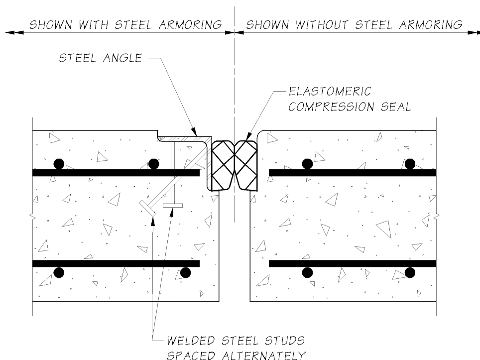
Compression Seal Joint Figure 9.1.3-1
