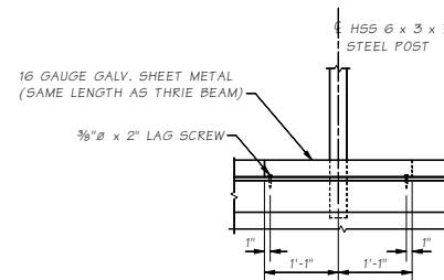
WATER BARRIER SPLICE DETAIL
