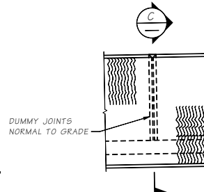
VIEW A
