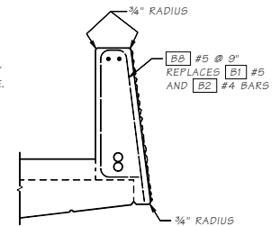
SLIPFORM ALTERNATE
