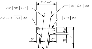
TOP FLANGE DETAIL SYMMETRICAL ABOUT C GIRDER
