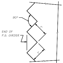
SAWTOOTH DETAILS
