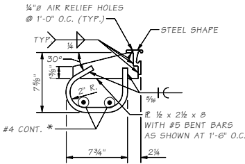
STRIP SEAL
