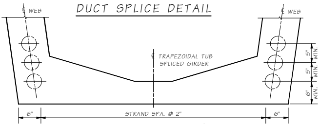
STRAND PATTERN AT C. SPAN
