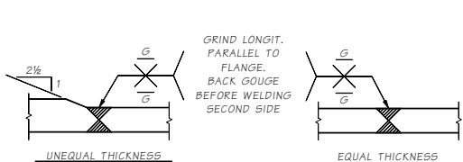
TENSION OR COMPRESSION FLANGE SPLICE
