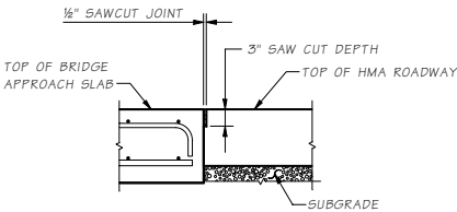
HMA ROADWAY JOINT DETAIL
