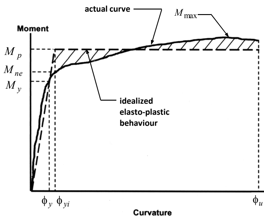
Figure 8.5-1 Moment-Curvature Model
