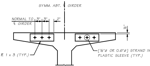
END VIEW TEMPORARY STRAND POST-TENSIONED ALTERNATE
