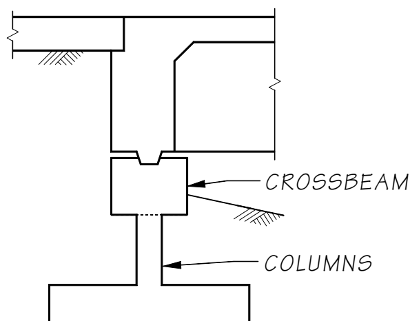
Spill-Through Abutment
