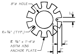
ANCHOR PLATE DETAIL
