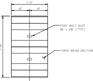
BACKUP PLATE
