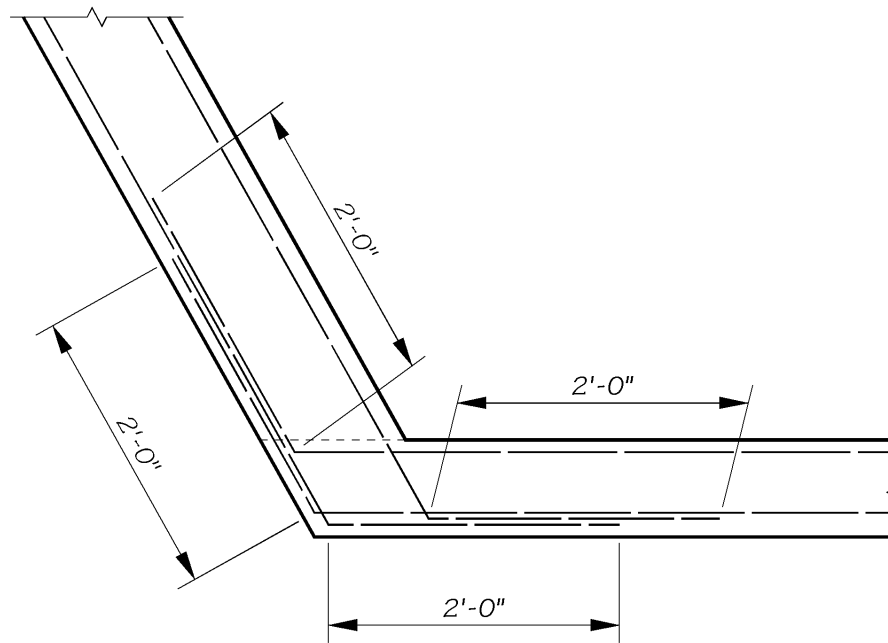
SLOPED WEB
