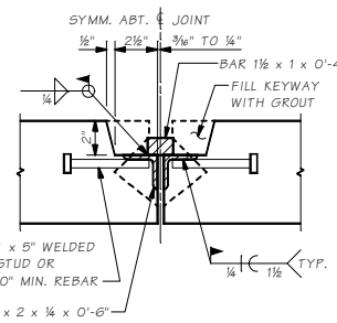
ALTERNATE 2
