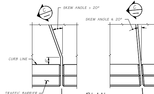
PLAN EXPANSION JOINT
