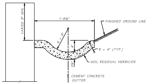
DETAIL E
