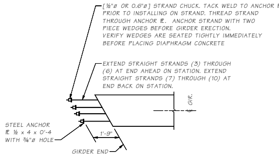
ALTERNATE #1
