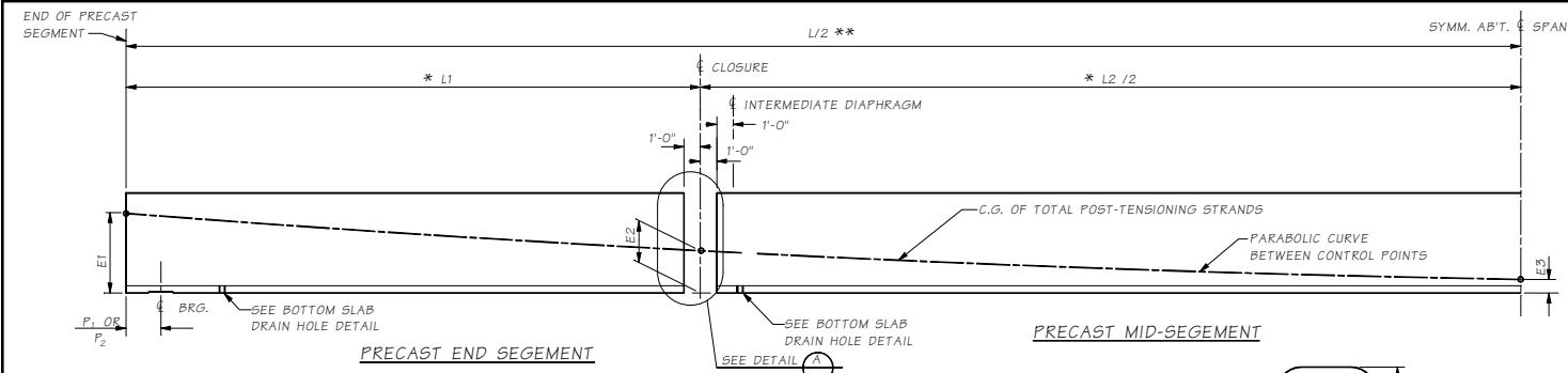
PRECAST LONGITUDINAL HALF-SECTION
