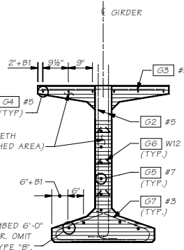
VIEW B STRANDS NOT SHOWN
