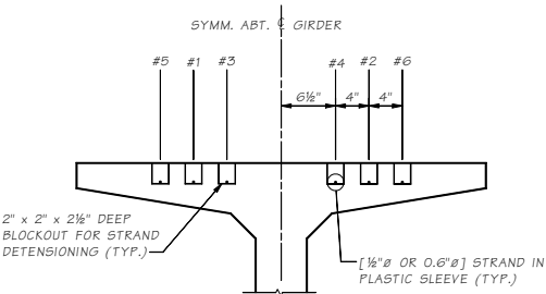
SECTION A
