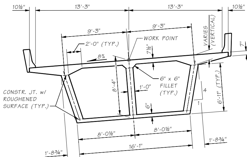
b - 8% SUPERELEVATION
