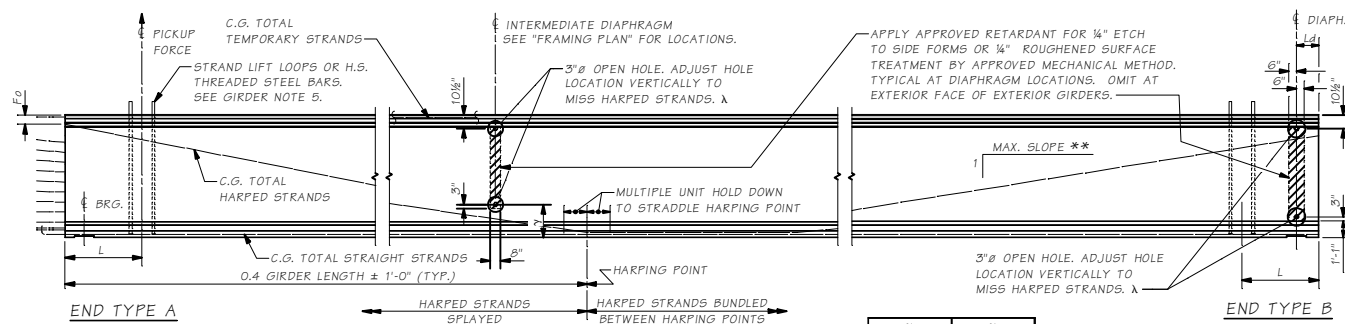
GIRDER ELEVATION
