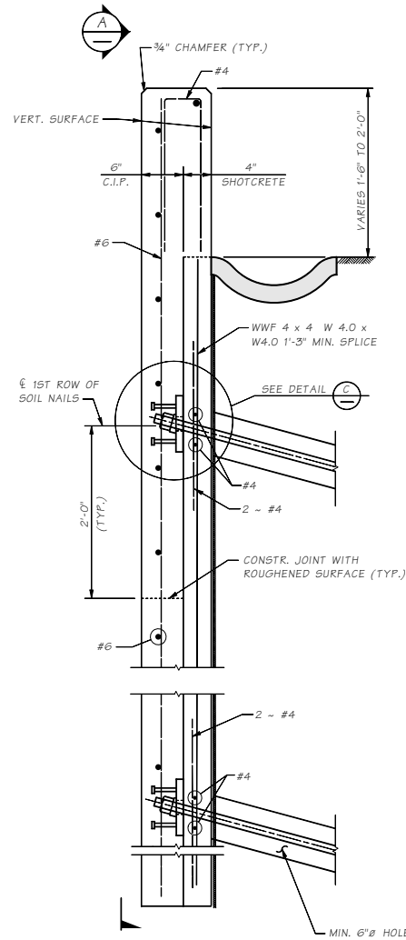
TYPICAL SECTION
