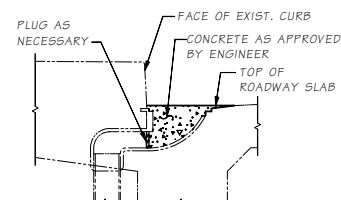
BRIDGE DRAIN PLUG DETAIL
