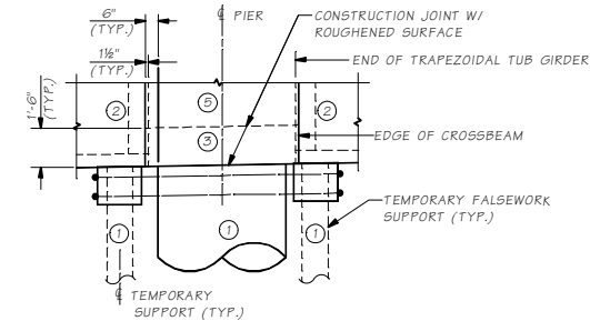
TEMPORARY SUPPORT DETAIL
