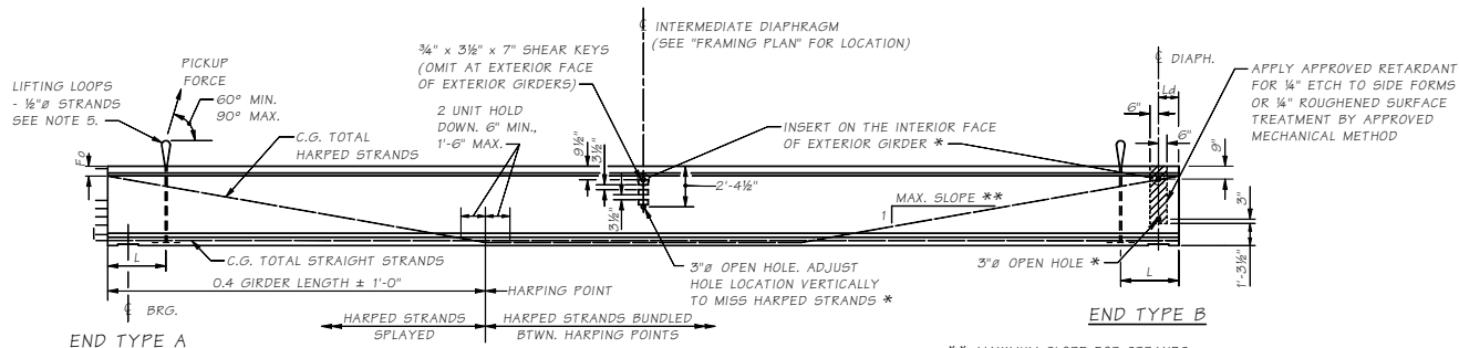
GIRDER ELEVATION
