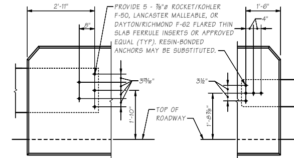
THREE BEAM END SECTION DESIGN "F" (SEE STD. PLAN C-7a)
