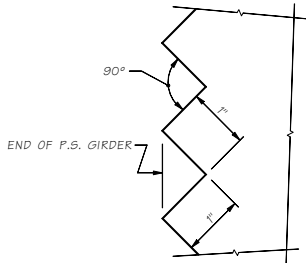
SAWTOOTH DETAILS
