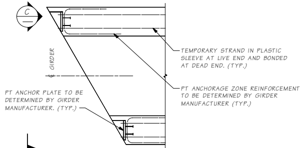
DETAIL B LIVE END SHOWN DEAD END SIMILAR.
