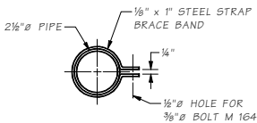
BRACE BAND
