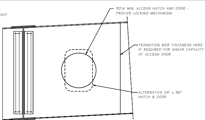
VIEW B SHOWING SIDE EXIT HATCH USE SIDE EXIT HATCH AND WALKWAY BETWEEN BOXES FOR RETURN TRIP INSPECTION ACCESS, AT LEAST ONE END
