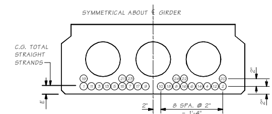
STRAND PATTERN
