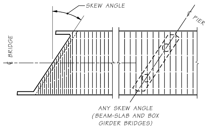
Partial Plans at Abutments
