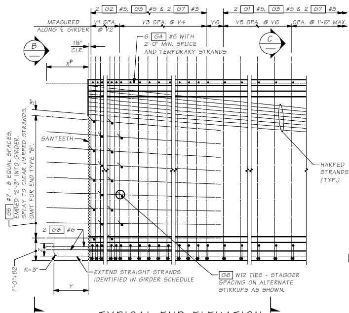
TYPICAL END ELEVATION
