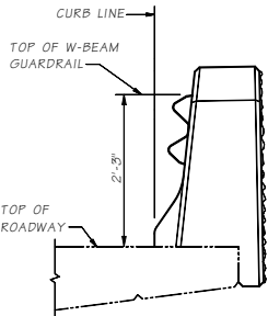
END VIEW W-BEAM SHOWN WITH "D" CONNECTION
