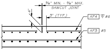
LONGITUDINAL JOINT DETAIL
