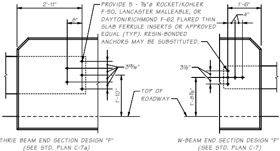
OUTSIDE ELEVATION TRAFFIC BARRIER - GUARDRAIL CONNECTION (WHERE SHOWN ON LAYOUT)
