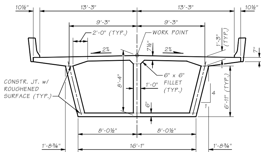
a - 2% CROWN
