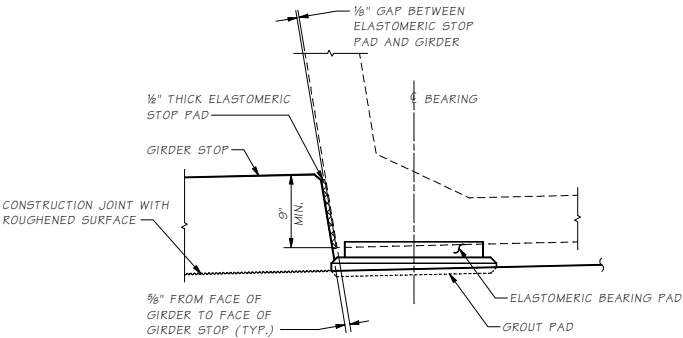
SECTION A
