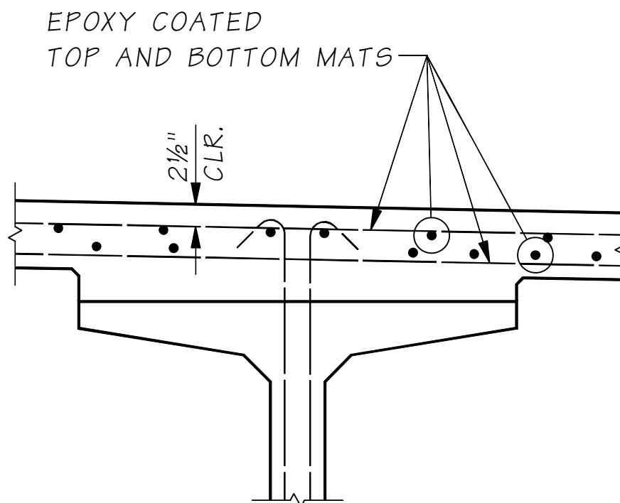
Type 1 Protection System Figure 5.7.4-1
