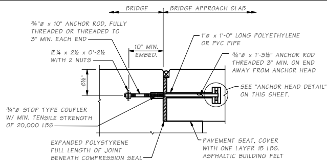
APPROACH ANCHOR - METHOD A
