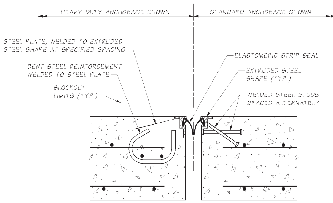
Strip Seal Joint Figure 9.1.4-2
