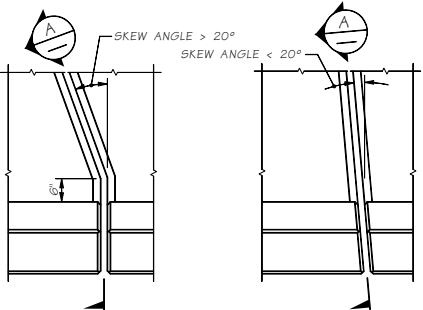
PLAN EXPANSION JOINT
