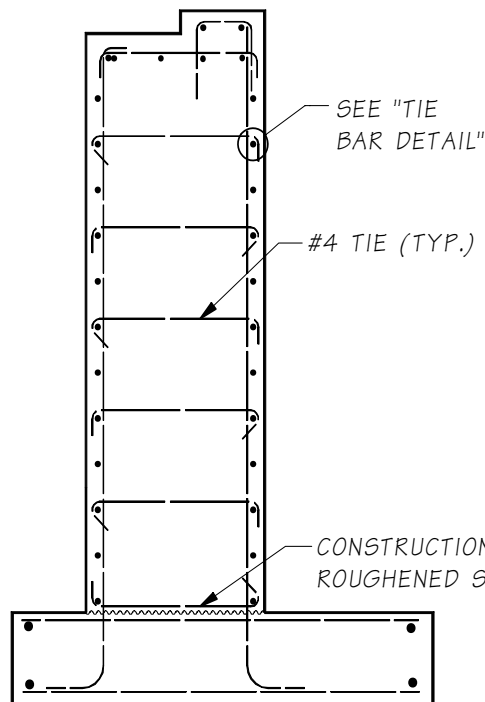
TYPICAL SECTION
