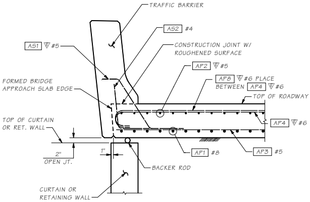
SECTION A 1
