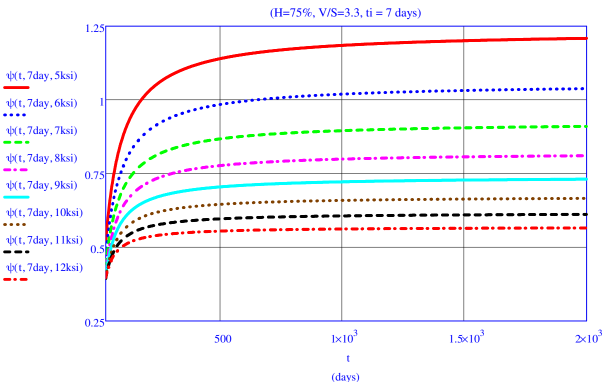
Creep Coefficient for Standard Conditions as Function of Initial Concrete Strength
