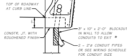
SECTION B WALL
