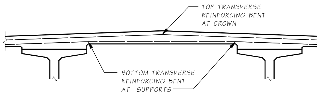
Bottom of Deck Slab at Crown Point
