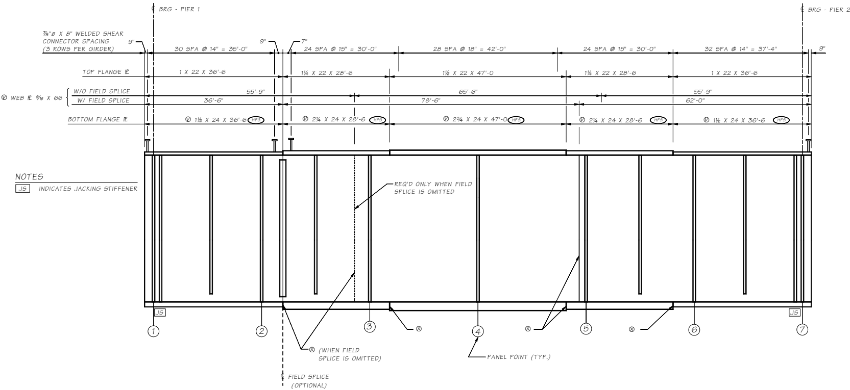
GIRDER ELEVATION
