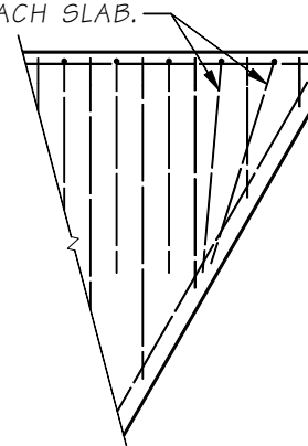
Flared Corner Steel Figure 10.6.4-2
