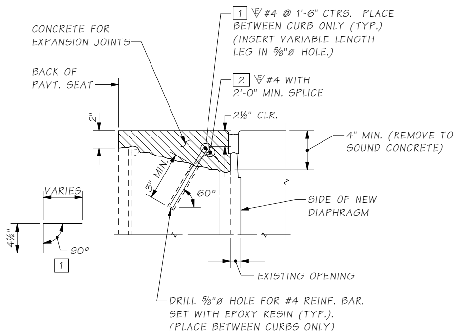
Expansion Joint Detail Shown for Compression Seal With New Reinforcing Steel Added Figure 5.5.5-2
