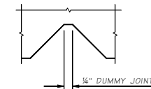
DUMMY JOINT DETAIL
