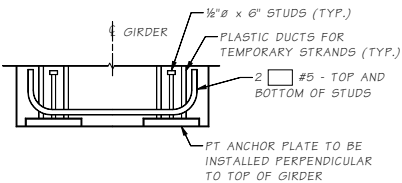
PLAN TEMPORARY STRAND POST-TENSIONED ALTERNATE
