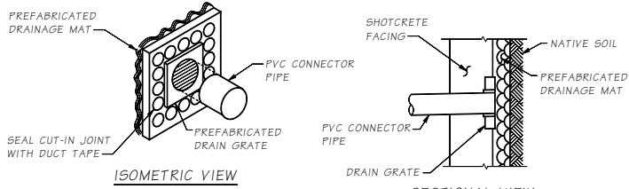
DETAIL G
