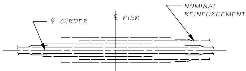
STAGGERED BAR PATTERN FOR BAR LENGTH > 60 FEET
