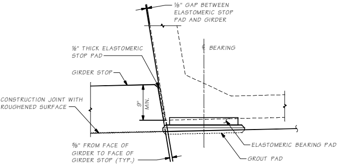
SECTION A
