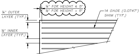
SECTION B
