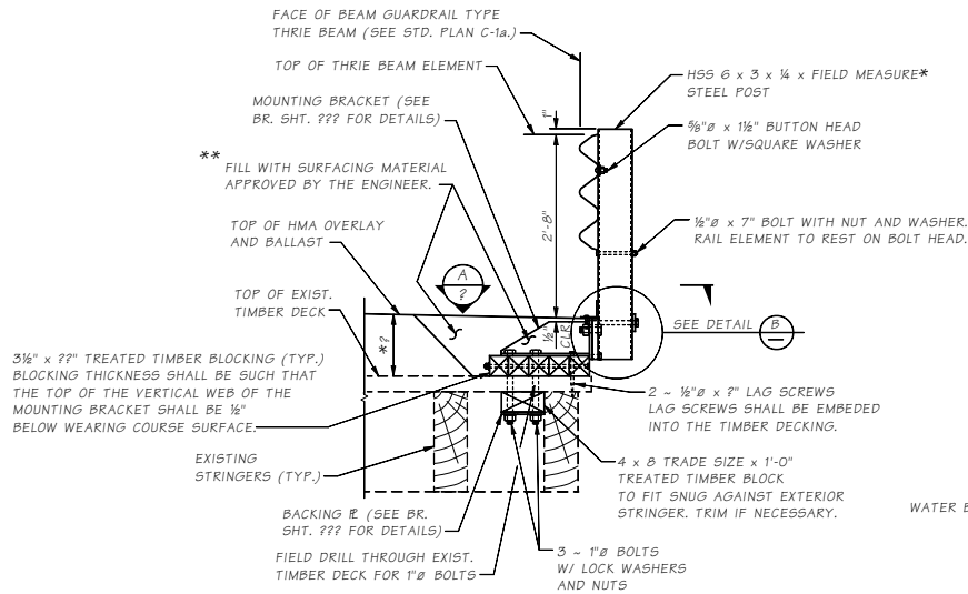
GUARDRAIL POST ASSEMBLY (SEE ASSEMBLIES)
