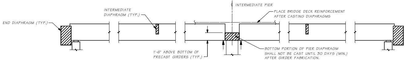
STAGE 2 CAST DIAPHRAGMS AND PLACE BRIDGE DECK REINFORCEMENT INSTALL TEMPORARY BRACING FOR DIAPHRAGM AND DECK PLACEMENT IN ACCORDANCE WITH SECTION 6-02.3(17)F.
