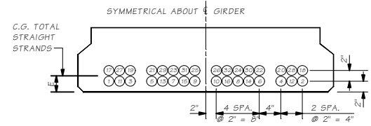
STRAND PATTERN
