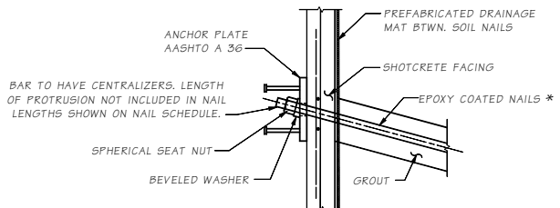
NAIL HEAD DETAIL
