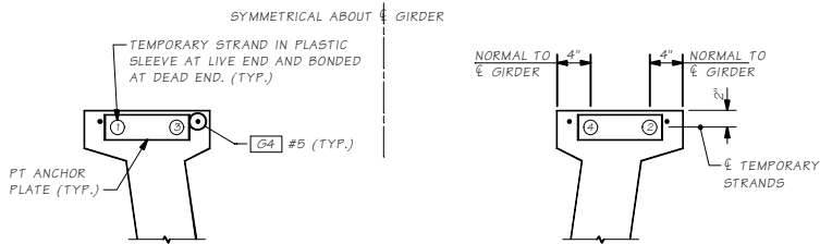
VIEW C
