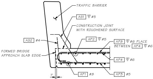
SECTION A 1
