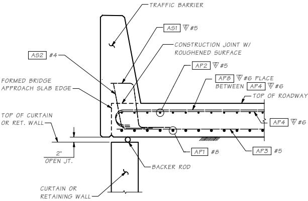
SECTION A 1
