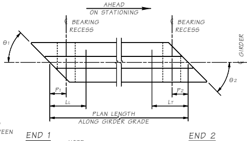
GIRDER SCHEDULE
