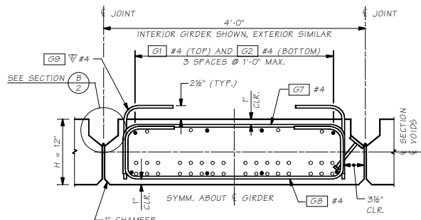
SECTION C
