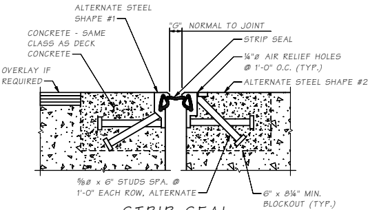
STRIP SEAL
