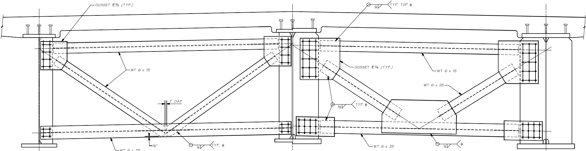
EXAMPLE INTERMEDIATE CROSSFRAME
