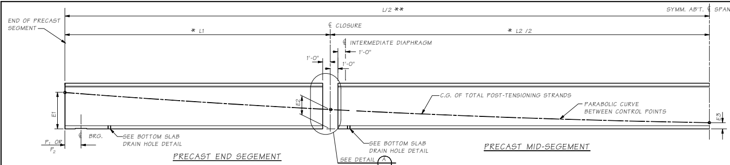
PRECAST LONGITUDINAL HALF-SECTION
