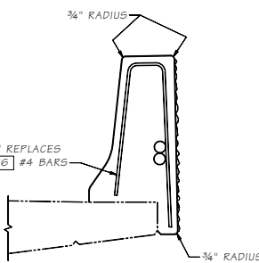
SLIPFORM ALTERNATE
