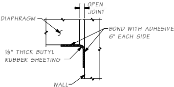
PLAN VIEW BUTYL RUBBER AT VERTICAL JOINTS
