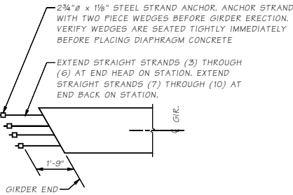
ALTERNATE #2
