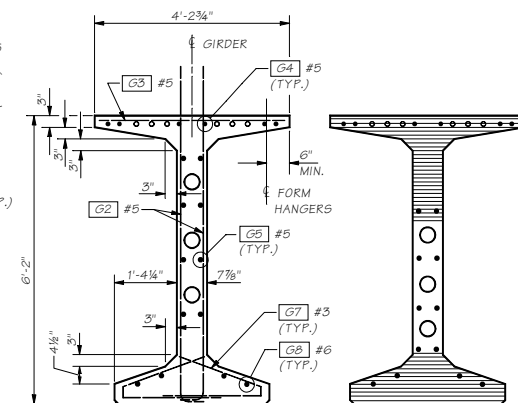
SECTION D
