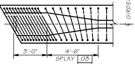
TRANSVERSE REINFORCING AT SKEWED ENDS ONLY TRANSVERSE REINFORCING SHOWN
