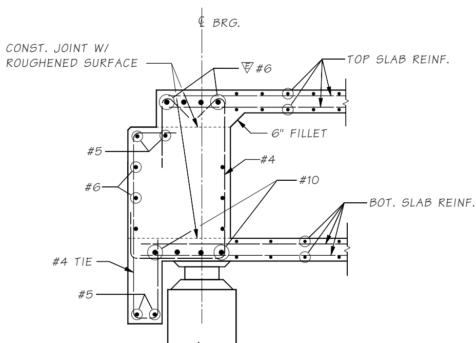
Typical End Diaphragm Reinforcement
