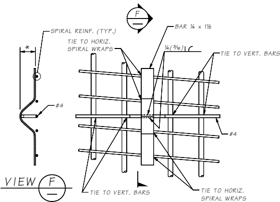
CENTRALIZER DETAIL EPOXY COAT CENTRALIZER OR PAINT WITH INORGANIC ZINC AFTER FABRICATION (OPTION 2)
