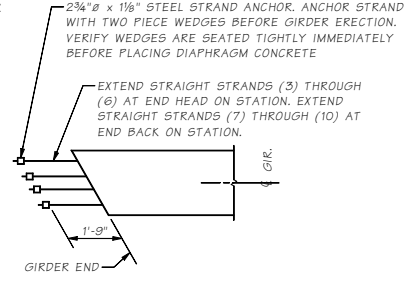
ALTERNATE #2
