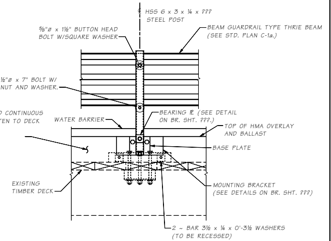
OUTSIDE ELEVATION AT TYPICAL GUARDRAIL POST
