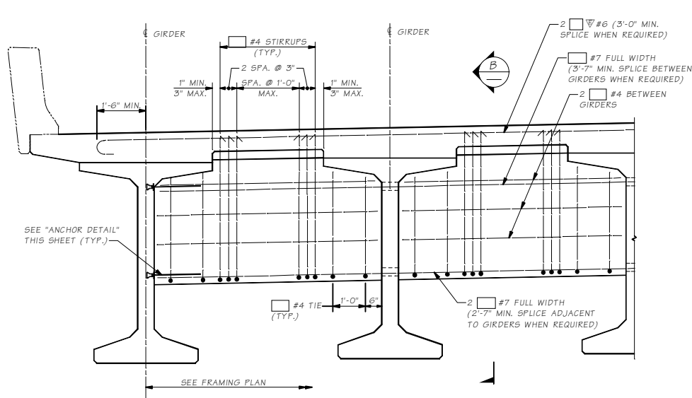
ELEVATION INTERMEDIATE DIAPHRAGM DIMENSIONS ARE ALONG DIAPHRAGM
