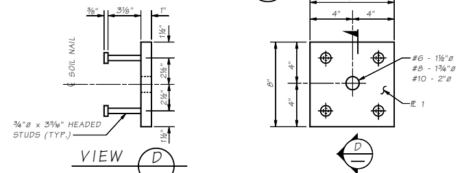
ANCHOR PLATE DETAILS
