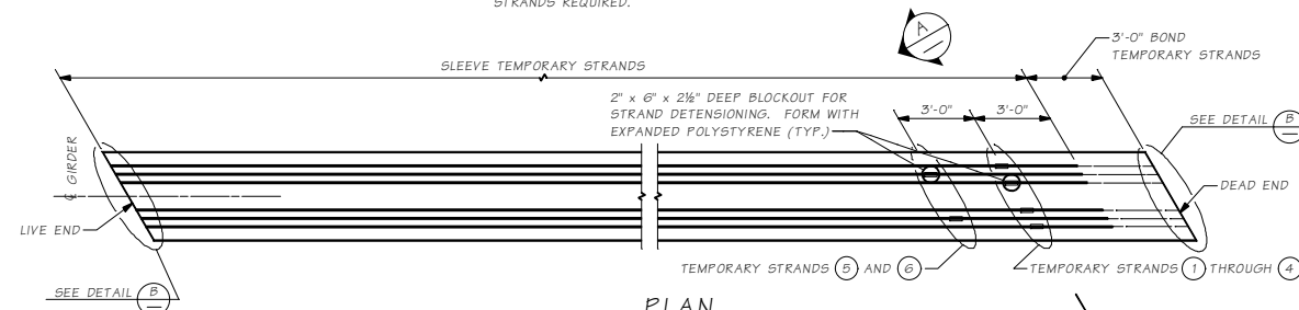
PLAN POST-TENSIONED TEMPORARY TOP STRANDS ALTERNATE SEE "GIRDER SCHEDULE" FOR NUMBER OF TEMPORARY STRANDS REQUIRED. POST-TENSIONED ALTERNATE ONLY AVAILABLE FOR 6 OR FEWER TEMPORARY STRANDS.
