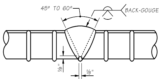
SINGLE V-GROOVE WELD AWS D1.4 FIGURE 3.2(A)
