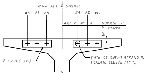
END VIEW TEMPORARY STRAND POST-TENSIONED ALTERNATE
