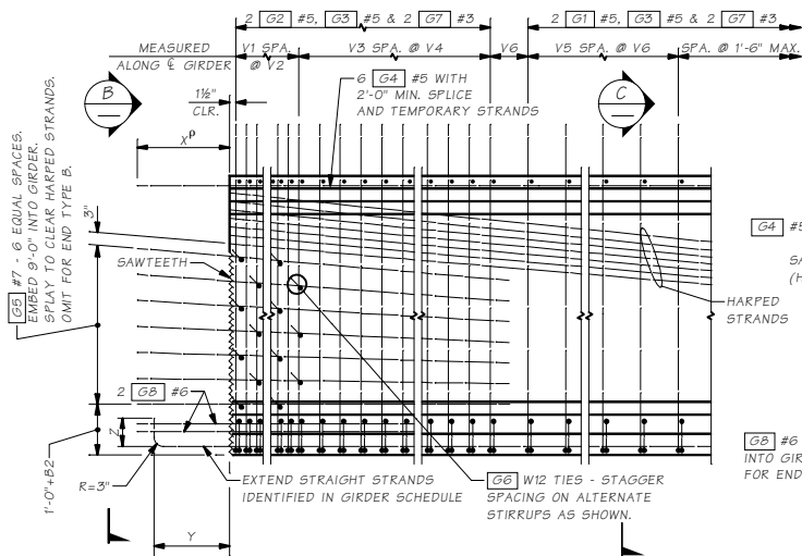
TYPICAL END ELEVATION
