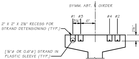
SECTION A
