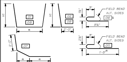
BENDING DIAGRAM (ALL DIMENSIONS ARE OUT TO OUT)
