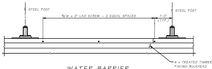
WATER BARRIER PLAN
