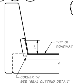
SECTION C
