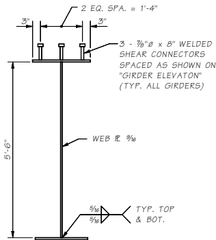
TYPICAL GIRDER SECTION
