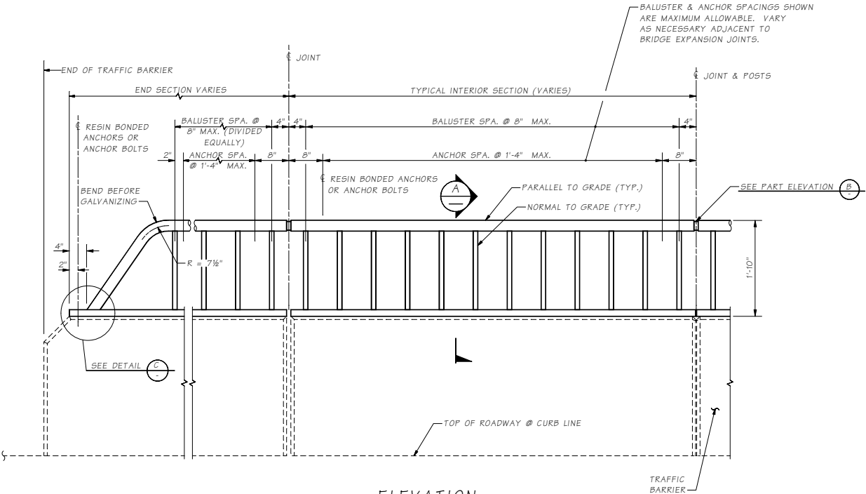
ELEVATION BALUSTER ATTACHMENT DETAILS NOT SHOWN
