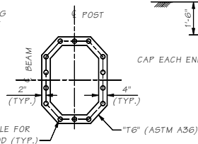
ANCHOR & DETAIL
