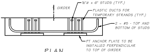
PLAN TEMPORARY STRAND POST-TENSIONED ALTERNATE
