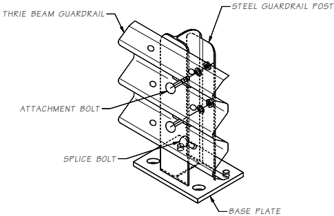
ISOMETRIC VIEW
