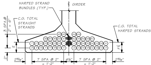
STRAND PATTERN AT C SPAN
