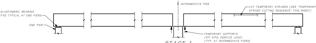
STAGE 1 SET GIRDERS ON TEMPORARY SUPPORT INSTALL TEMPORARY BRACING FOR ERECTION IN ACCORDANCE WITH SECTION 6-02.3(17)F.
