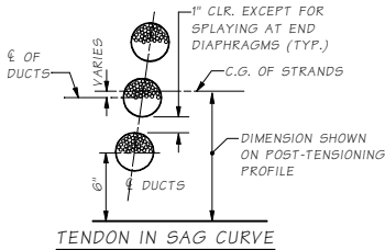
STRAND LOCATION DETAIL
