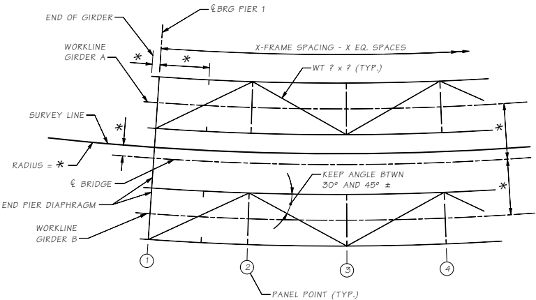
EXAMPLE - PARTIAL FRAMING PLAN * PROVIDE PROJECT DIMENSIONS AND SPECIFY HOW MEASURED
