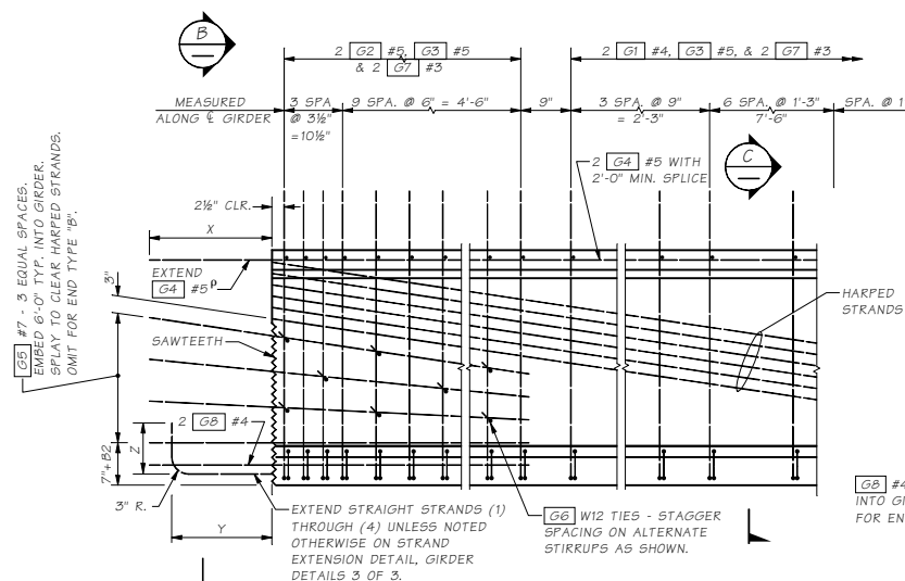
TYPICAL END ELEVATION
