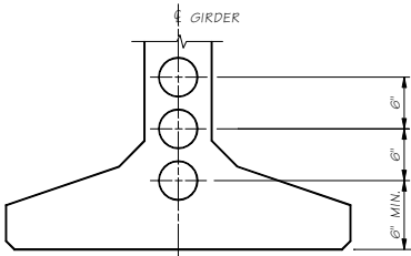
POST-TENSIONING STRAND PATTERN AT \frac{1}{2} SPAN
