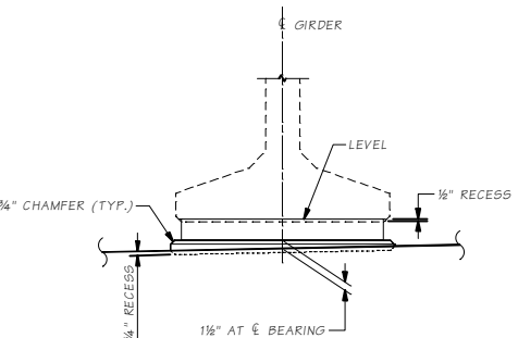
GROUT PAD ELEVATION
