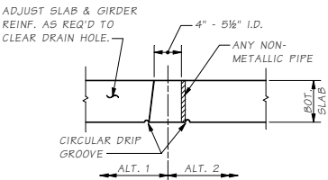
BOTTOM SLAB DRAIN HOLE
