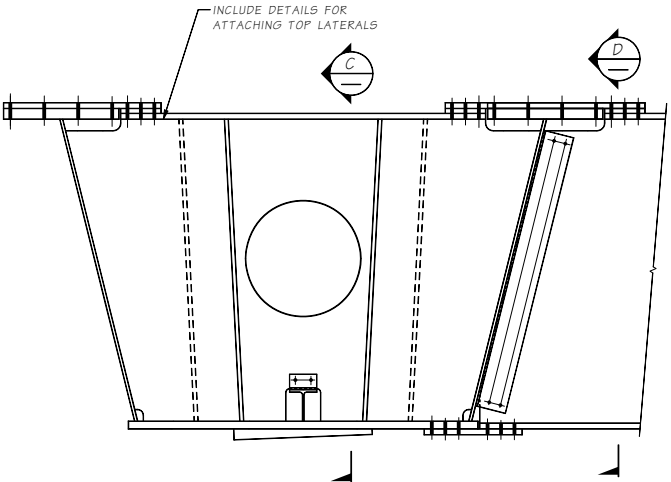
EXAMPLE INTERIOR PIER DIAPHRAGM
