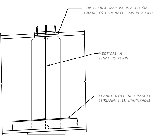
SECTION C
