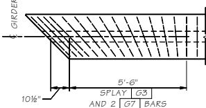
TRANSVERSE REINFORCING SKEWED ENDS
