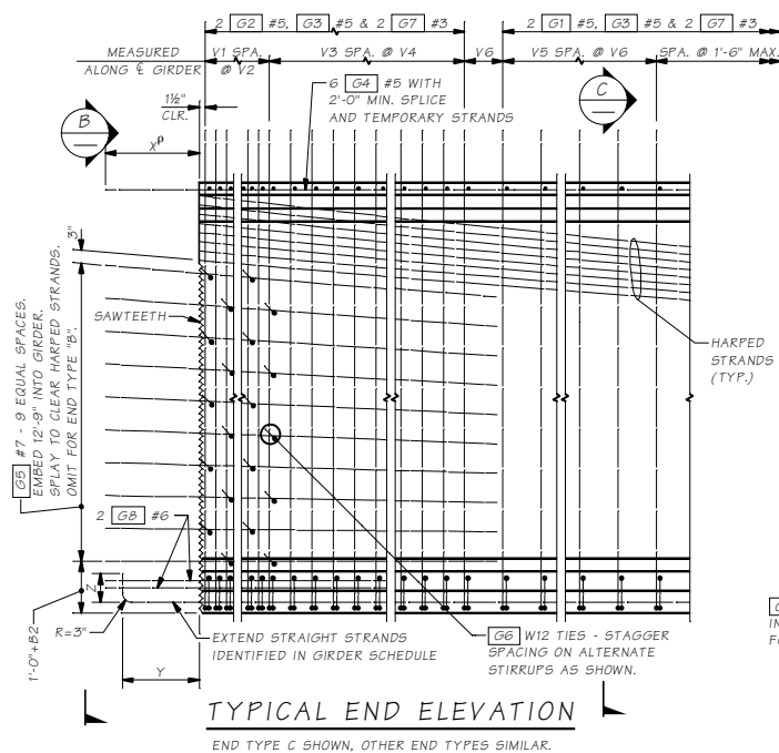
GIRDER ELEVATION
