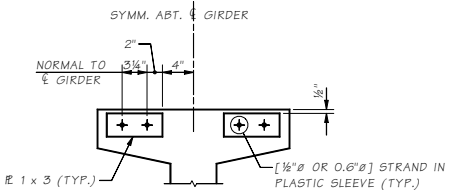
END VIEW TEMPORARY STRAND POST-TENSIONED ALTERNATE
