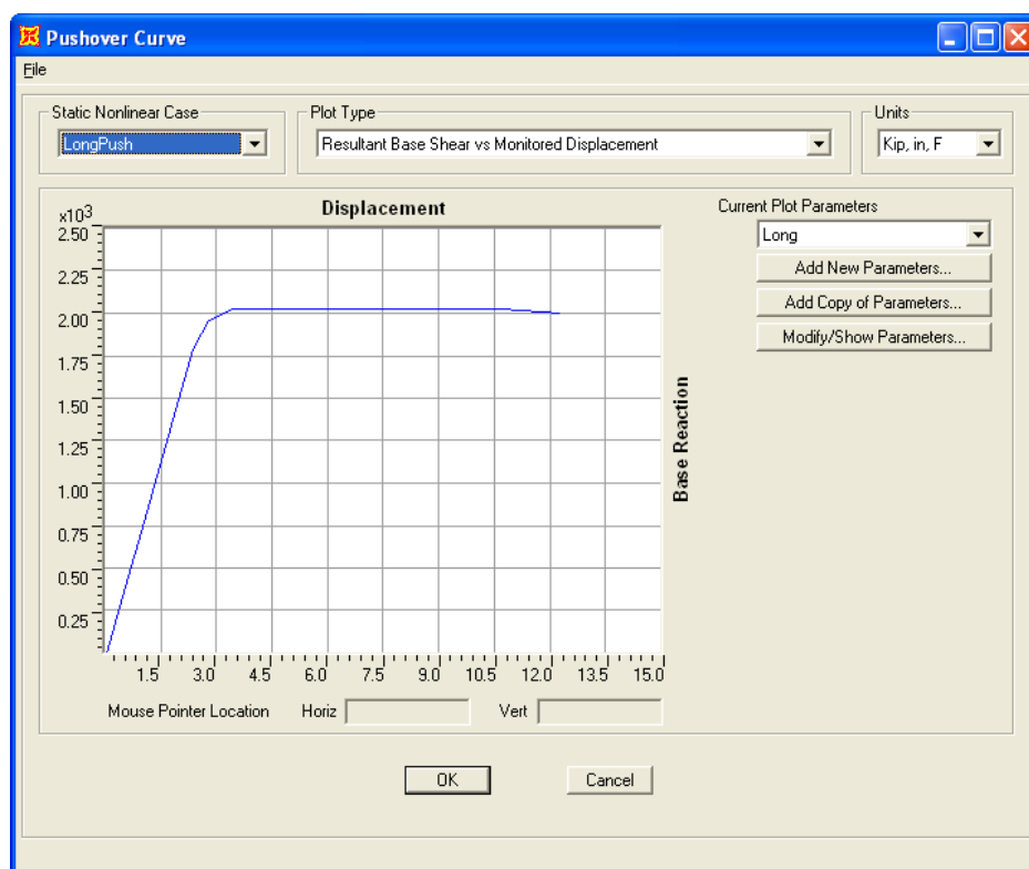
Pushover Curve for Load Case “LongPush” Figure 5.3.1-1
