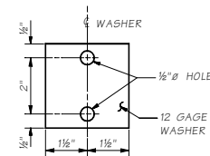
WASHER DETAIL HOT DIP GALVANIZE AFTER FABRICATION
