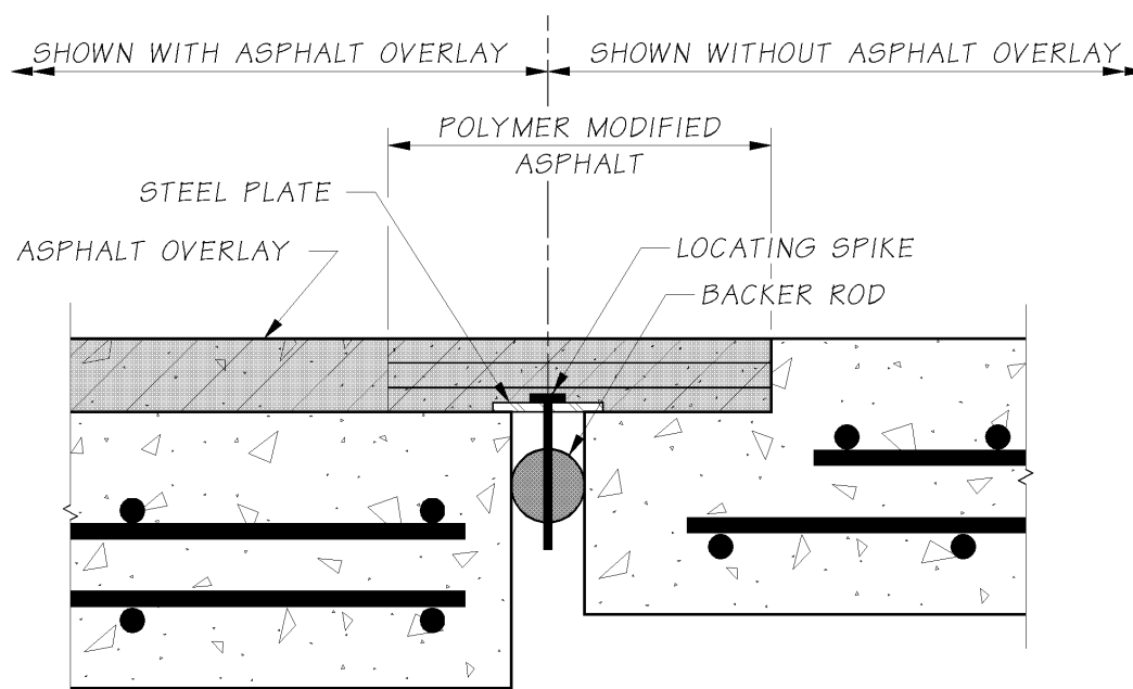
Asphaltic Plug Joint
