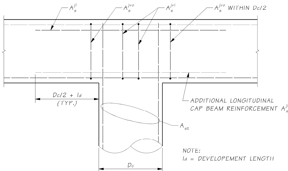
Figure 8.13.5.1.3-1 Additional Longitudinal Cap Beam Reinforcement for Joint Force Transfer BDM Figure 4.2.44-1
