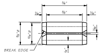
DRIVE PIN DETAIL SLOTTED TYPE SPRING PIN (ANSI B18.2.2)
