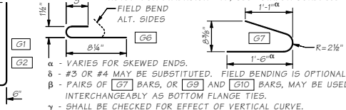
SECTION C
