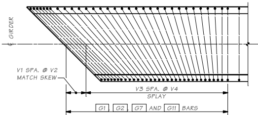
TRANSVERSE REINFORCING SKEWED ENDS LENGTH OF G1 AND G7 VARY WITH SKEW. ONLY TRANSVERSE REINFORCEMENT SHOWN.
