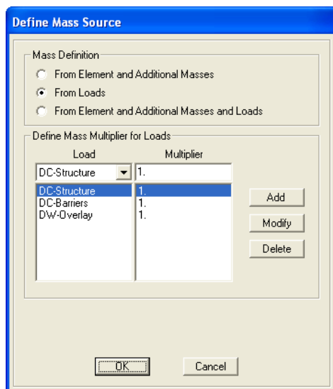
Mass Source Definition Figure 3.1.1-1
