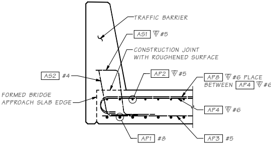
SECTION A 1
