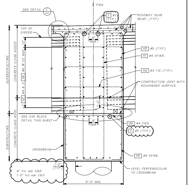
SECTION A
