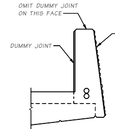
SECTION C
