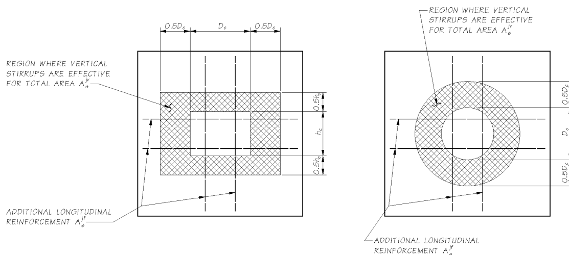
Figure 6.4.8-1 Vertical Joint Shear Reinforcement Region BDM Figure 4.2.21-1
