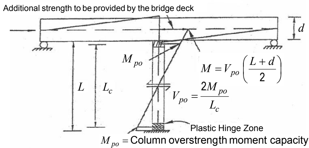
(a) Longitudinal Response for Nonintegral Abutments
