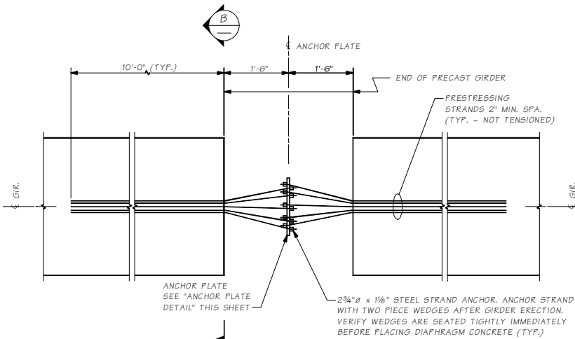
ADDITIONAL STRAND EXTENSION DETAIL
