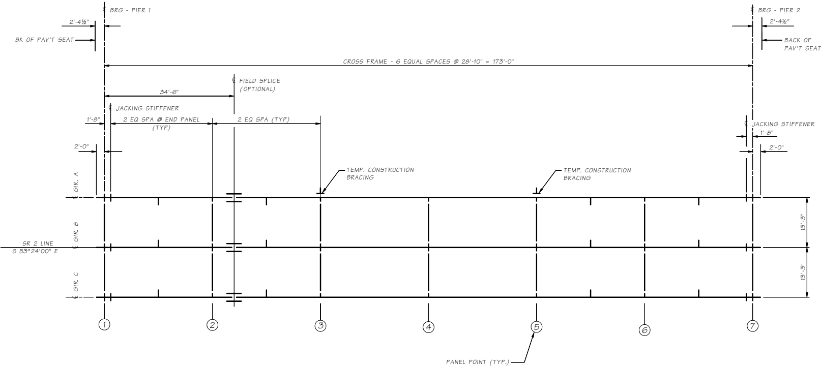
FRAMING PLAN
