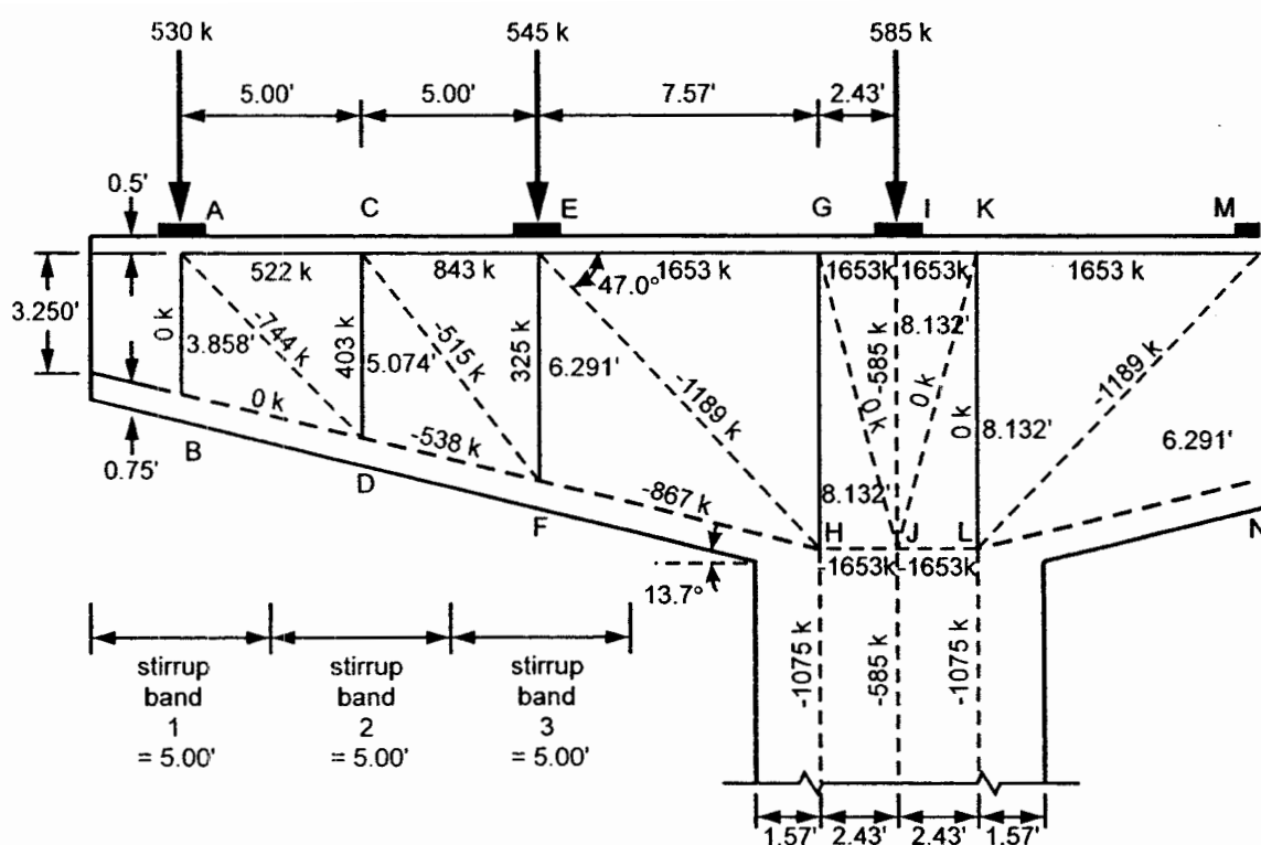
Figure 5.2. Truss idealization.
