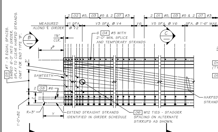
TYPICAL END ELEVATION
