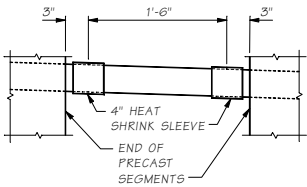
DUCT SPLICE DETAIL
