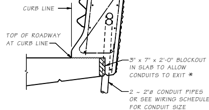
SECTION B BRIDGE
