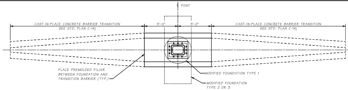
PLAN BARRIER TRANSITION
