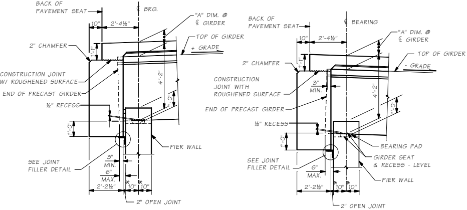
END DIAPHRAGM GEOMETRY
