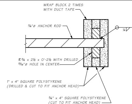
ANCHOR HEAD DETAIL
