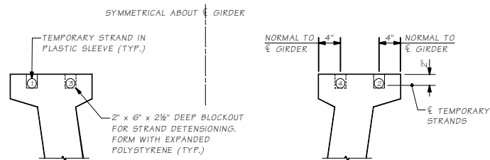
SECTION A
