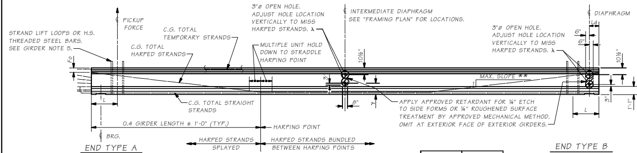
GIRDER ELEVATION
