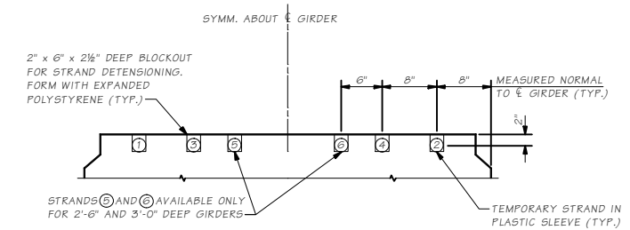
SECTION D
