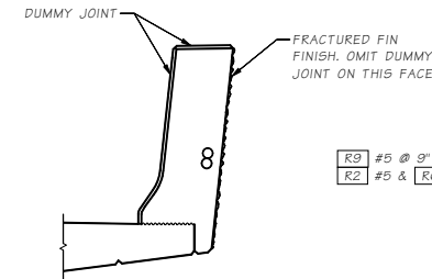
SECTION C
