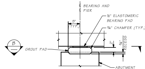
DETAIL C
