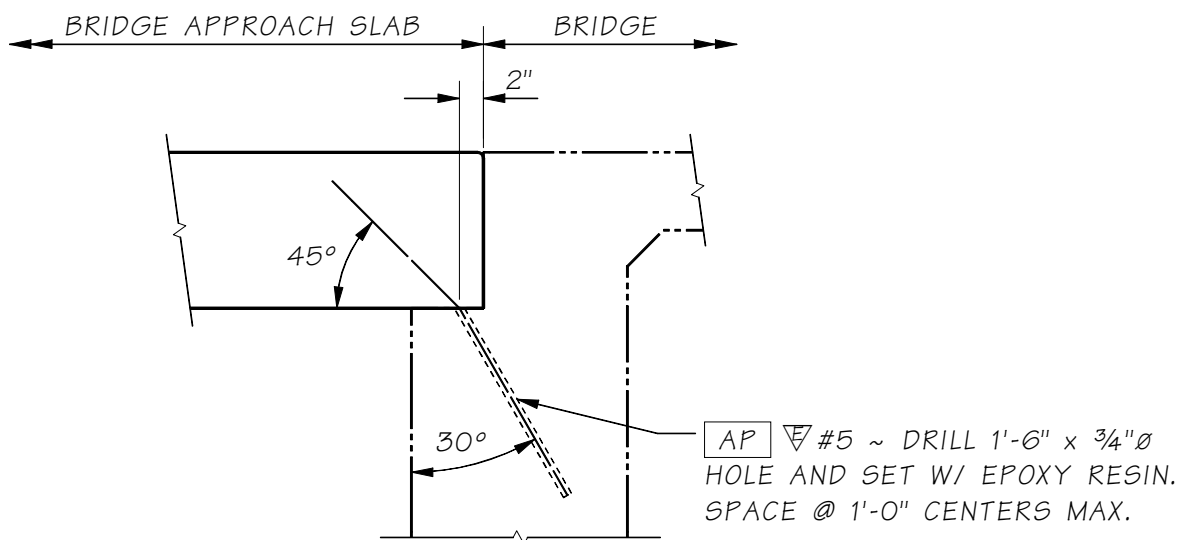
Pinned Approach Slab Detail
