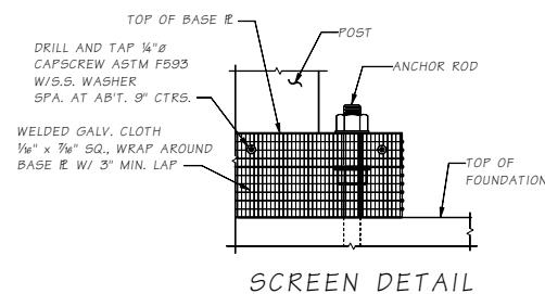
SCREEN DETAIL
