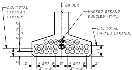
STRAND PATTERN AT SPAN
