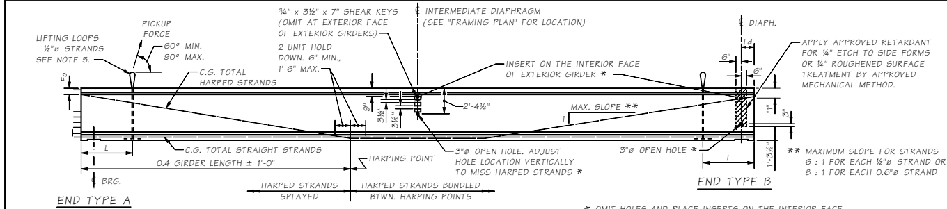
GIRDER ELEVATION
