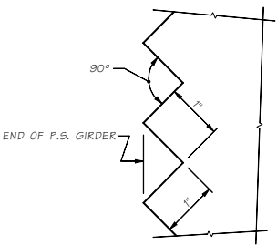
SAWTOOTH DETAILS
