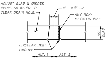
BOTTOM SLAB DRAIN HOLE
