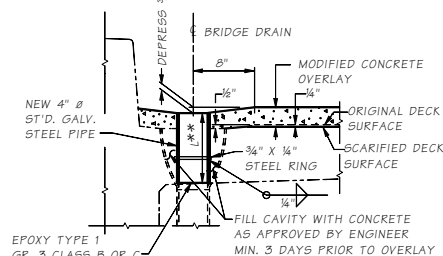
SECTION C
