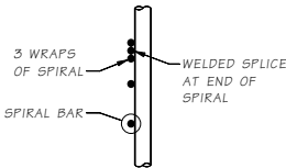
SPIRAL TERMINATION DETAIL
