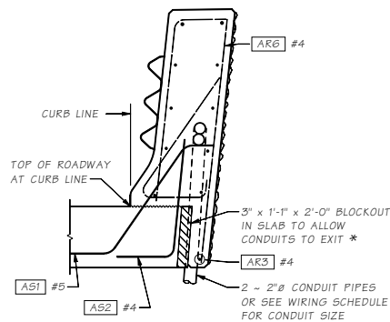
SECTION B APPROACH SLAB
