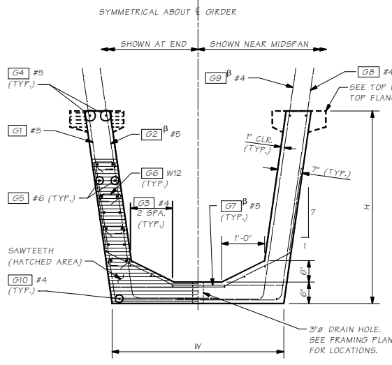
TYPICAL SECTION
