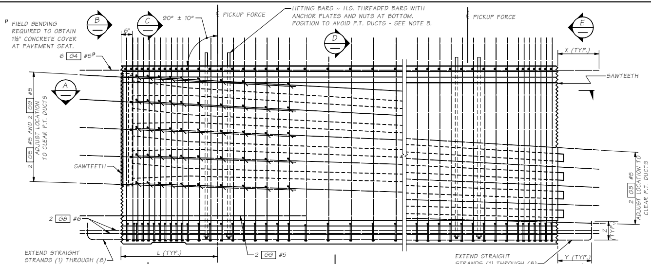
TYPICAL END ELEVATION AT CLOSURE
