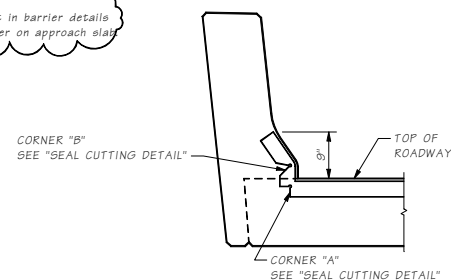
SECTION C
