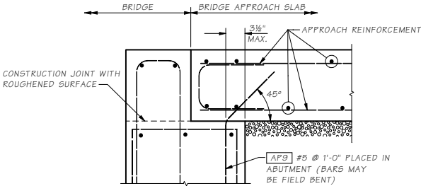
ANCHOR DETAIL
