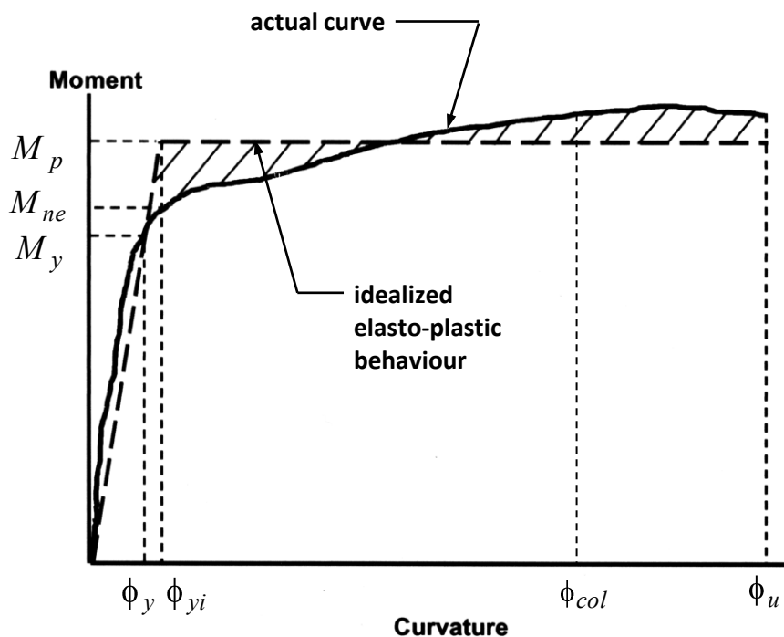
Figure C 4.9-1 Moment-Curvature Diagram BDM Figure 4.2.10-1
