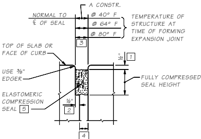
COMPRESSION SEAL CONCRETE OPENING
