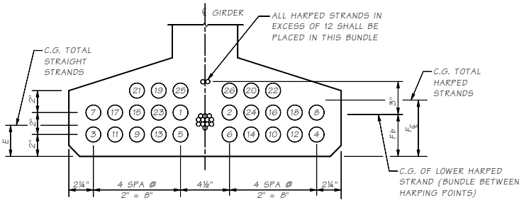
STRAND PATTERN AT \frac{1}{2} SPAN
