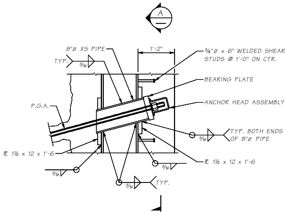
ELEVATION - SOLDIER PILE WITH P.G.A. THRU WEB
