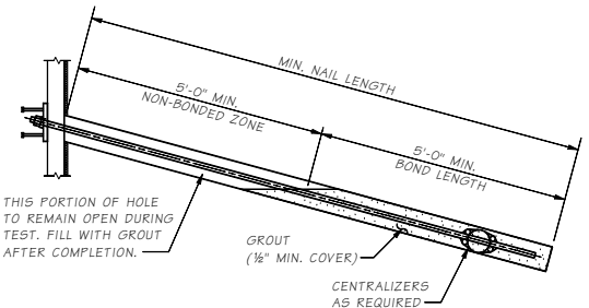
TEST NAIL DETAIL
