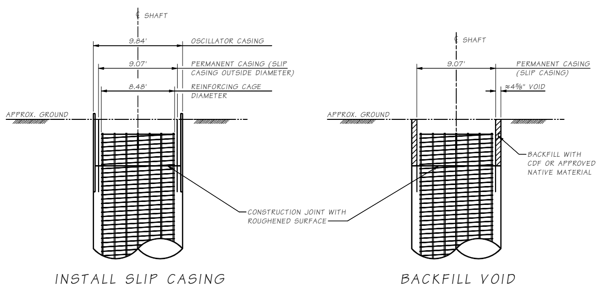
10'-0" Ø Shaft Constructed With The Oscillator Method
