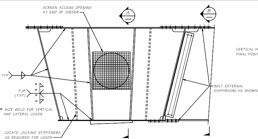
EXAMPLE END DIAPHRAGM
