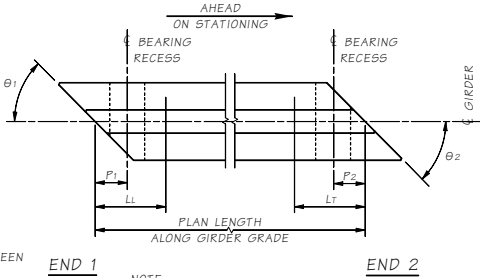
GIRDER SCHEDULE
