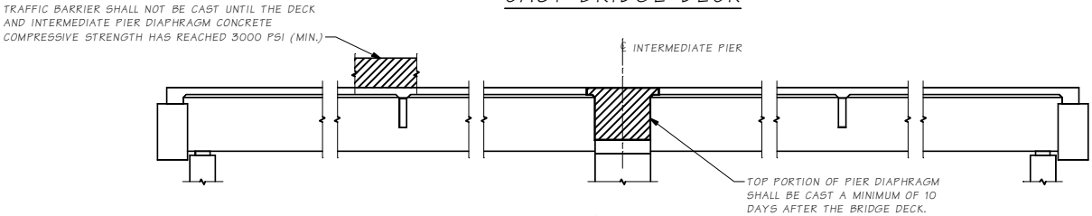
STAGE 4 COMPLETE DIAPHRAGMS
