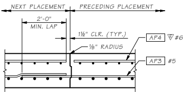
ALTERNATE LONGITUDINAL JOINT DETAIL
