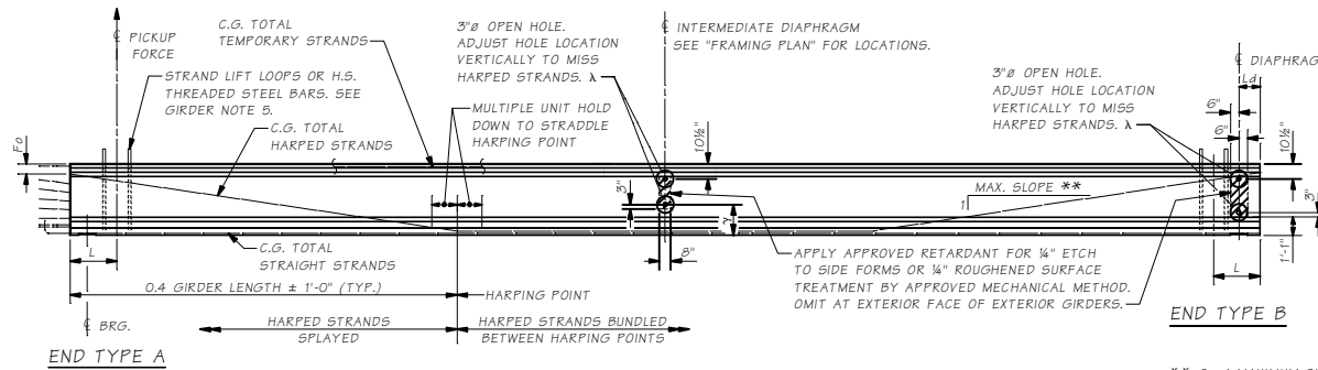
GIRDER ELEVATION
