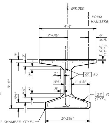
SECTION (C)
