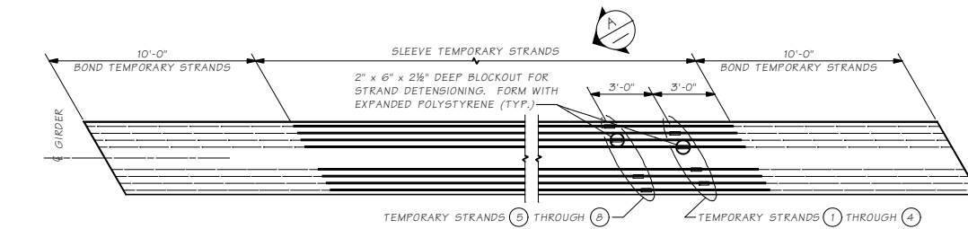
PLAN PRETENSIONED TEMPORARY TOP STRANDS ALTERNATE SEE "GIRDER SCHEDULE" FOR NUMBER OF TEMPORARY STRANDS REQUIRED.
