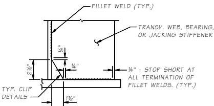
TYPICAL FILLET WELD TERMINATION DETAIL
