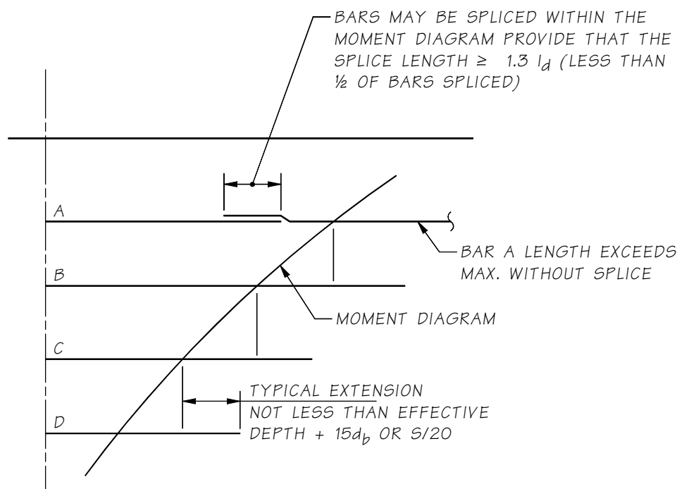
Bar Splice Within Moment Envelope
