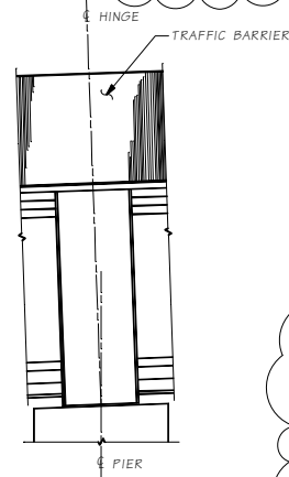
END VIEW HINGE DIAPHRAGM
