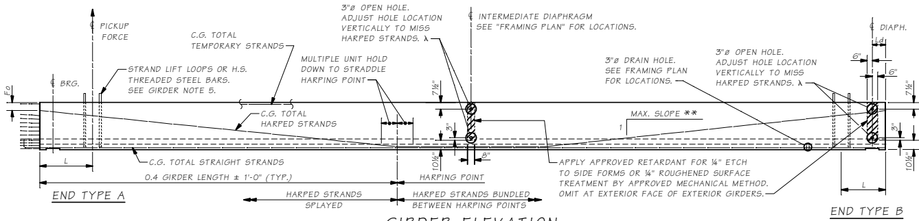
GIRDER ELEVATION
