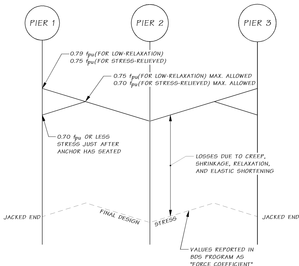
Stress Diagram for a 2-Span PT Bridge
