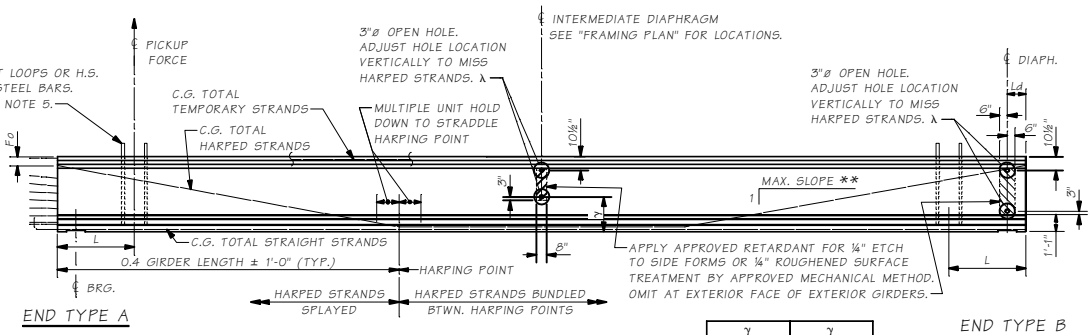
GIRDER ELEVATION
