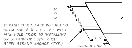
STRAND EXTENSION DETAIL ANCHOR STRAND WITH TWO PIECE WEDGES BEFORE GIRDER ERECTION. VERIFY WEDGES ARE SEATED TIGHTLY IMMEDIATELY BEFORE PLACING DIAPHRAGM CONCRETE.
