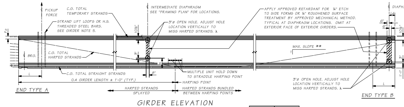
GIRDER ELEVATION
