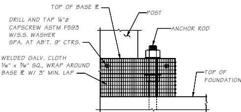
SCREEN DETAIL
