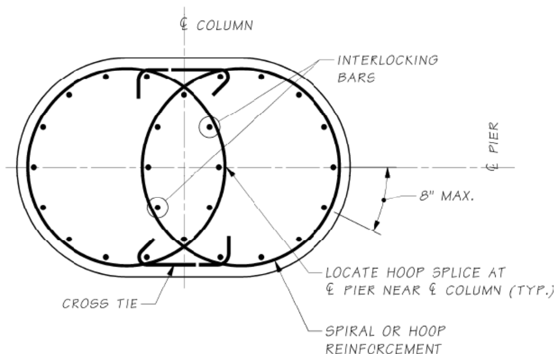
Figure C8.6.3-3 Column Interlocking Spiral and Hoop Details
