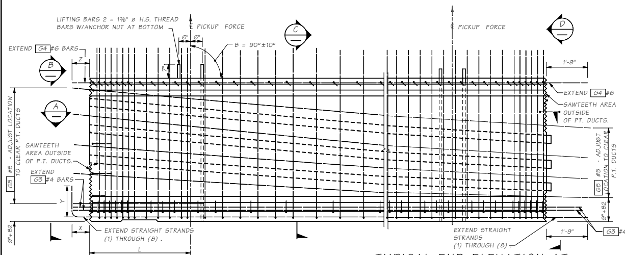
TYPICAL END ELEVATION AT END DIAPHRAGMS
