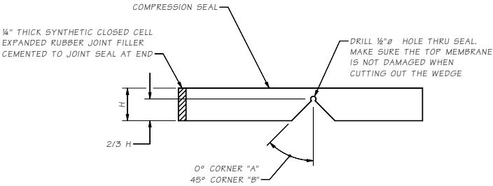
SEAL CUTTING DETAIL
