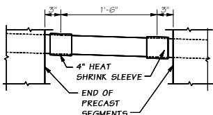
DUCT SPLICE DETAIL
