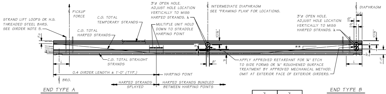
GIRDER ELEVATION
