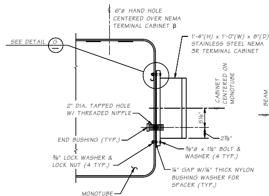
NEMA 3R TERMINAL CABINET DETAIL
