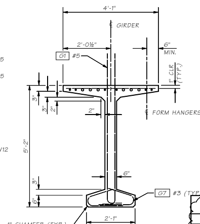
SECTION C
