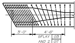
TRANSVERSE REINFORCING AT SKEWED ENDS
