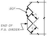
SAWTOOTH DETAILS
