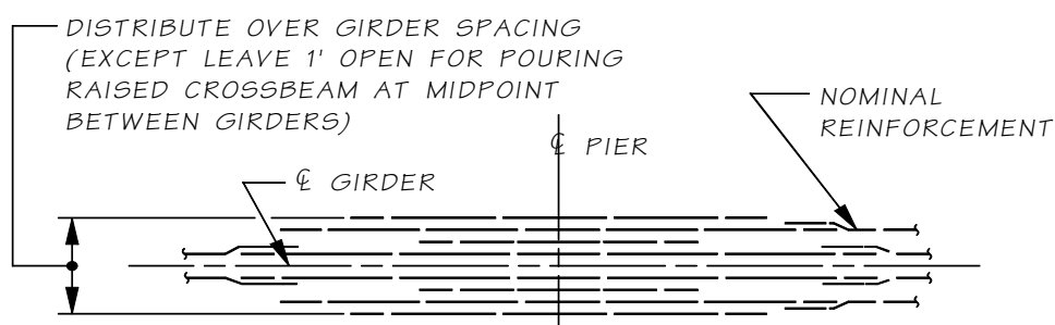
SYMMETRICAL BAR PATTERN FOR BAR LENGTH < 60 FEET
