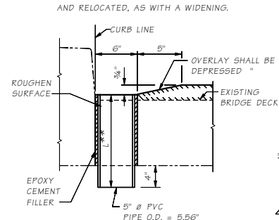
ELEVATION VIEW STRAIGHT DROP
