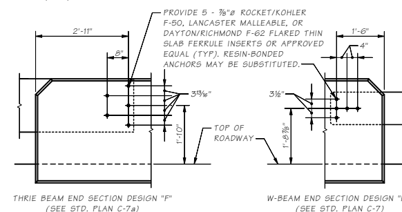
OUTSIDE ELEVATION TRAFFIC BARRIER - GUARDRAIL CONNECTION (WHERE SHOWN ON LAYOUT)
