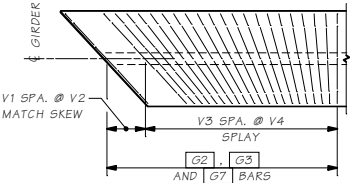
TRANSVERSE REINFORCING SKEWED ENDS
