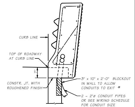
SECTION B WALL
