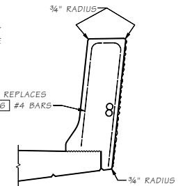
SLIPFORM ALTERNATE
