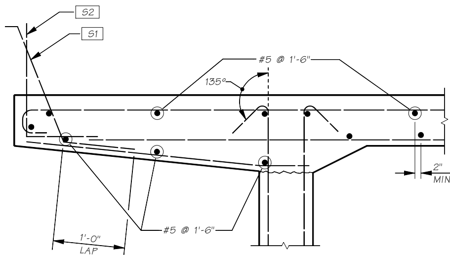
Overhang Detail
