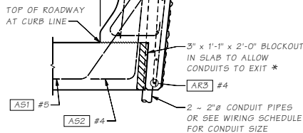
SECTION (B) APPROACH SLAB
