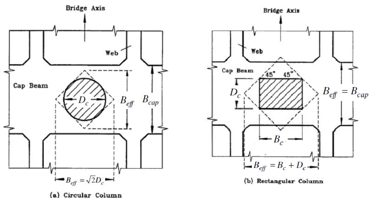
Figure 8.13.2-1 Effective Joint Width for Shear Stress Calculation BDM Figure 4.2.42-1
