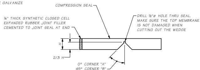
SEAL CUTTING DETAIL
