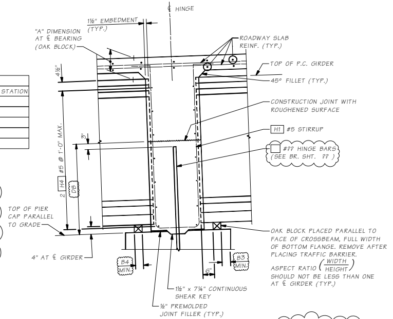
SECTION A
