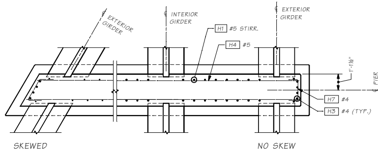
SECTION B
