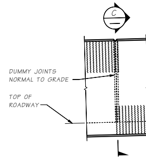
VIEW A ?
