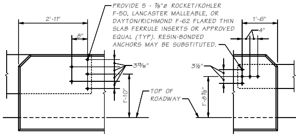
THRE BEAM END SECTION DESIGN "F" (SEE STD. PLAN C-7a) W-BEAM END SECTION DESIGN "F" (SEE STD. PLAN C-7)
