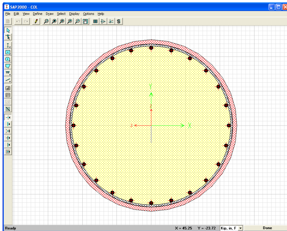
Section Designer View of Frame Section “COL” Figure 2.4-2
