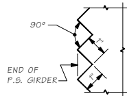
SAWTOOTH DETAILS SAWTEETHS ARE FULL WIDTH - USE SAWTOOTH KEYS FROM BOTTOM OF BOTTOM FLANGE TO BOTTOM OF LOWEST HARPED STRAND AS WELL AS TOP FLANGE ADJACENT TO HARPED STRANDS.
