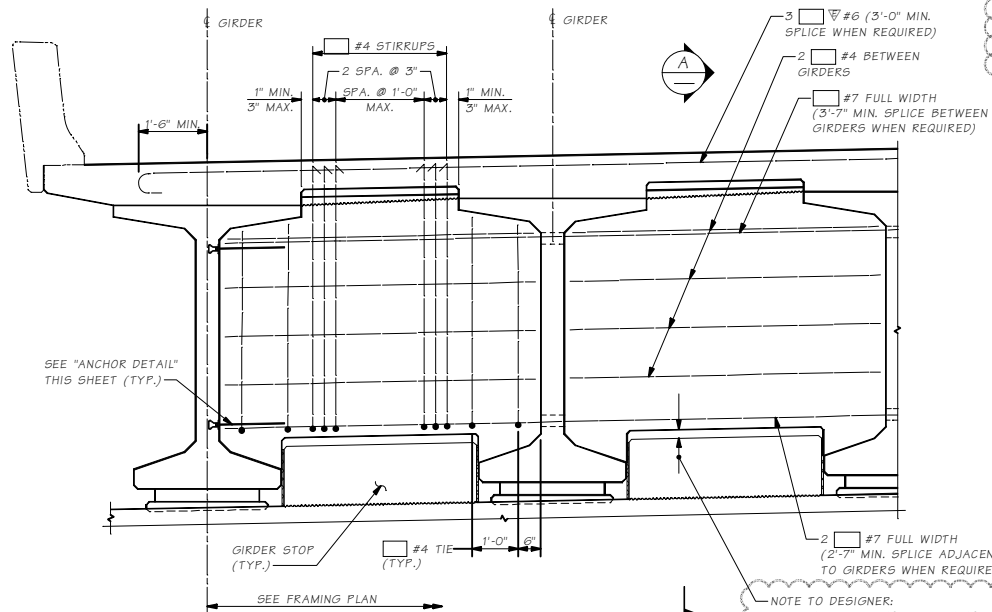
ELEVATION END DIAPHRAGM DIMENSIONS ARE ALONG \bar{C} DIAPHRAGM
