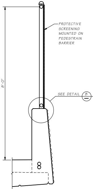
TYPICAL SECTION PROTECTIVE SCREEN
