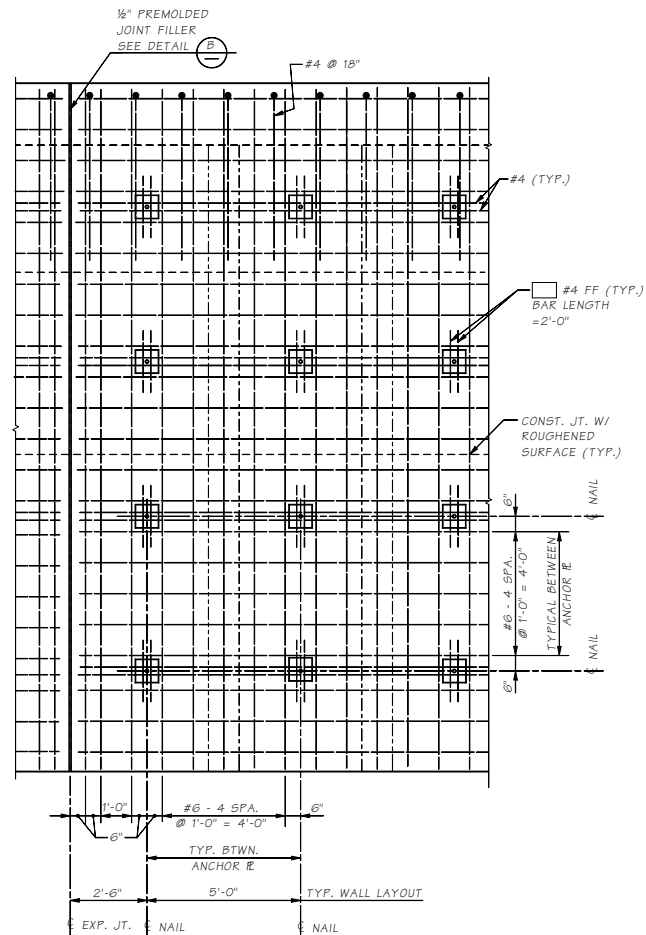
FASCIA WALL REINFORCEMENT WWF NOT SHOWN FOR CLARITY
