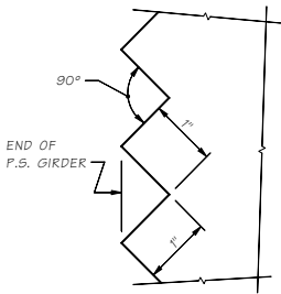
SAWTOOTH DETAILS
