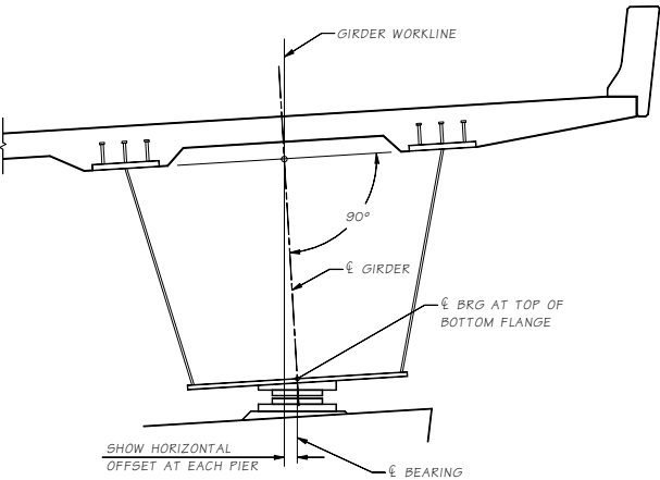
BEARING OFFSET DETAIL
