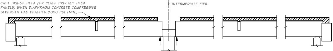
STAGE 3 CAST BRIDGE DECK
