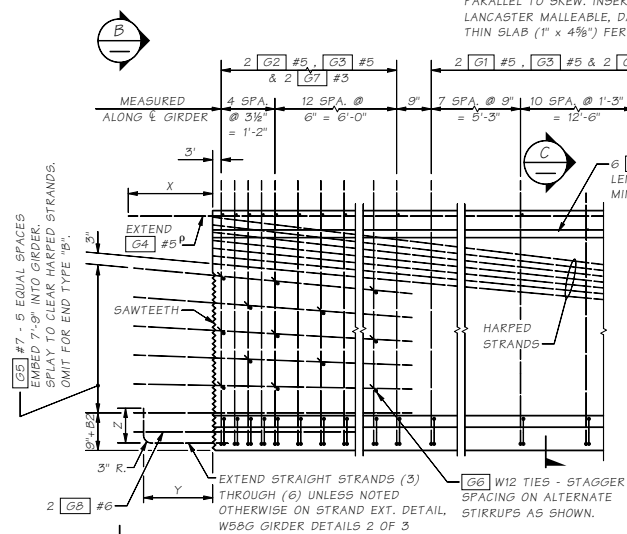
TYPICAL END ELEVATION
