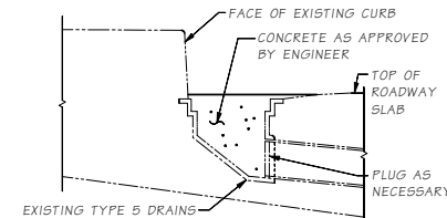
BRIDGE DRAIN PLUG DETAL
