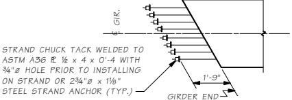
STRAND EXTENSION DETAIL
