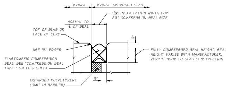
COMPRESSION SEAL DETAIL
