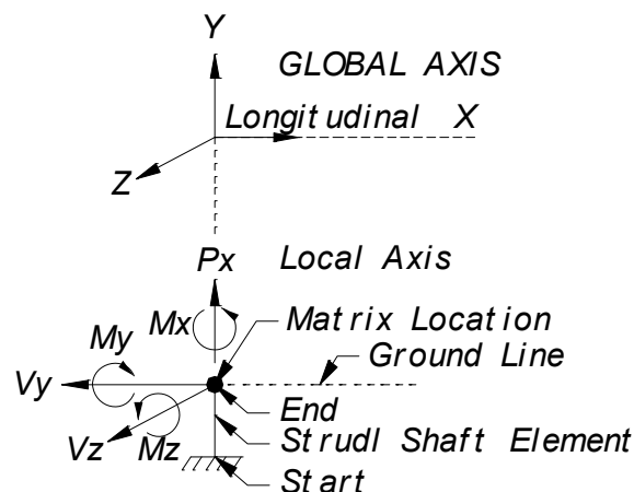
GTStrudl Local Axis Coordinate System
