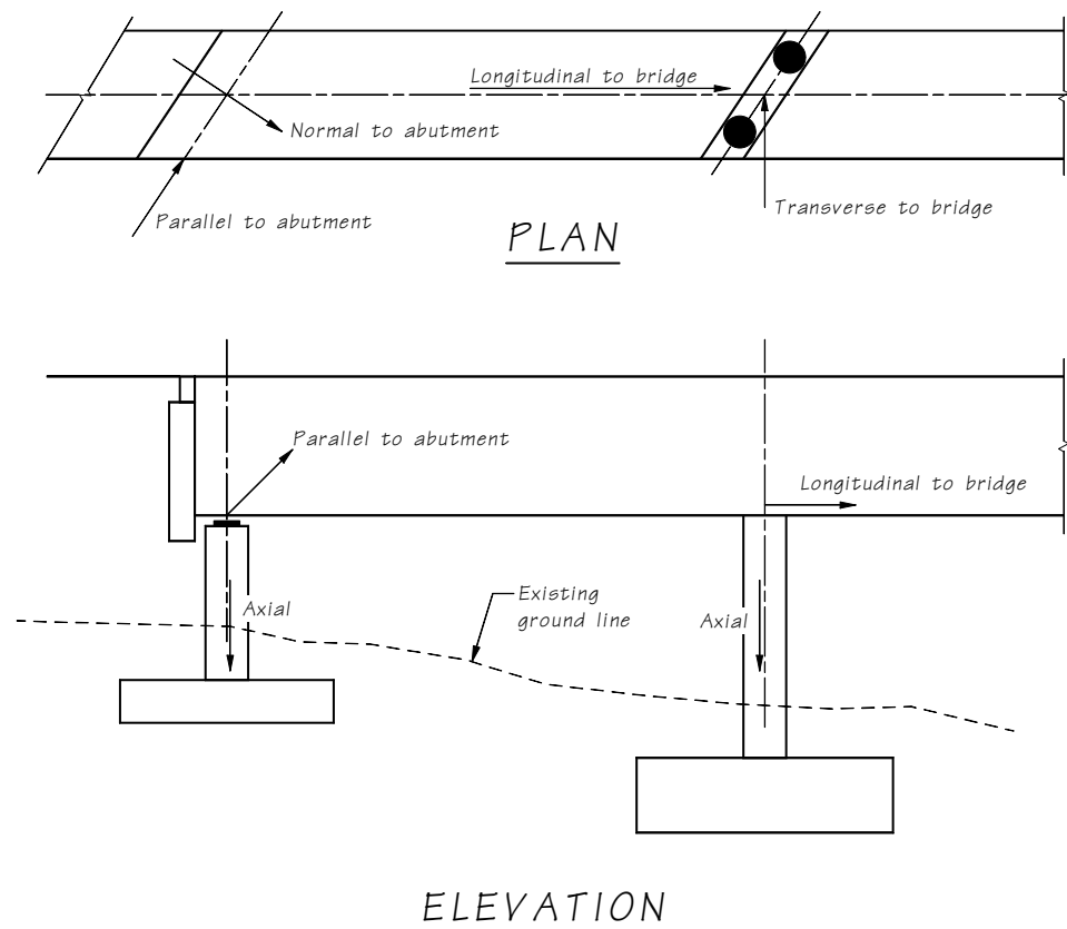
Substructure Directional Forces
