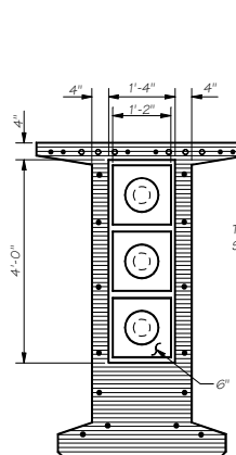
VIEW B
