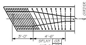
TRANSVERSE REINFORCING AT SKEWED ENDS
