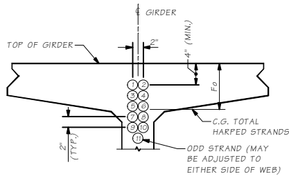
STRAND PATTERN AT GIRDER END
