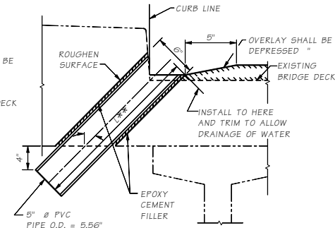
ELEVATION VIEW INCLINED DROP
