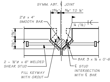
ALTERNATE 1
