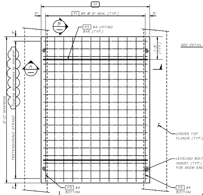
PLAN SIP DECK PANEL
