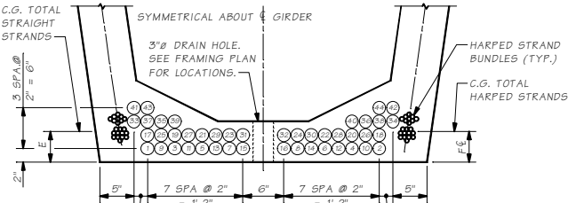
STRAND PATTERN AT SPAN STRAIGHT STRAND LOCATION SEQUENCE SHALL BE AS SHOWN (1), (2) ETC. 4 FOOT WIDE BOTTOM FLANGE SHOWN, OTHERS SIMILAR.
