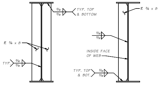
TYPICAL STIFFENER AT INTERMEDIATE X-FRAME
