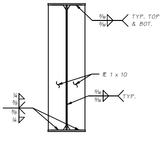
BEARING AND JACKING STIFFENERS
