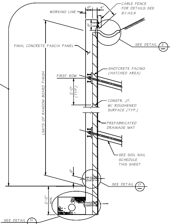
TYPICAL SECTION SOIL NAIL WALL
