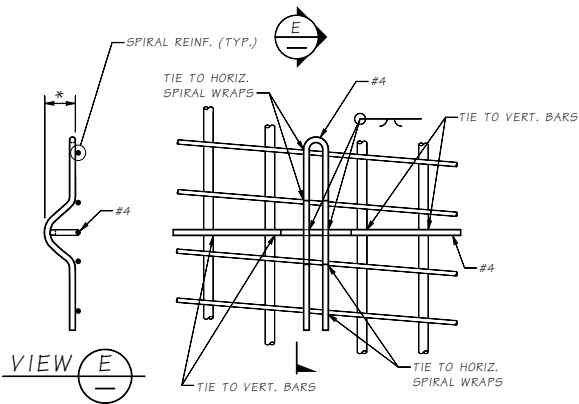
CENTRALIZER DETAIL EPOXY COAT CENTRALIZER OR PAINT WITH INORGANIC ZINC AFTER FABRICATION (OPTION 1)
