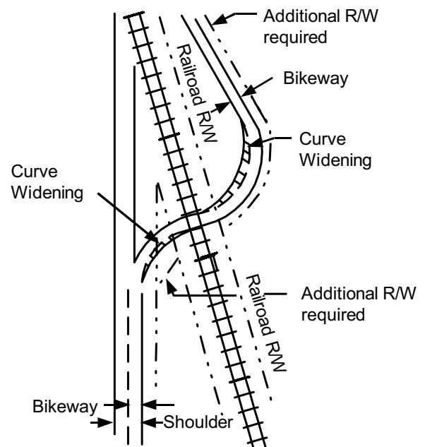
90° Crossing (most desirable)
