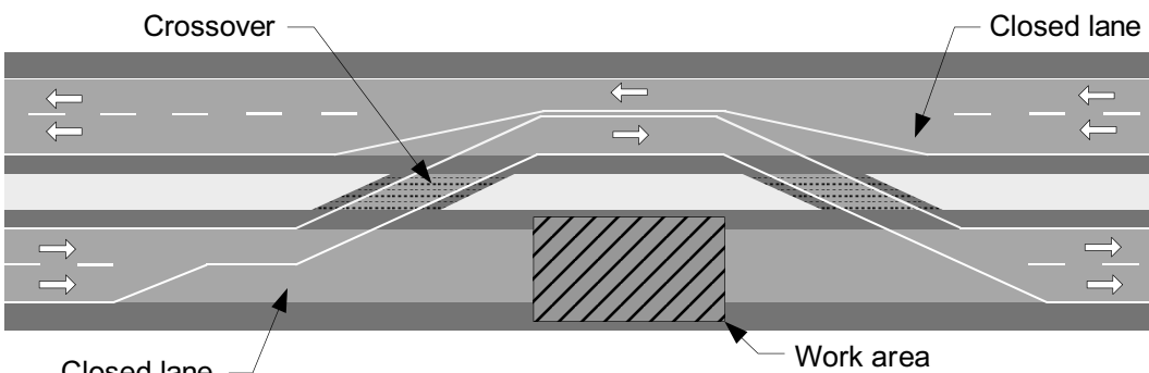
Crossover (with lane closures)
