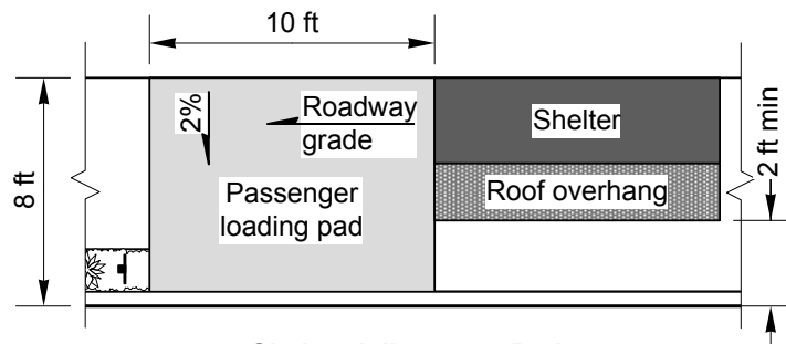
Shelter Adjacent to Pad
