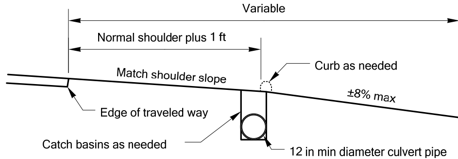
Profile Controls
