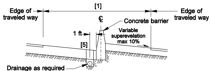
Alternate Design 1: Treatment on Curves
