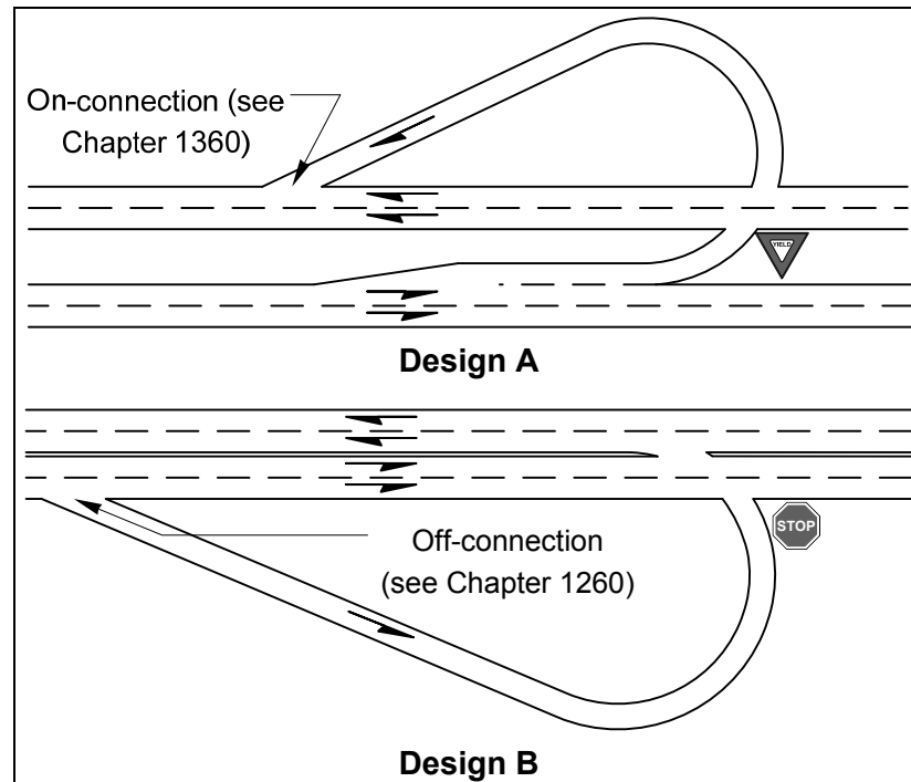
U-Turn Roadway Exhibit 1310-9
