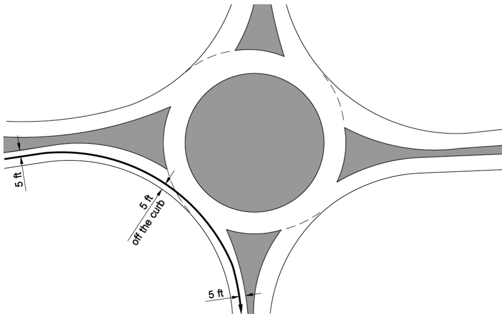
Right-Turn Movement
