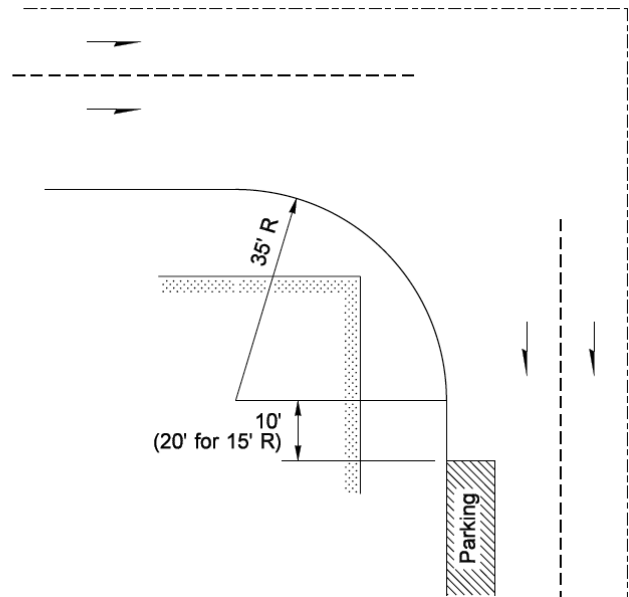
On-Street Parking After Turn
