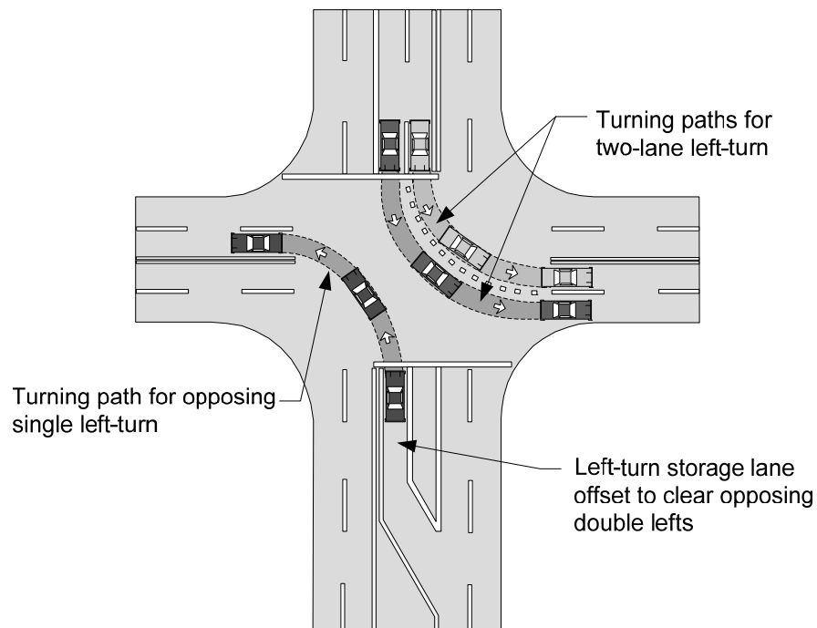
Left-Turn Lane Configuration With Concurrent Phasing
