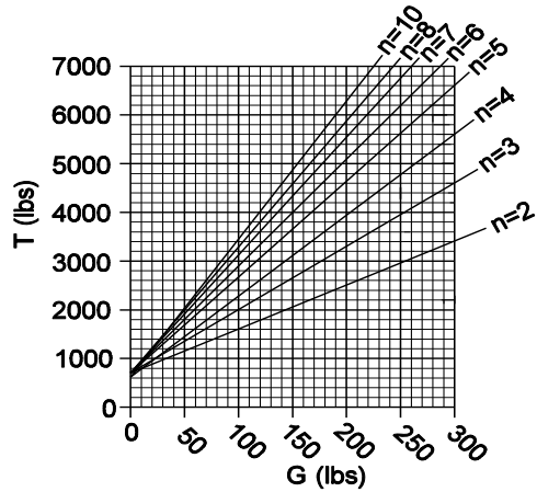
Chart 1 - Span Length 90' and Less
