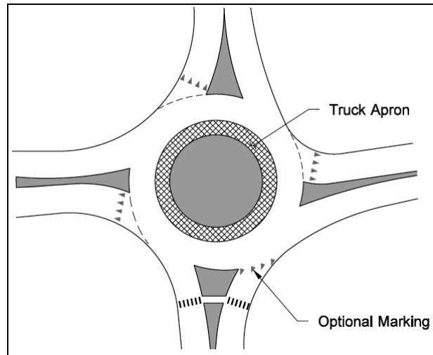
Single-Lane Roundabout Exhibit 1320-5
