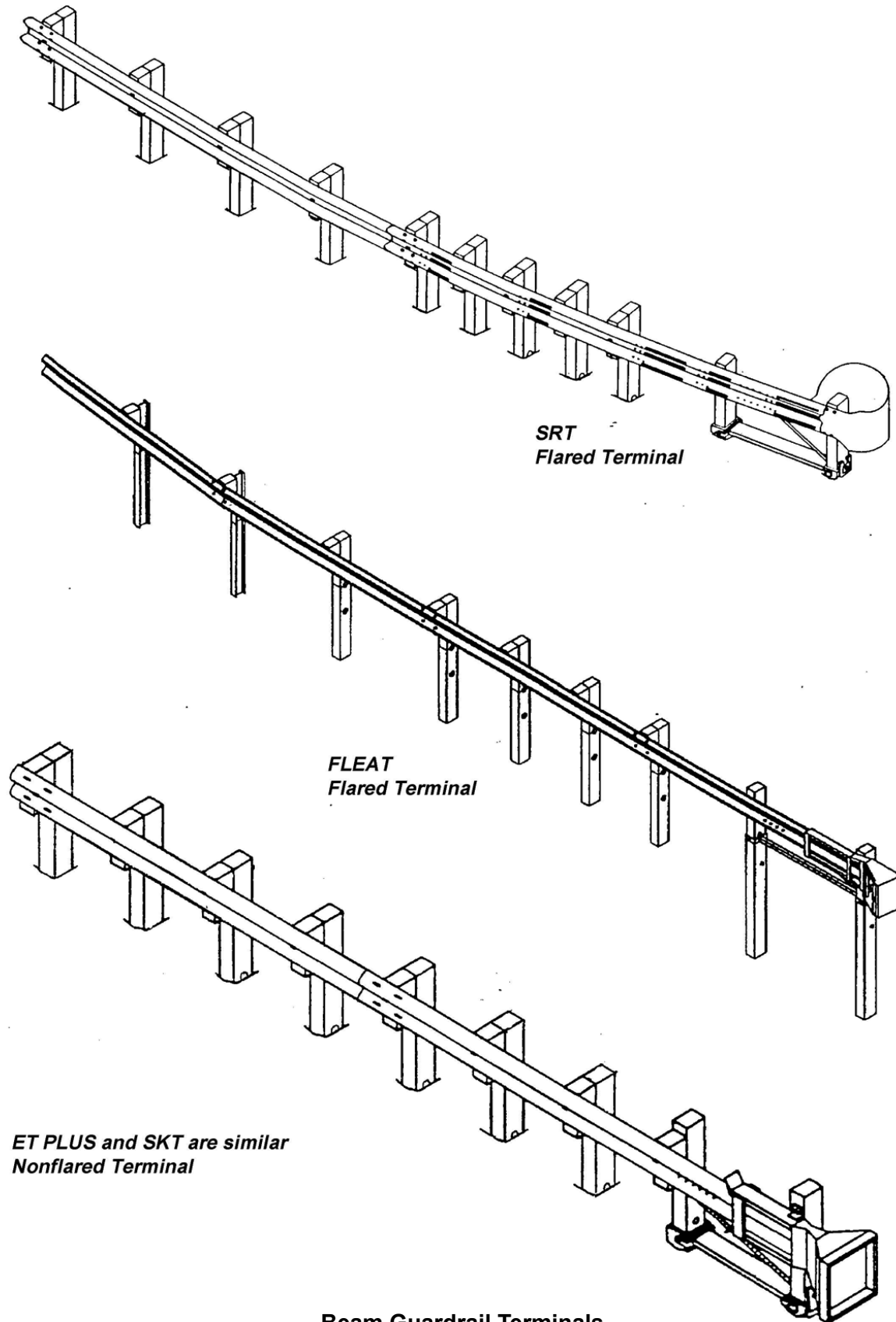
Beam Guardrail Terminals Exhibit 1610-13b
