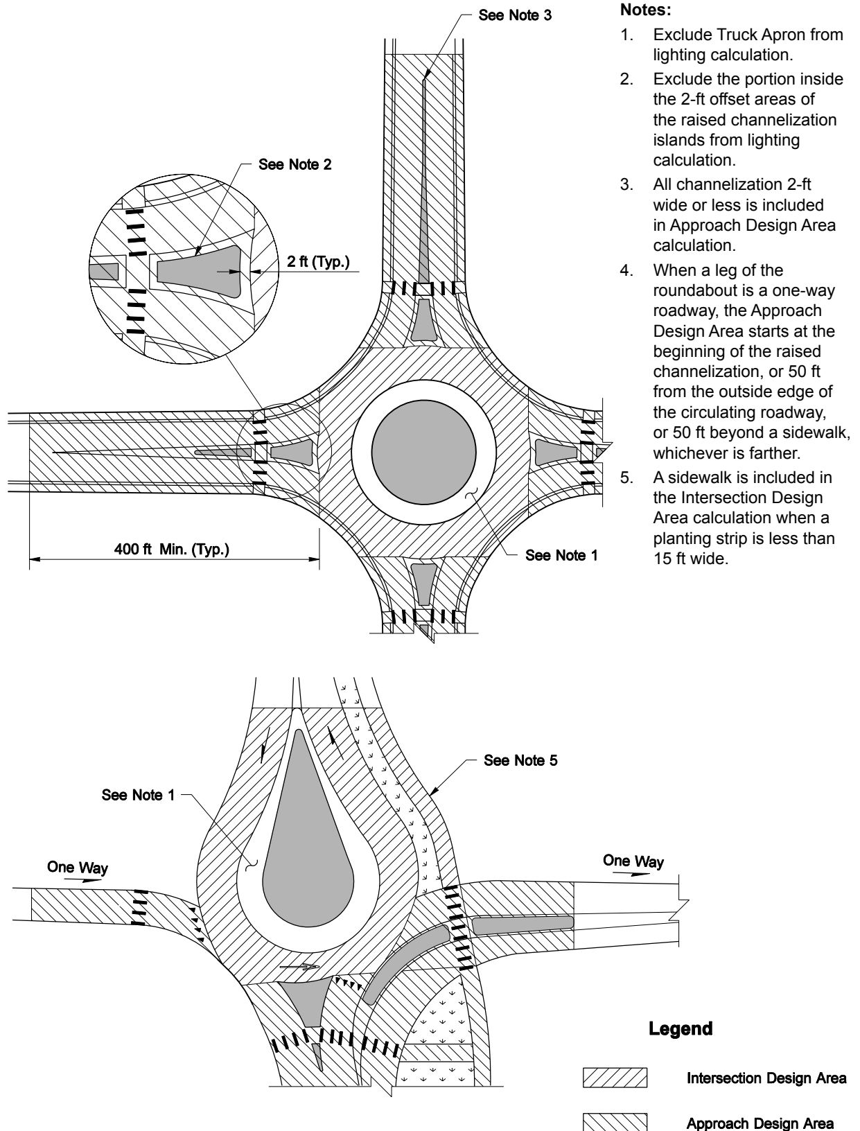
Roundabout Exhibit 1040-12
