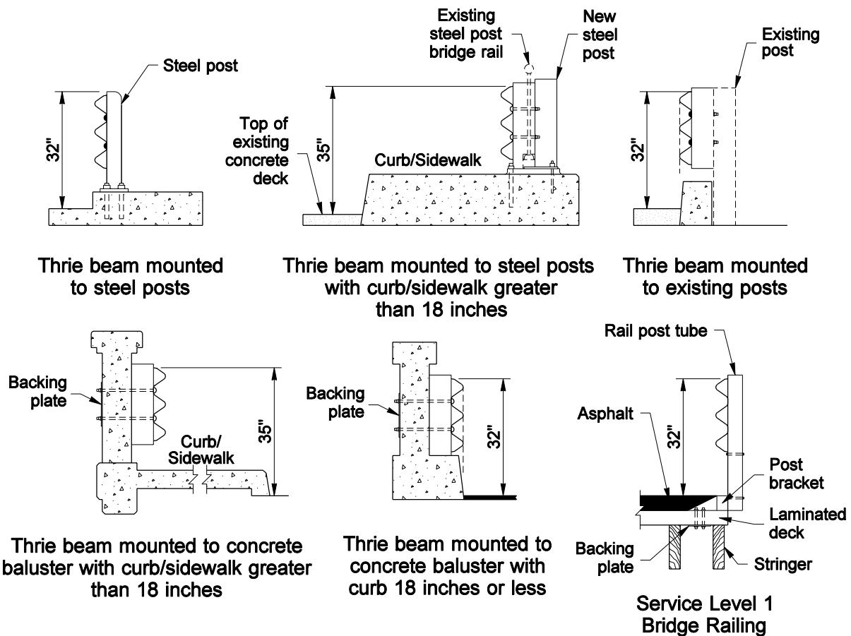
Thrie Beam Rail Retrofit Criteria Exhibit 1610-15
