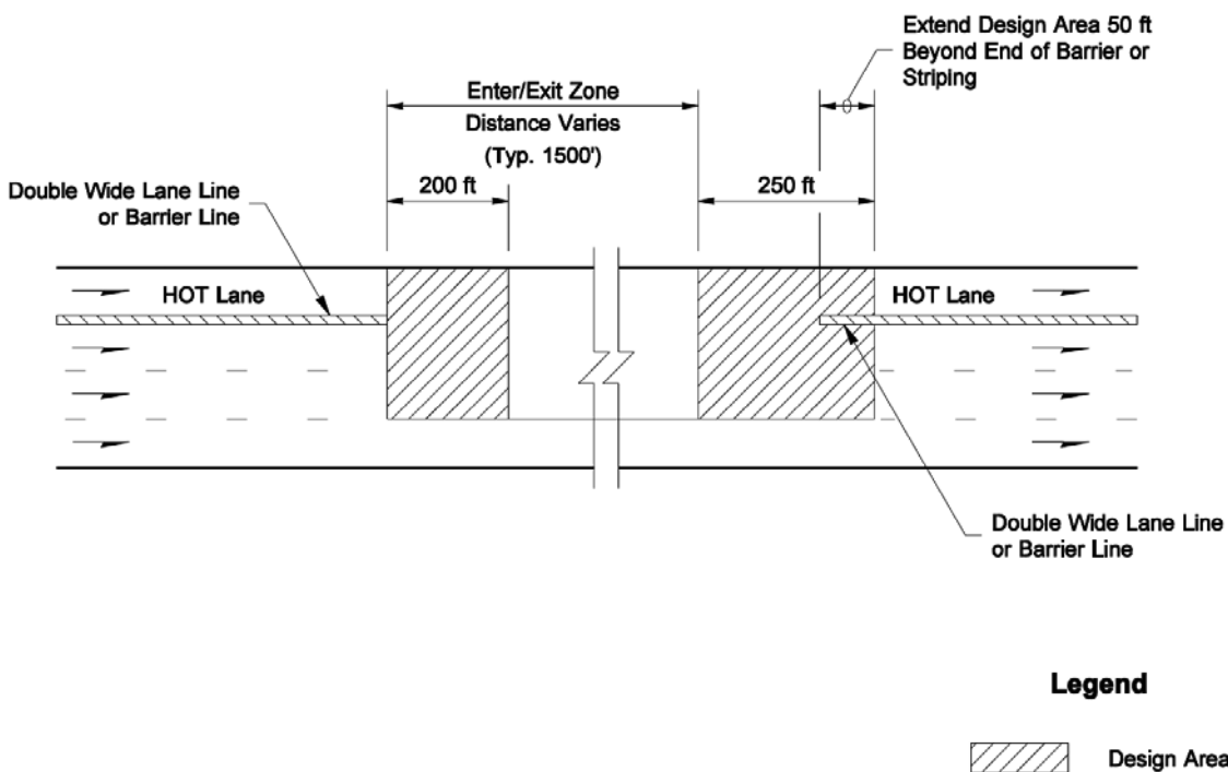
HOT (High-Occupancy Toll) Lane Enter/Exit Zone Exhibit 1040-5
