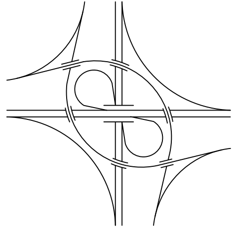
Semidirectional
