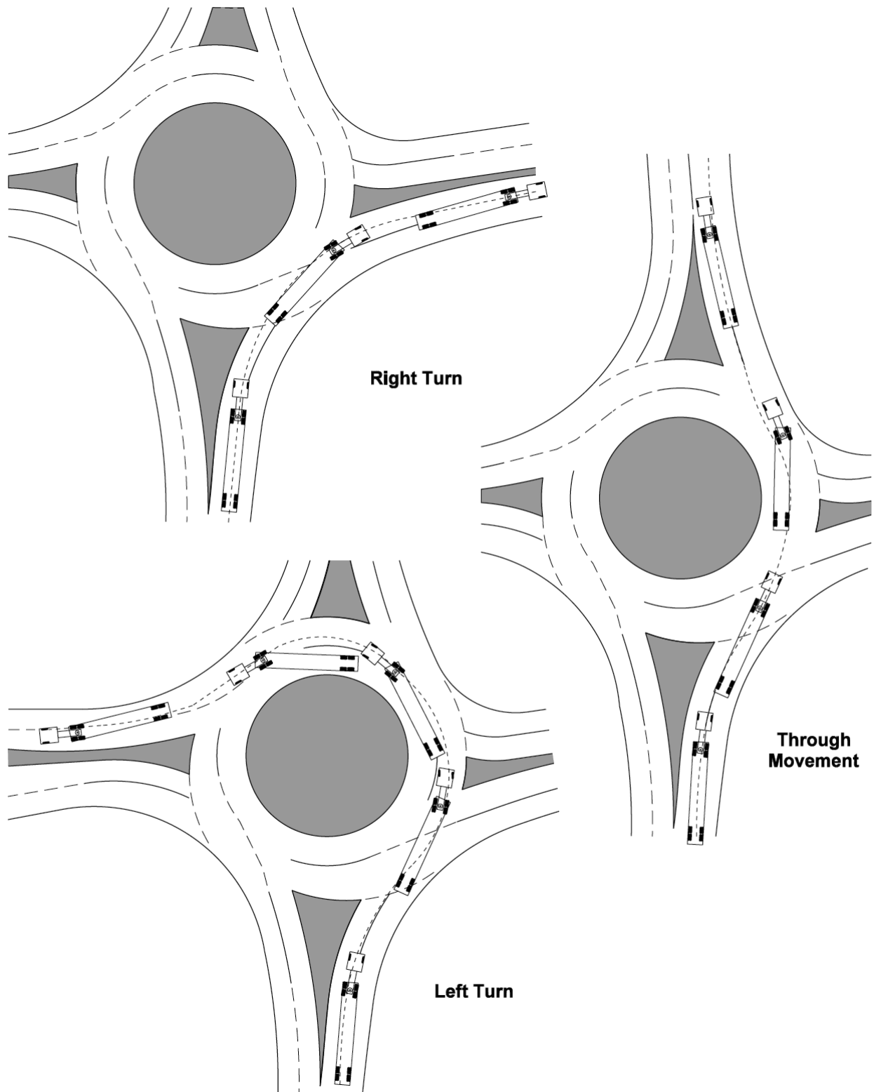
Truck Turning Paths Exhibit 1320-14b
