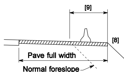
Shoulder Widening for Barrier
