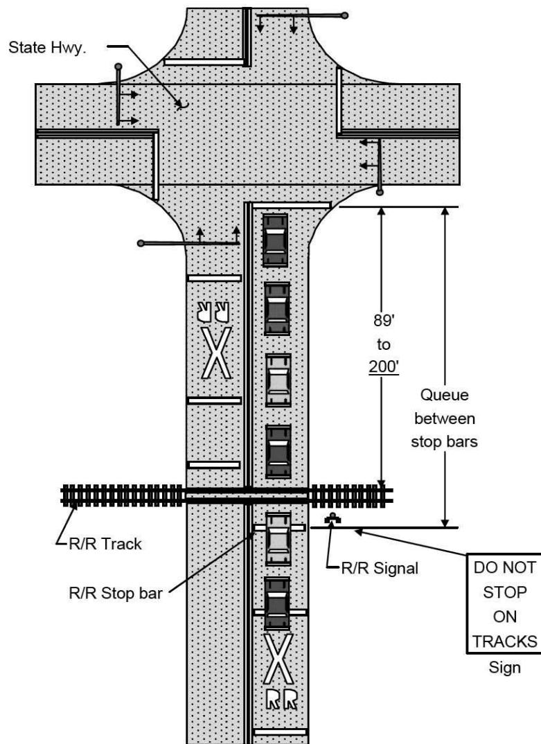
Railroad Crossing more than 88 feet from Intersection
