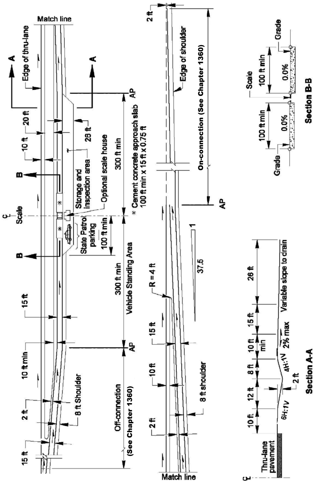
Truck Weigh Site: Multilane Highways Exhibit 1720-1
