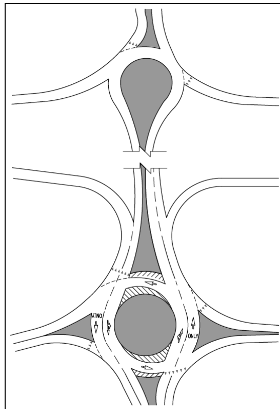
Teardrop Roundabout With Ramps Exhibit 1320-7c
