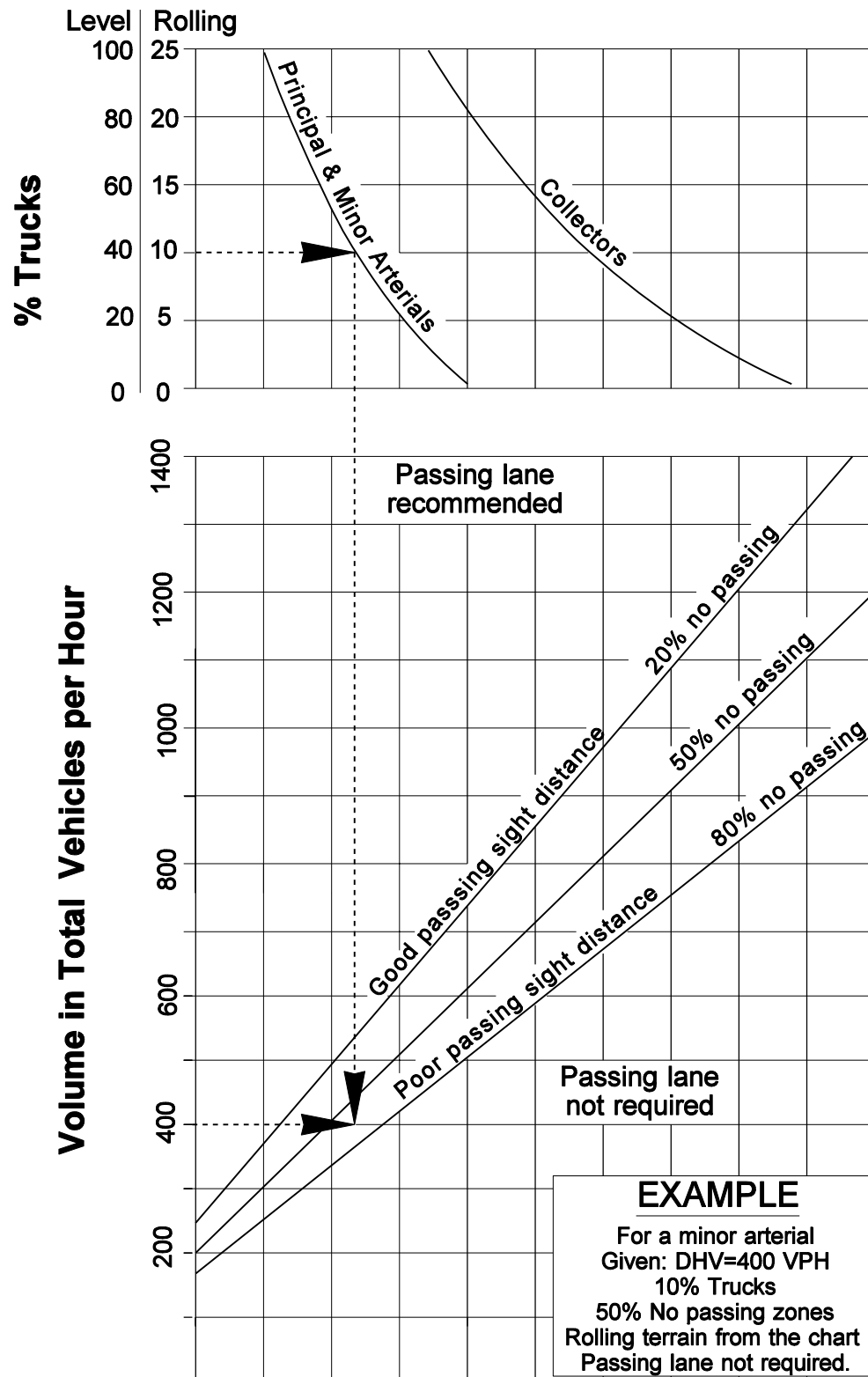
Warrant for Passing Lanes Exhibit 1270-5
