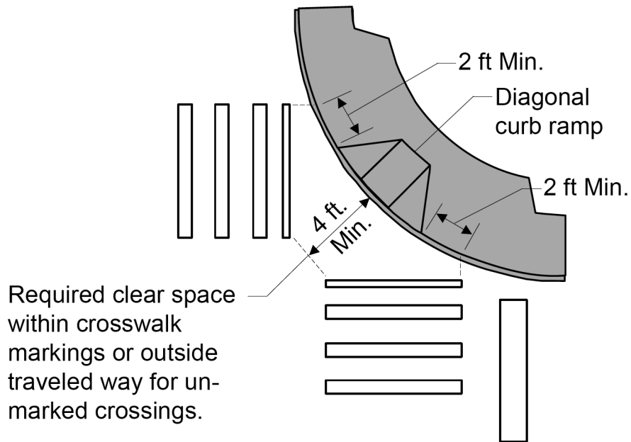
Clear Space for Diagonal Ramp
