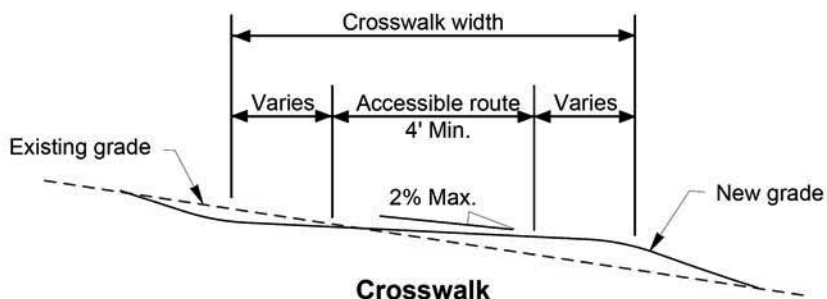
Marked Crosswalk
