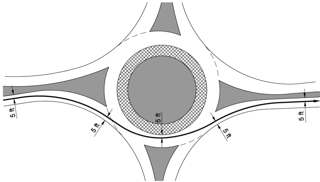
Single-Lane Roundabout
