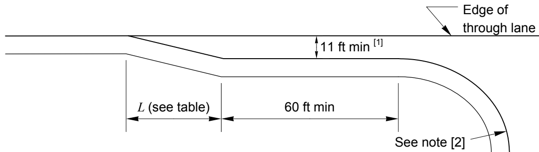
Right-Turn Pocket
