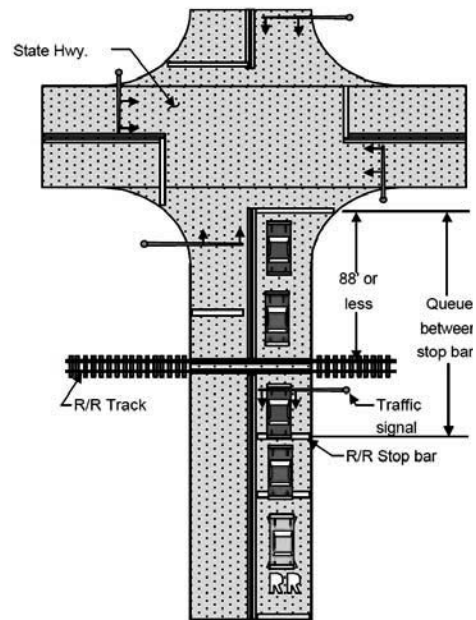
Railroad Crossing With High Exposure Factor
