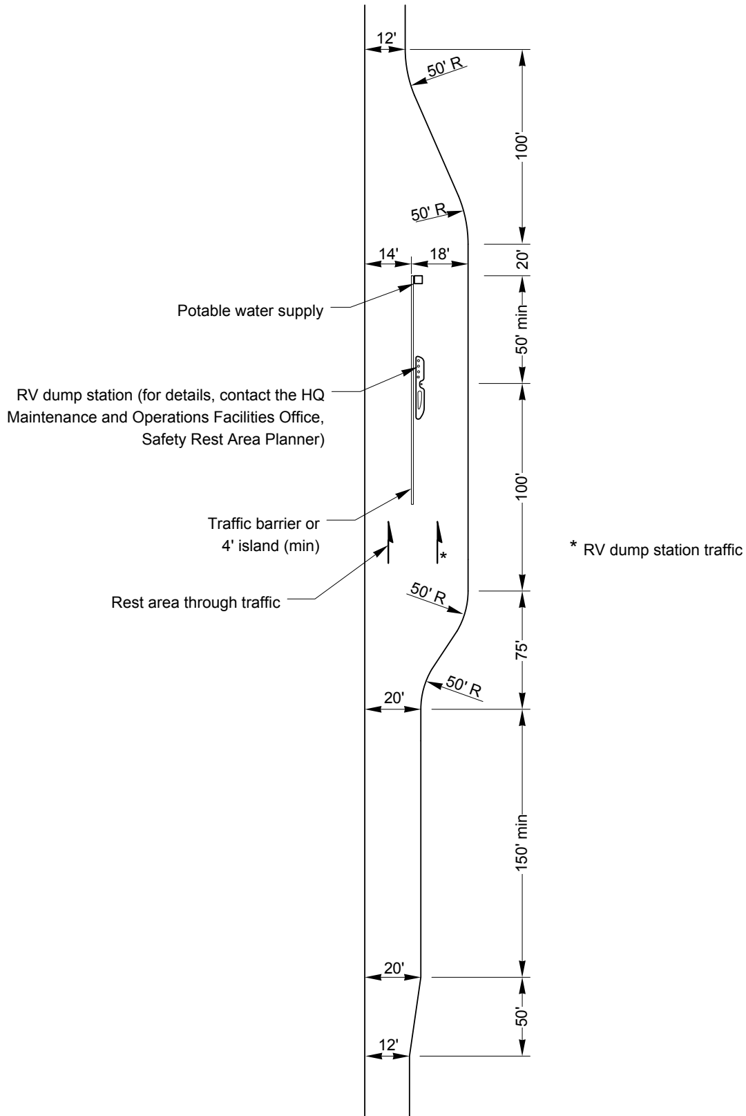
Typical Single RV Dump Station Layout Exhibit 1710-2
