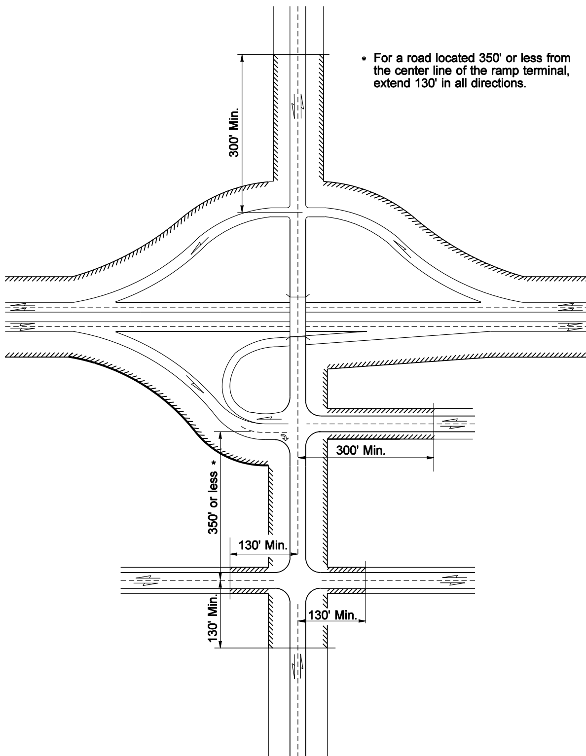
Full Access Control Limits: Interchange Exhibit 530-1b
