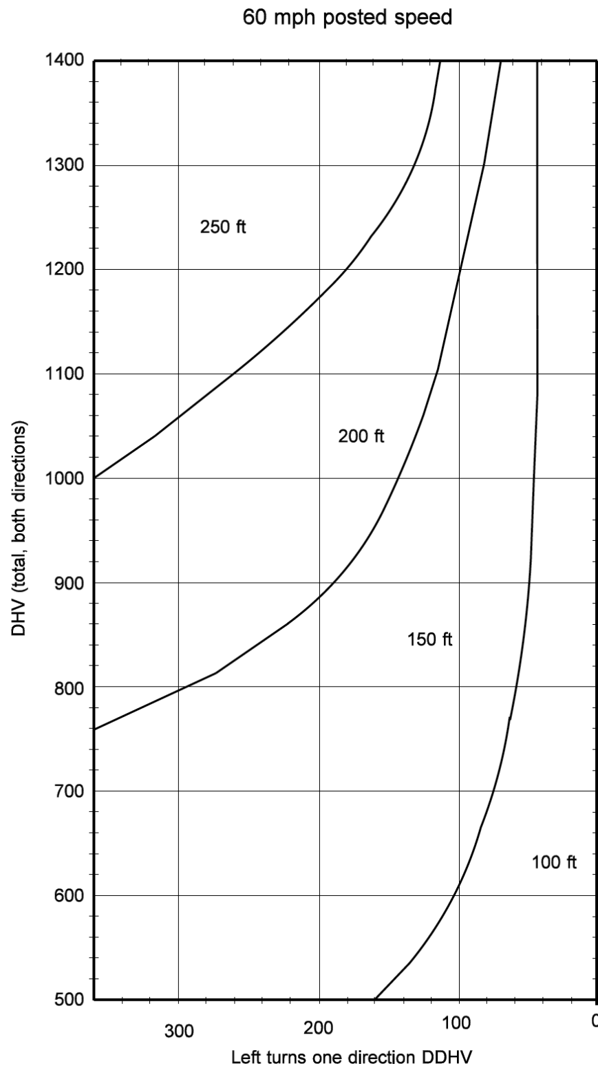
Left-Turn Storage Length: Two-Lane, Unsignalized Exhibit 1310-13c
