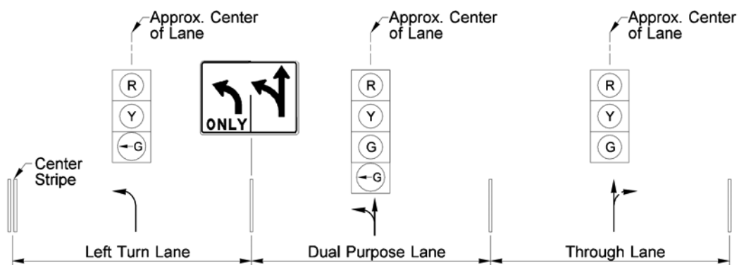
One Through Lane, a Dual Purpose (Left or Through) Lane and One Left Turn Storage Lane With Split Phasing for Protected Left Turns (Left turn and through movements terminate together.)
