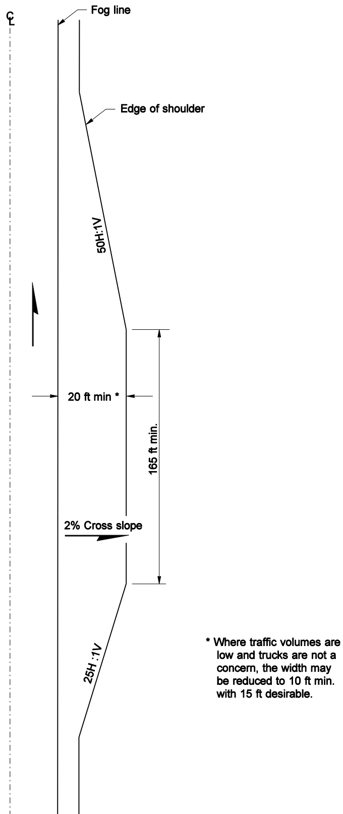
Chain Up/Chain Off Area Exhibit 1270-9
