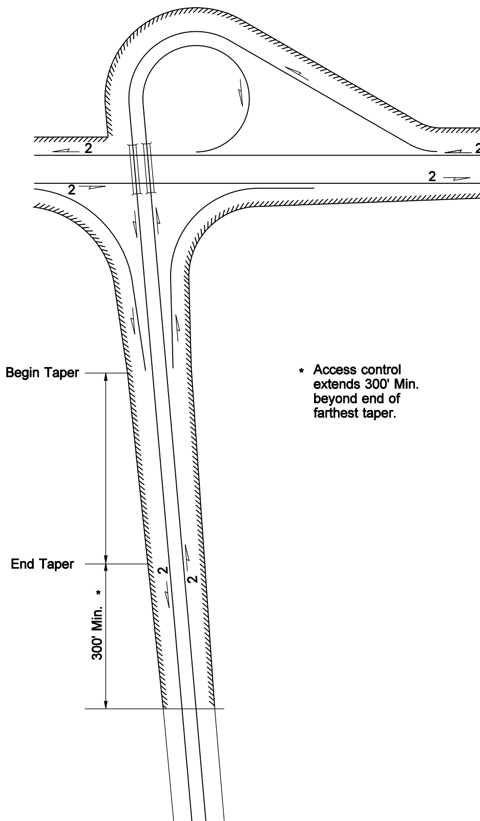
Full Access Control Limits: Ramp Terminal With Transition Taper Exhibit 530-1d
