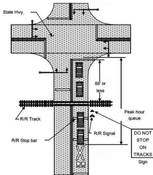
Railroad Crossing With Low Exposure Factor
