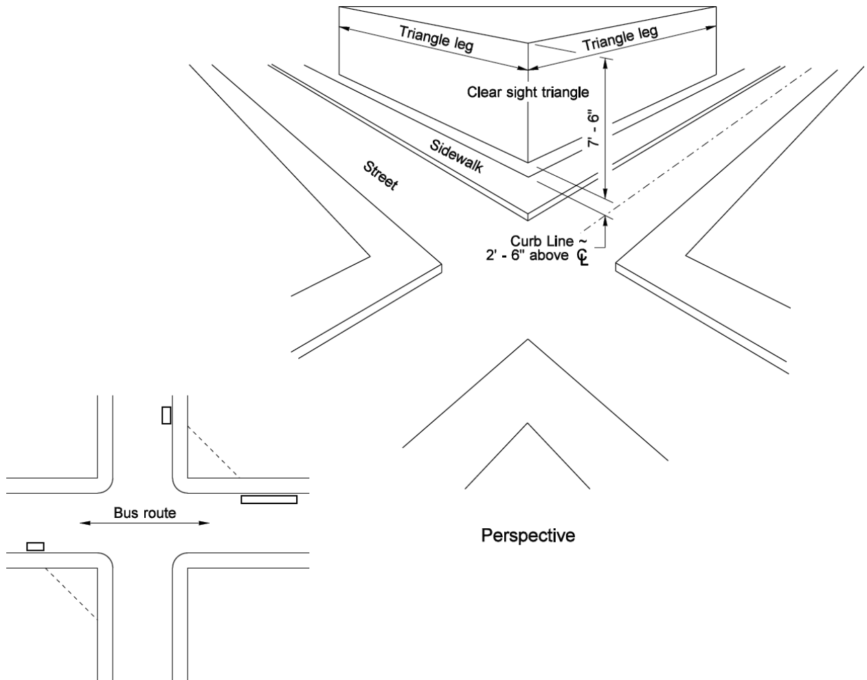
Shelter Siting Exhibit 1430-8
