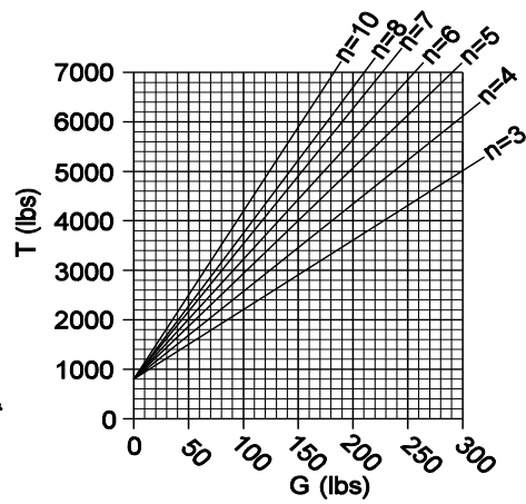
Chart 2 - Span Length 91' to 120'
