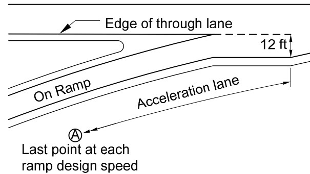
Parallel On-Connection
