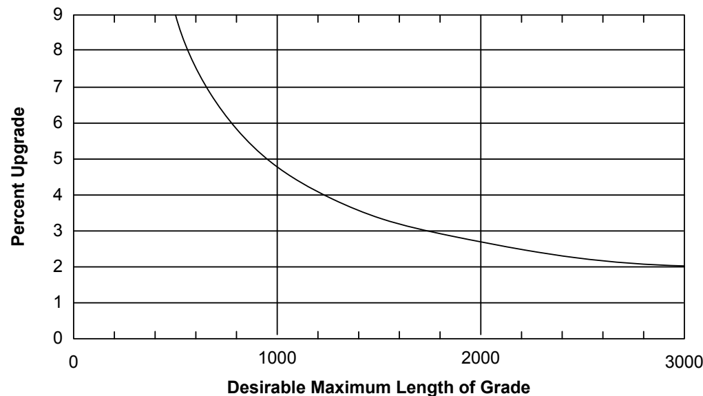
Grade Length Exhibit 1220-1
