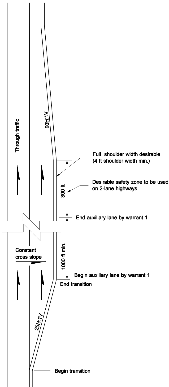
Auxiliary Climbing Lane Exhibit 1270-4
