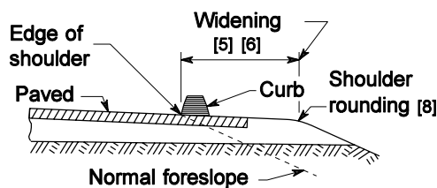
Asphalt Concrete Curb Placement
