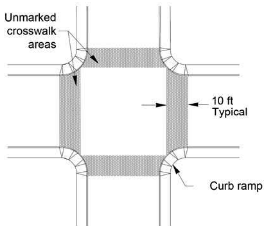
Unmarked Crosswalks
