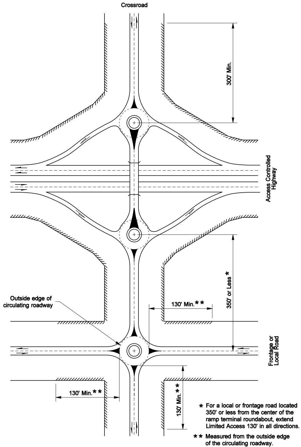
Full Access Control Limits: Interchange With Roundabouts Exhibit 530-1c
