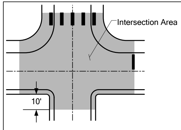
Intersection Area Exhibit 1310-1
