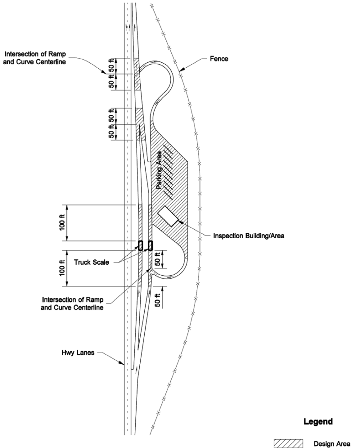
Truck Weigh Site Exhibit 1040-18
