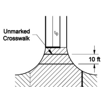
Unmarked Crosswalk Detail
