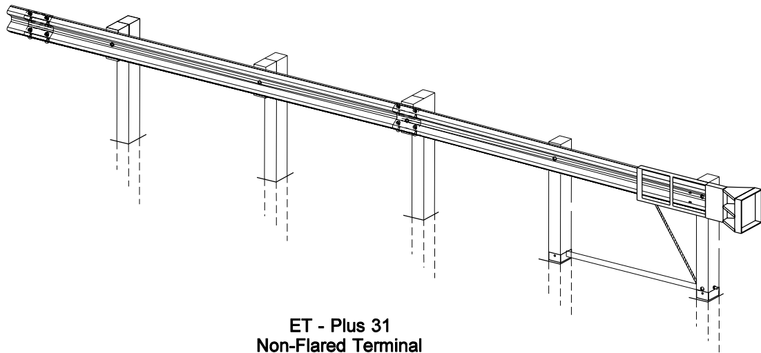
SKT - MGS Non-Flared Terminal
