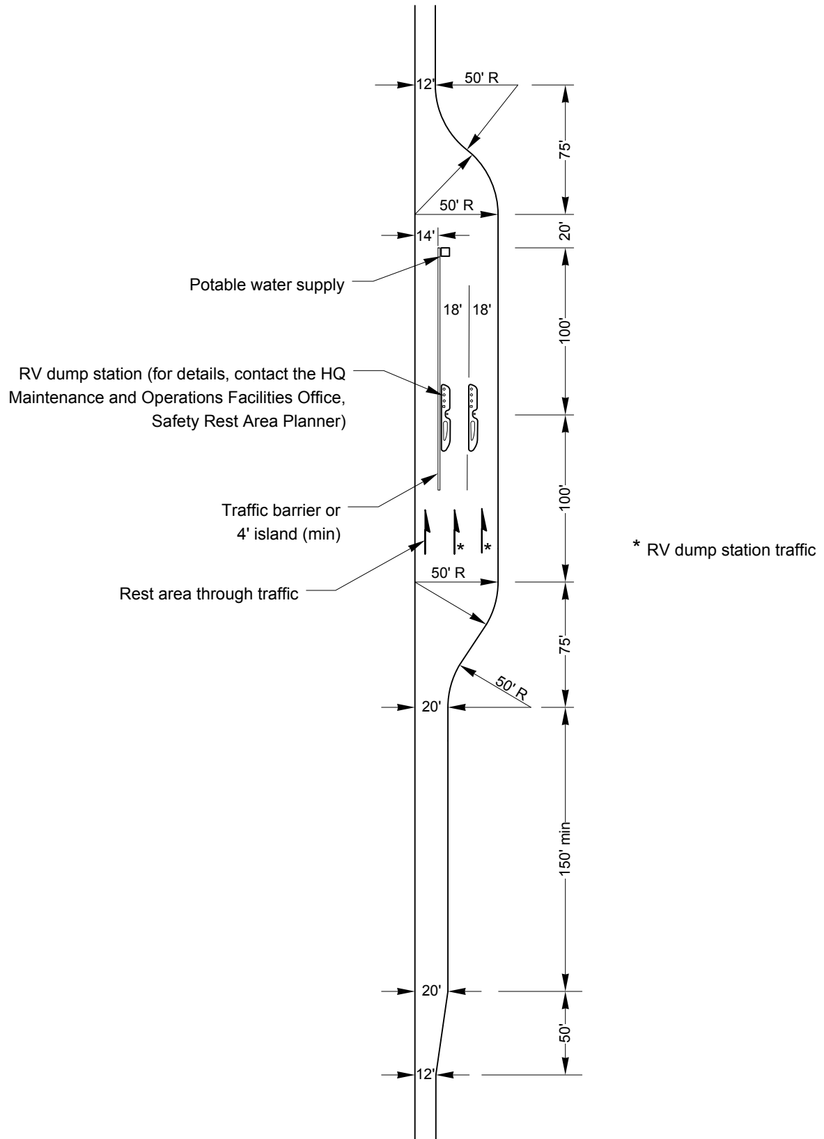
Typical Two RV Dump Station Layout Exhibit 1710-3
