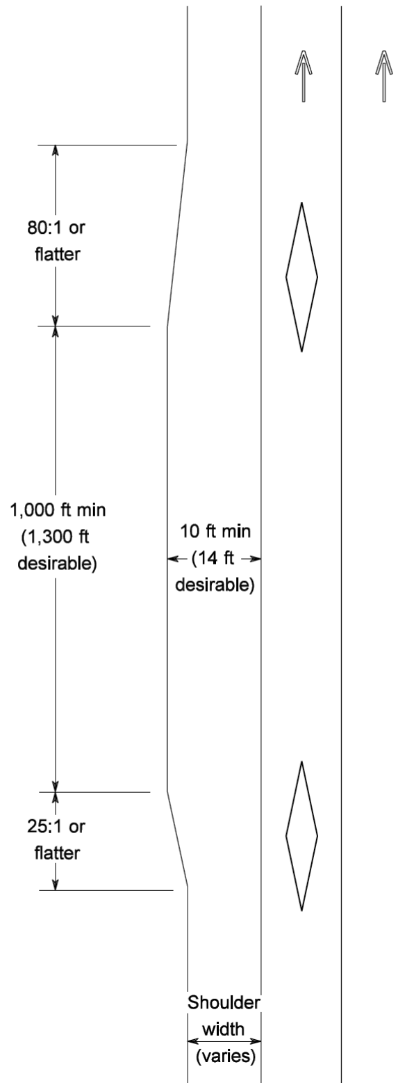
Enforcement Area: One Direction Only Exhibit 1410-5a
