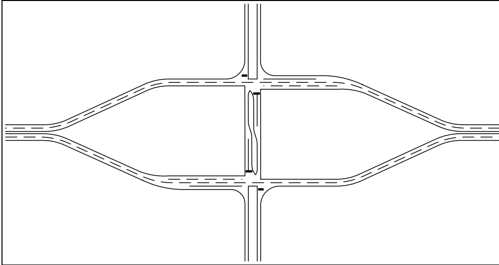
Split Intersections Exhibit 1310-4
