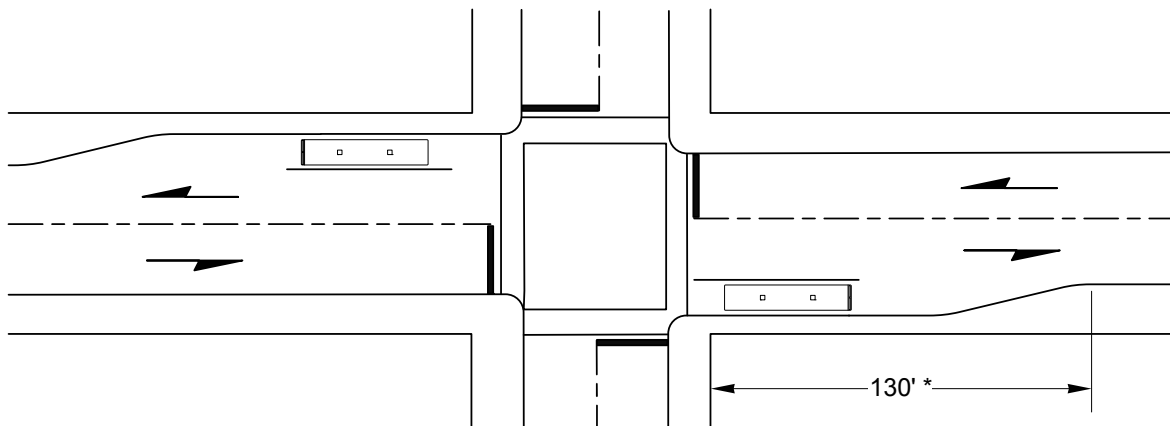
Far-Side Bus Pullout After Right Turn
