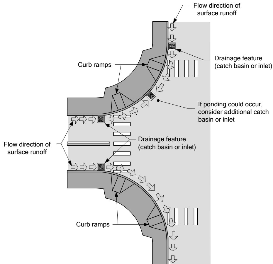
Curb Ramp Drainage Exhibit 1510-9
