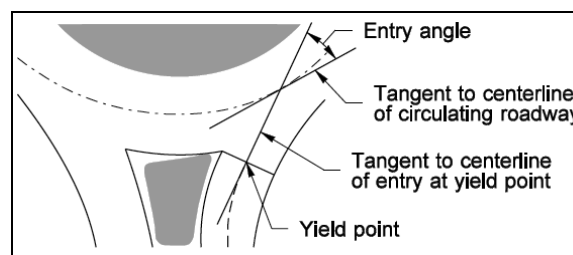
Entry Angle Exhibit 1320-2
