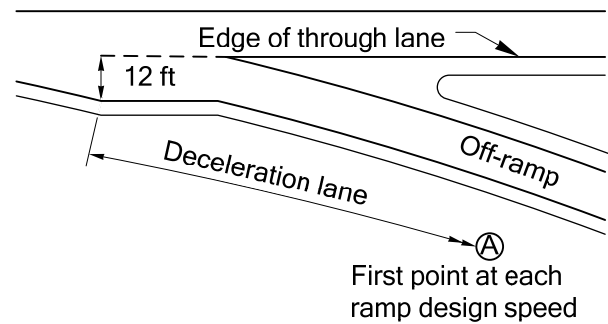
Parallel Off-Connection
