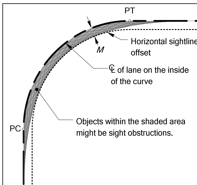
Sight Distance Area on Horizontal Curves
