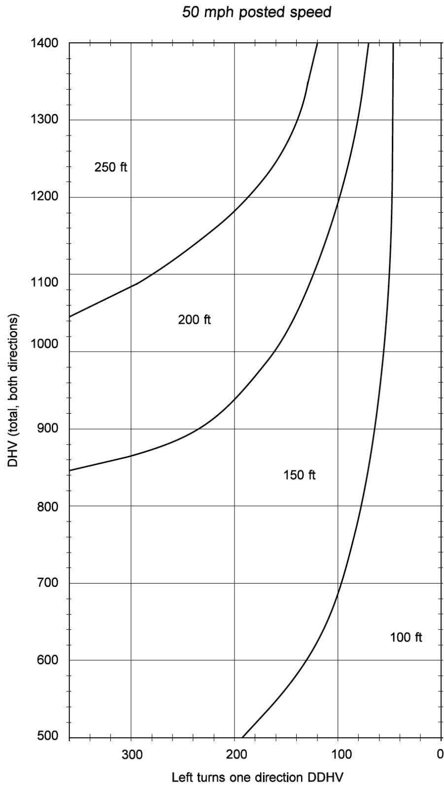
Left-Turn Storage Length: Two-Lane, Unsignalized Exhibit 1310-13b
