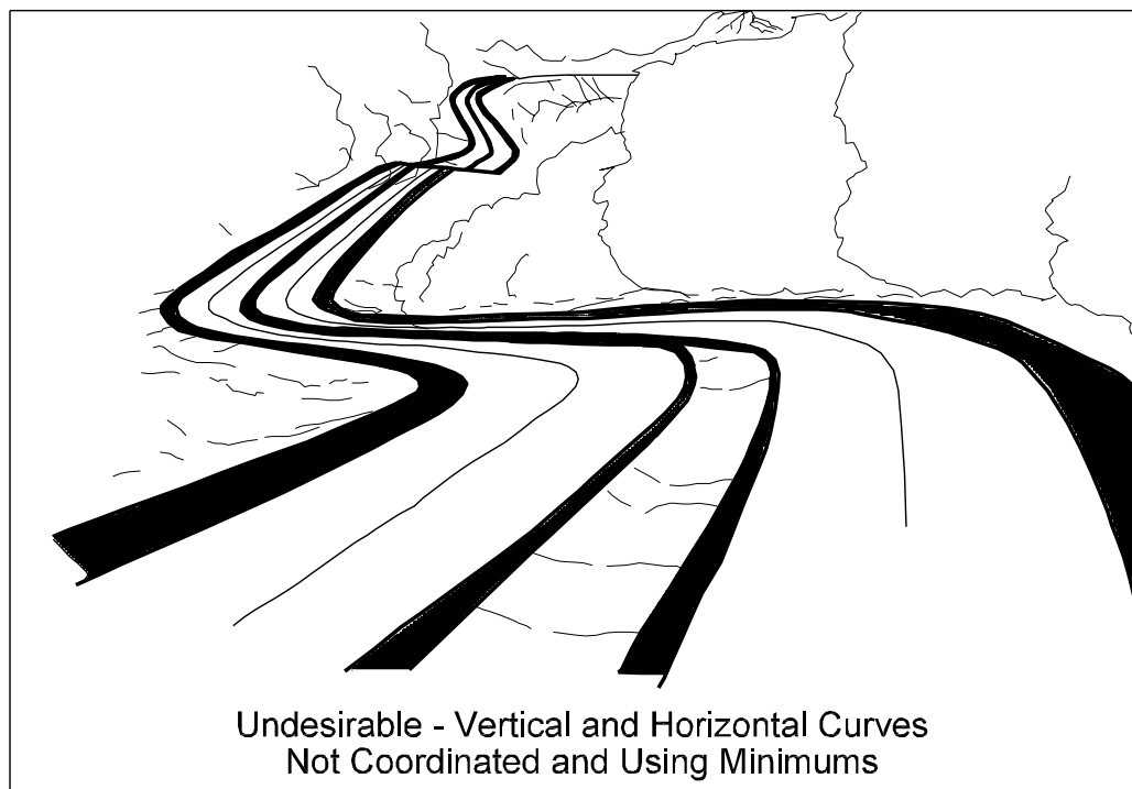
Coordination of Horizontal and Vertical Alignments Exhibit 1220-2c
