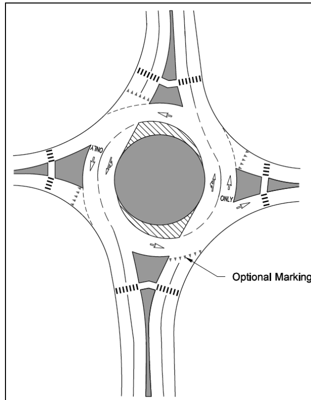
Multilane Roundabout Exhibit 1320-6a
