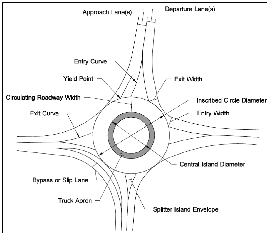
Roundabout Elements
