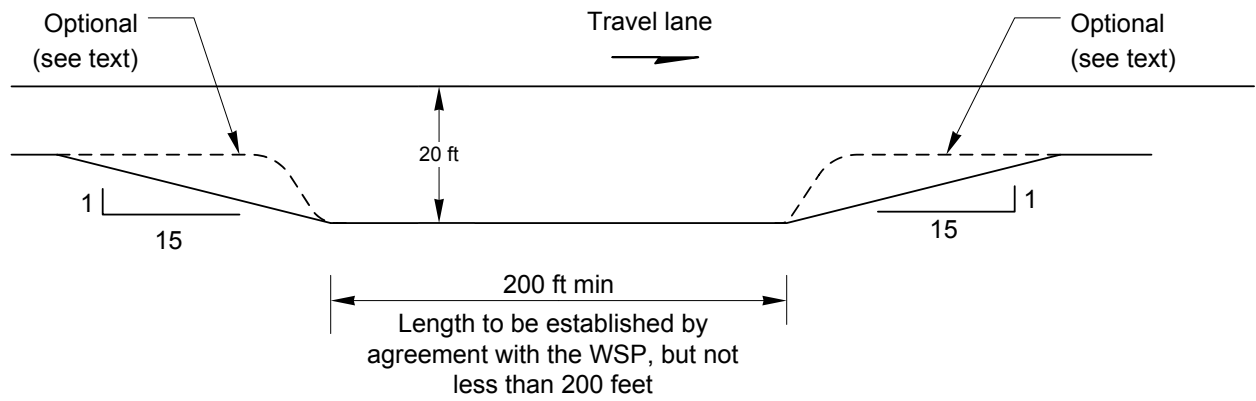
Small Shoulder Site Exhibit 1720-6
