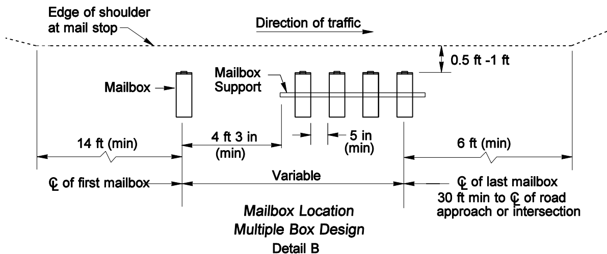
Mailbox Location and Turnout Design Exhibit 1600-6
