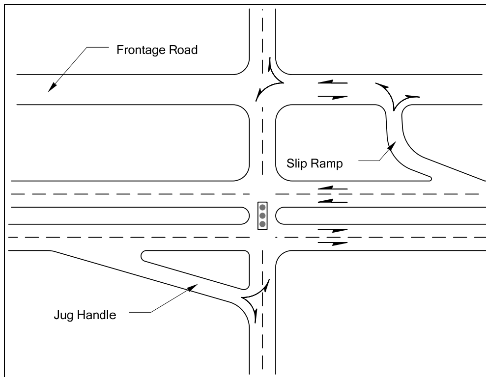
Exhibit 1310-2a
