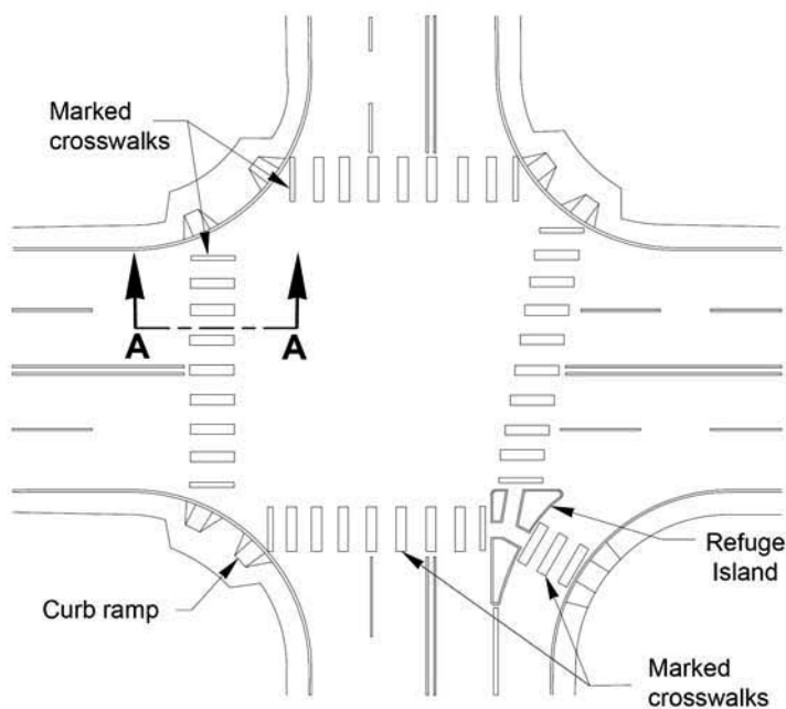
Marked Crosswalk
