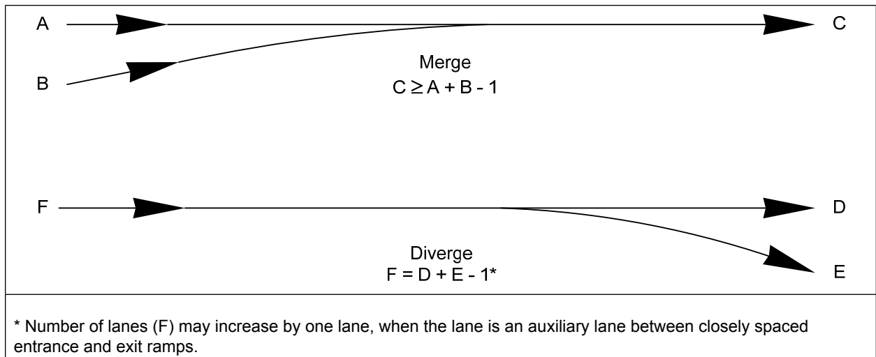
Lane Balance Exhibit 1360-7a
