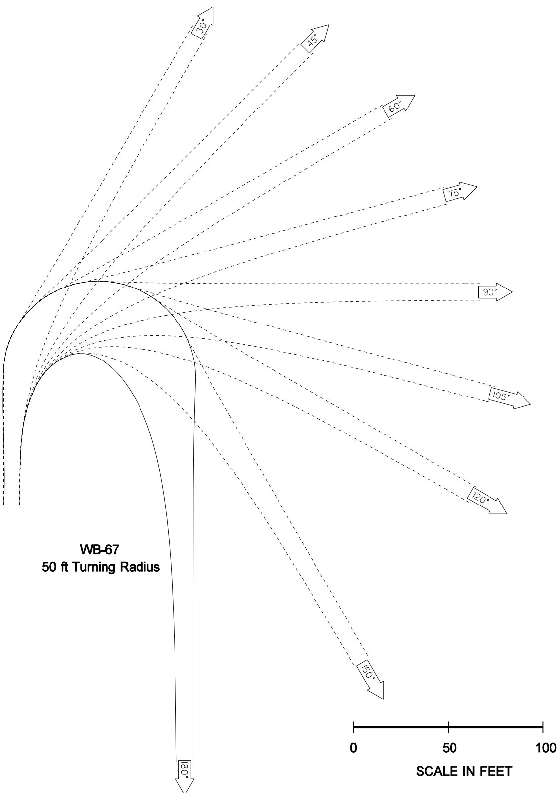
Turning Path Template Exhibit 1310-20c
