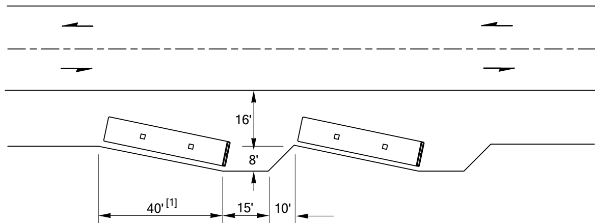
Sawtooth Design [2]
