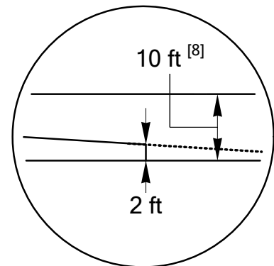
Paving Detail
