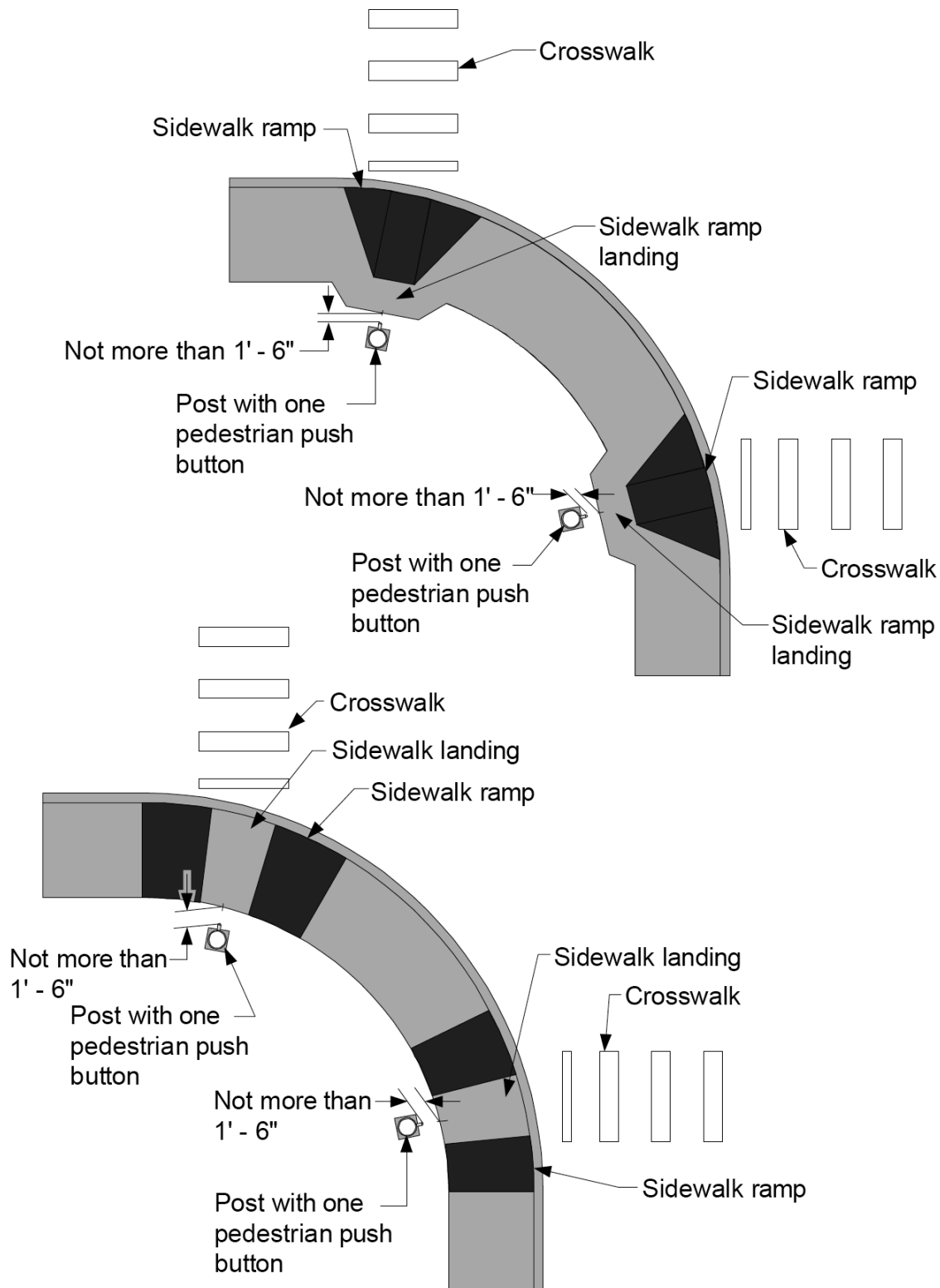
Pedestrian Push Button Locations Exhibit 1330-8b
