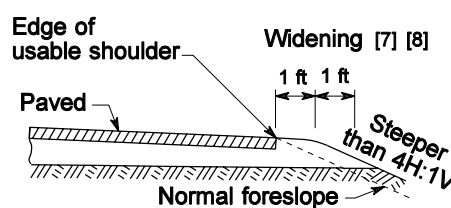
Shoulder Rounding [2]
