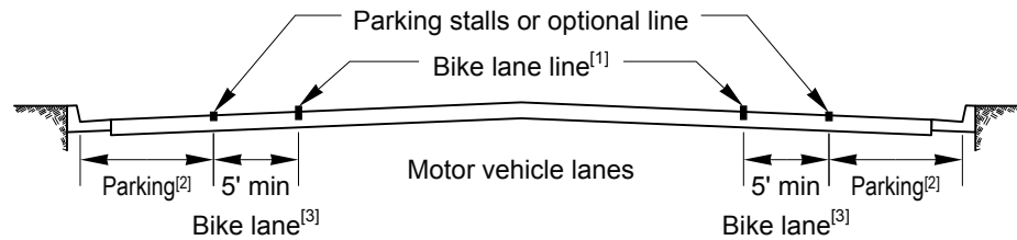
Design A: Marked Parking
