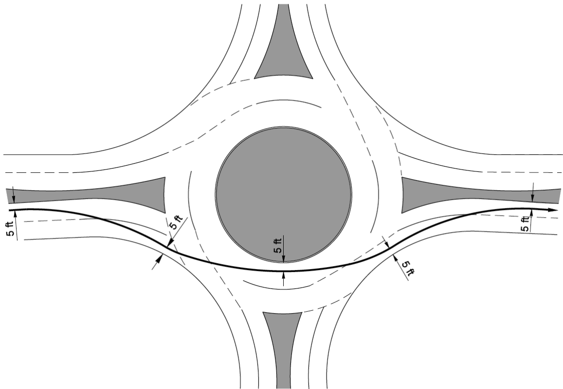
Multilane Roundabout
