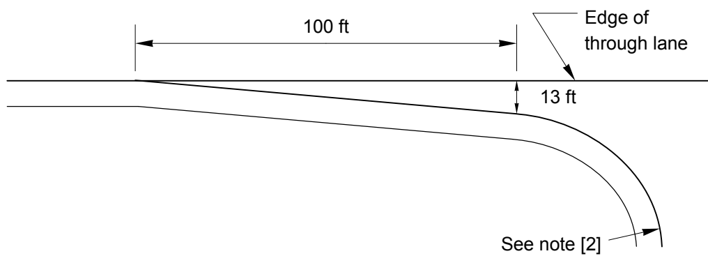
Right-Turn Taper
