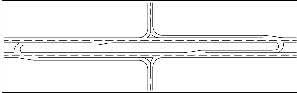
Indirect Left Turns: Unsignalized Intersections Exhibit 1310-2b
