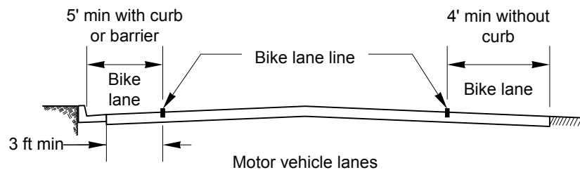
Design C: Parking Prohibited
