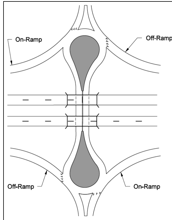
Double Teardrop Exhibit 1320-7b
