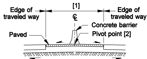
Design A: Crowned Median
