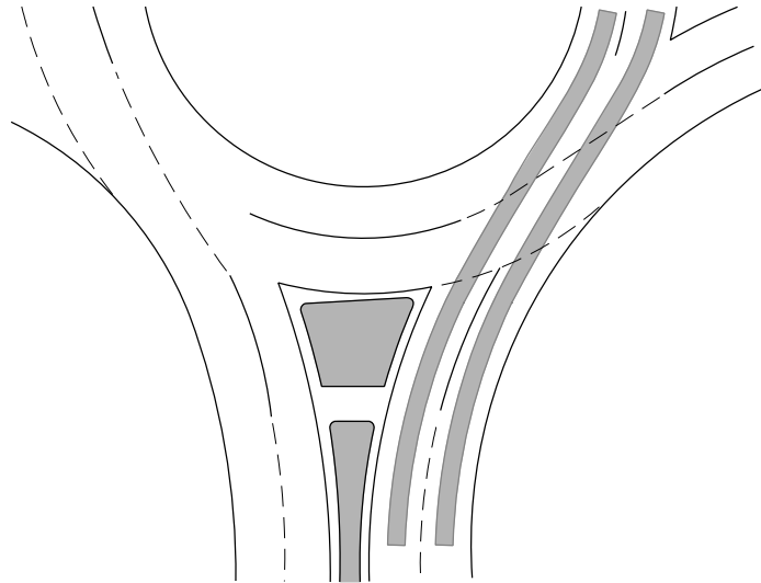
Entry Design Without Path Overlap (Desirable)
