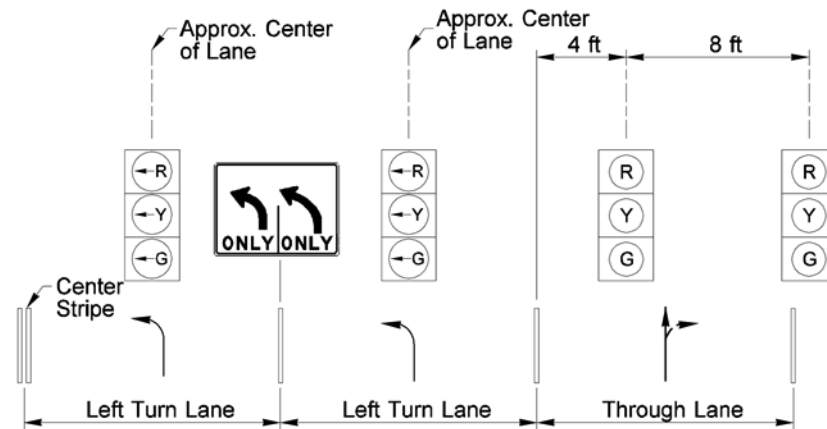
One Through Lane and Two Left Turn Storage Lanes With Protected Left Turn Phasing
