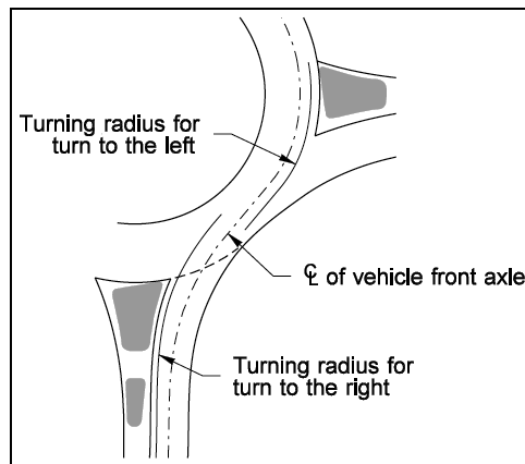
Turning Radius (R) Exhibit 1320-3
