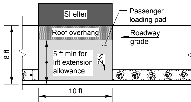
Shelter Behind Pad
