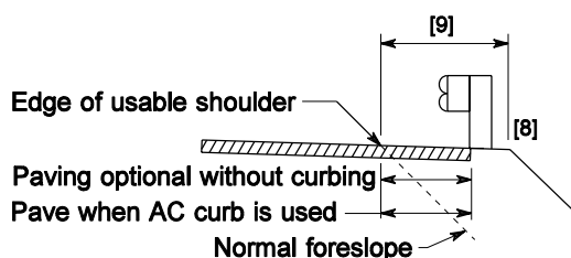
Shoulder Widening for Guardrail
