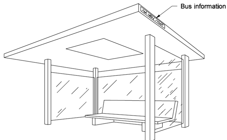
Typical Bus Shelter Design Exhibit 1430-9
