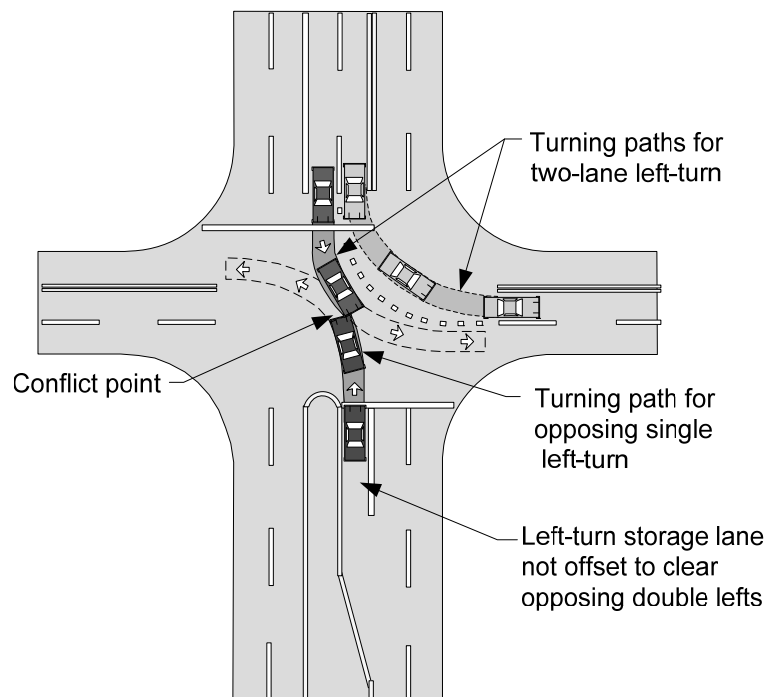
Left-Turn Lane Configuration Preventing Concurrent Phasing
