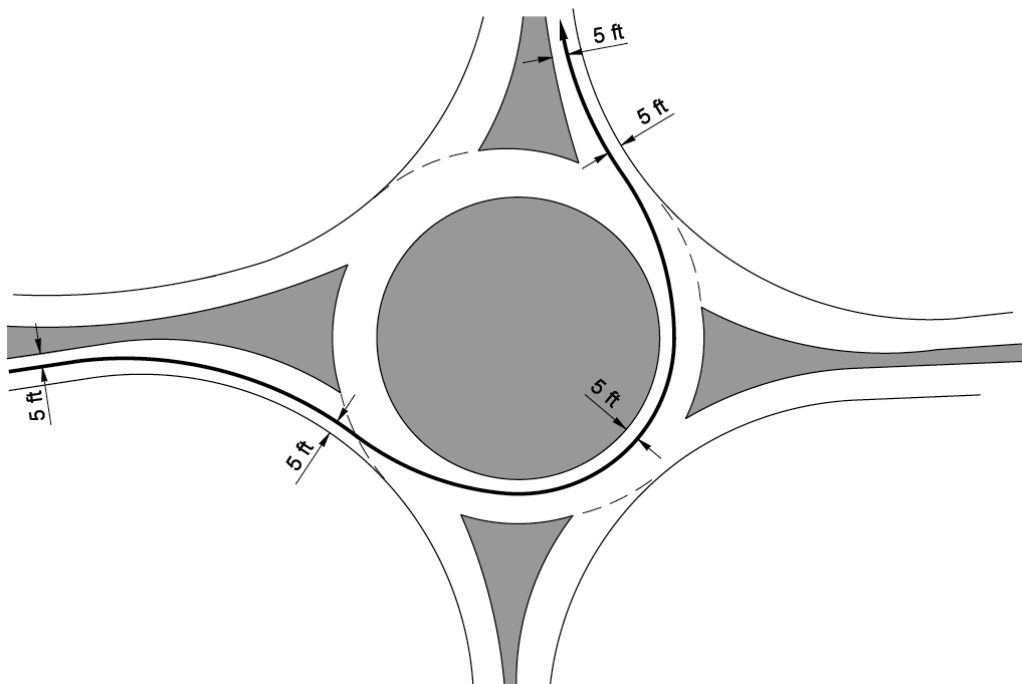
Left-Turn Movement
