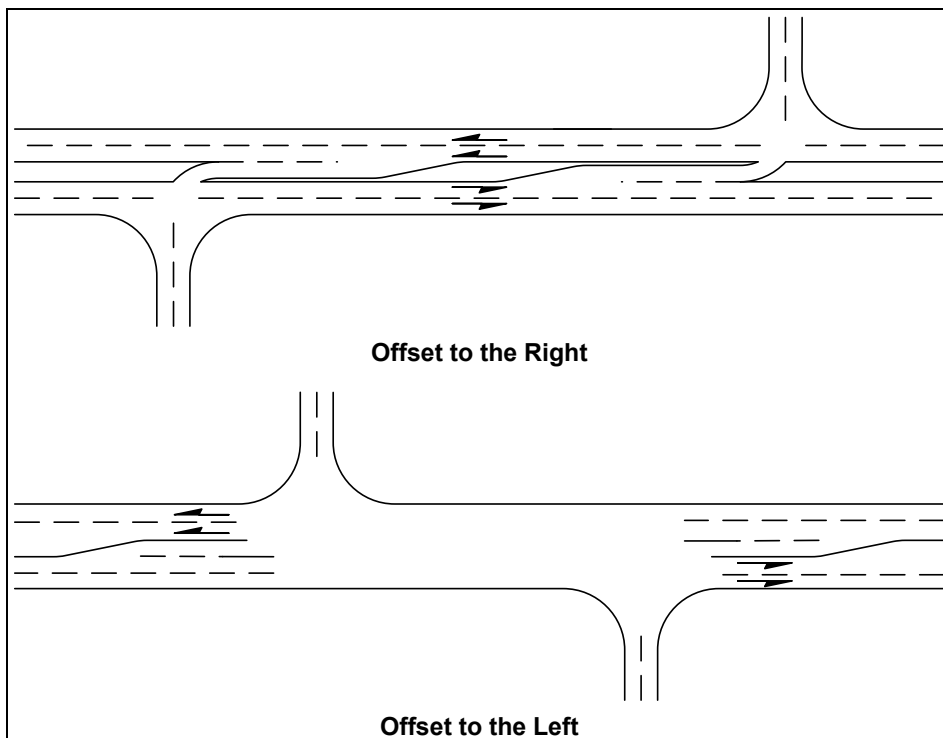
Split Tee Intersections Exhibit 1310-3
