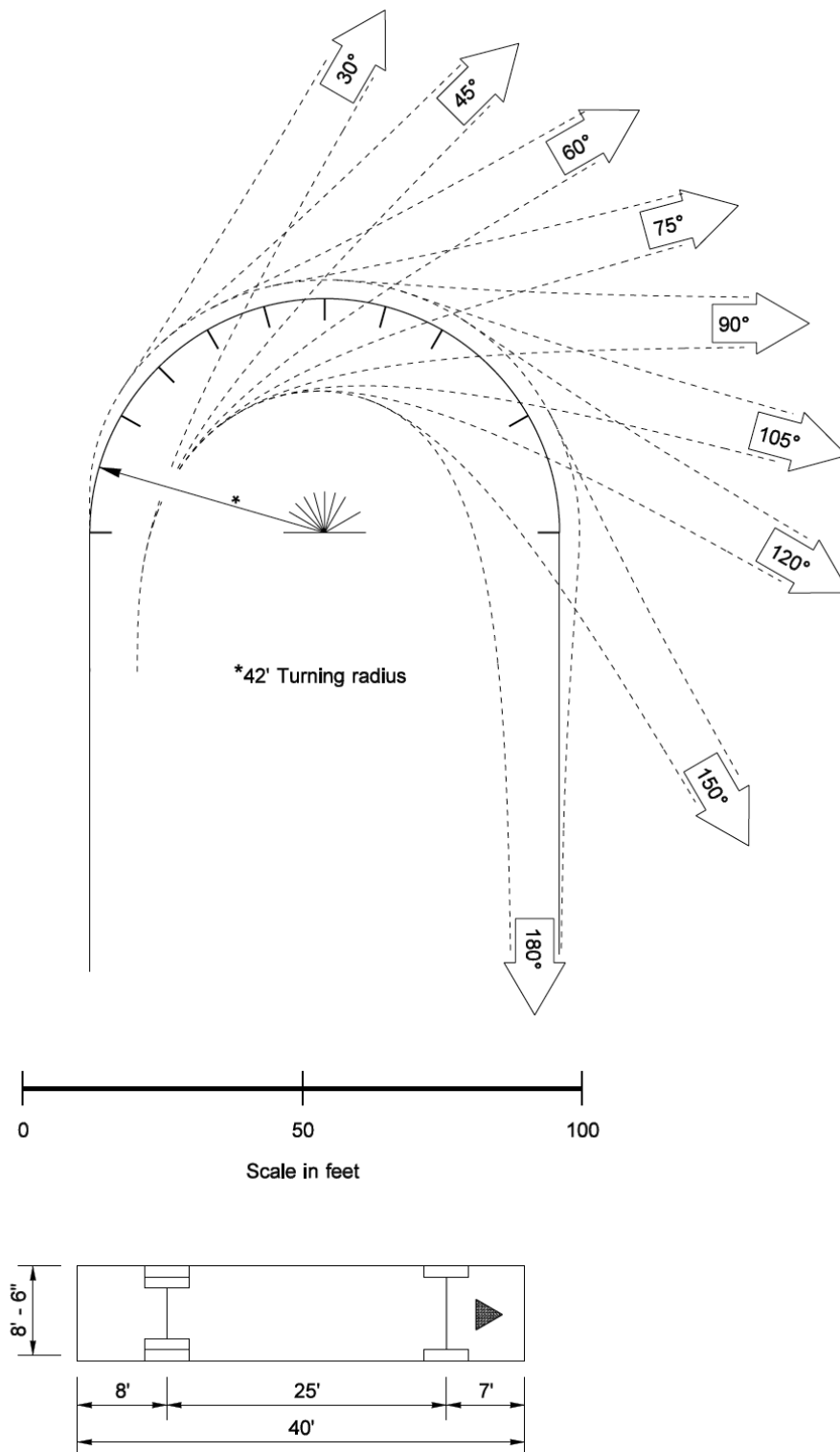
Turning Template for a 40-Foot Bus Exhibit 1430-10
