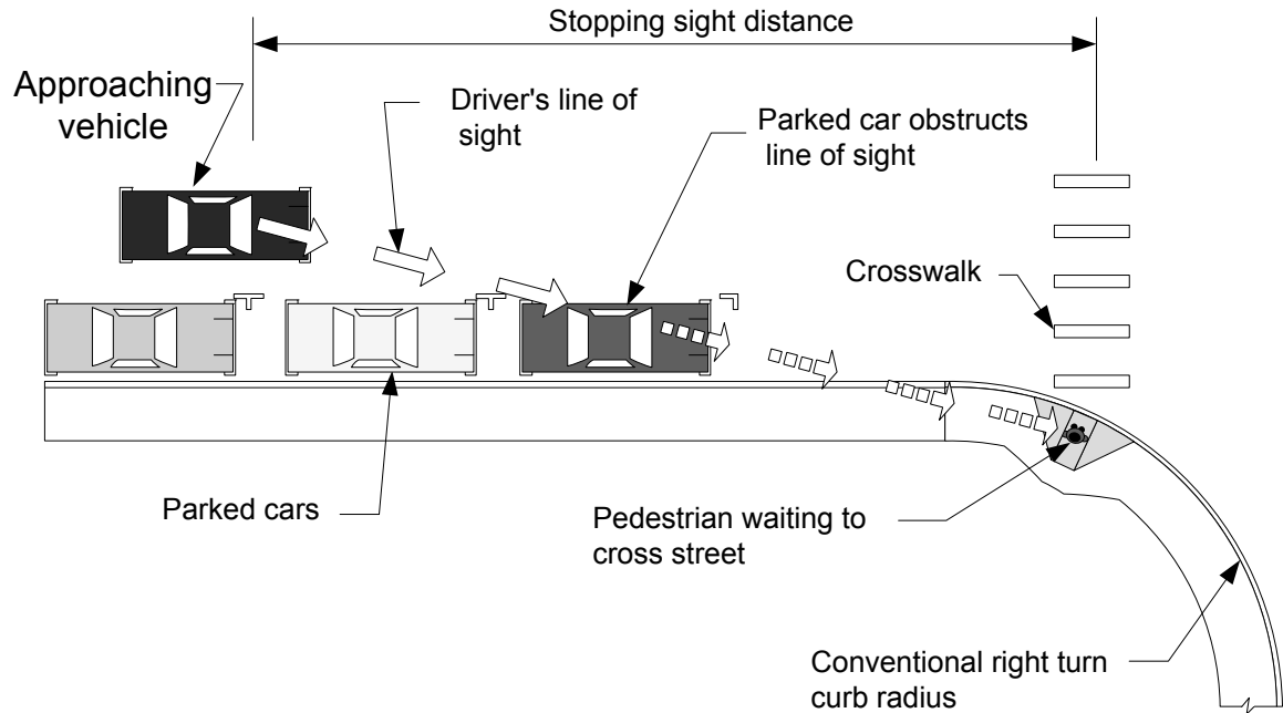
Parked car blocking line of sight
