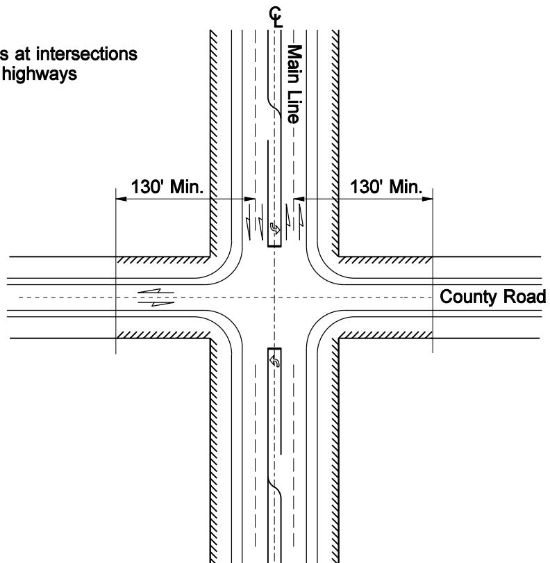
Modified Access Control Limits: Intersections Exhibit 530-3b
