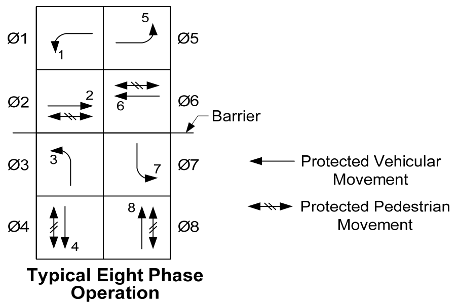
Standard Intersection Movements and Head Numbers Exhibit 1330-4
