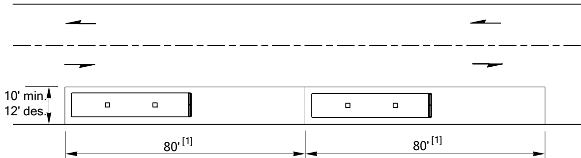
Parallel Design
