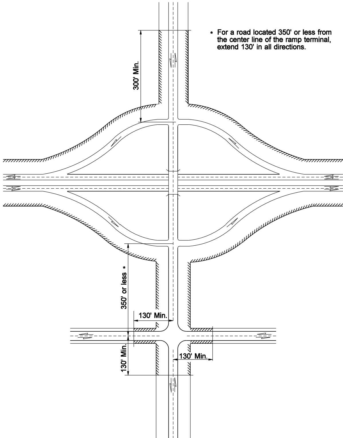
Full Access Control Limits: Interchange Exhibit 530-1a
