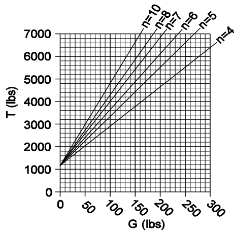
Chart 3 - Span Length 121' to 150'
