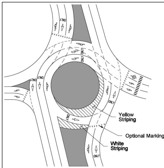
Multilane Roundabout Exhibit 1320-6c
