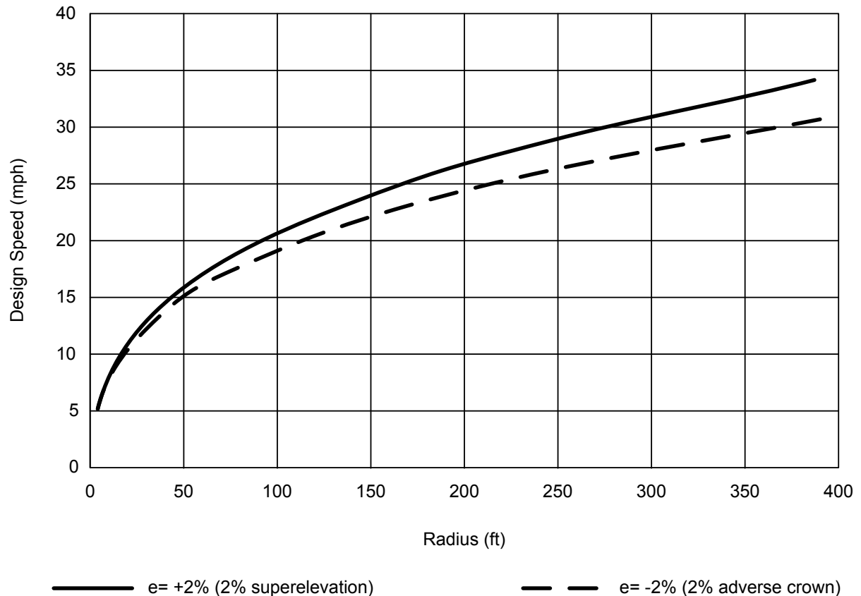
Speed vs. Radius Exhibit 1320-9
