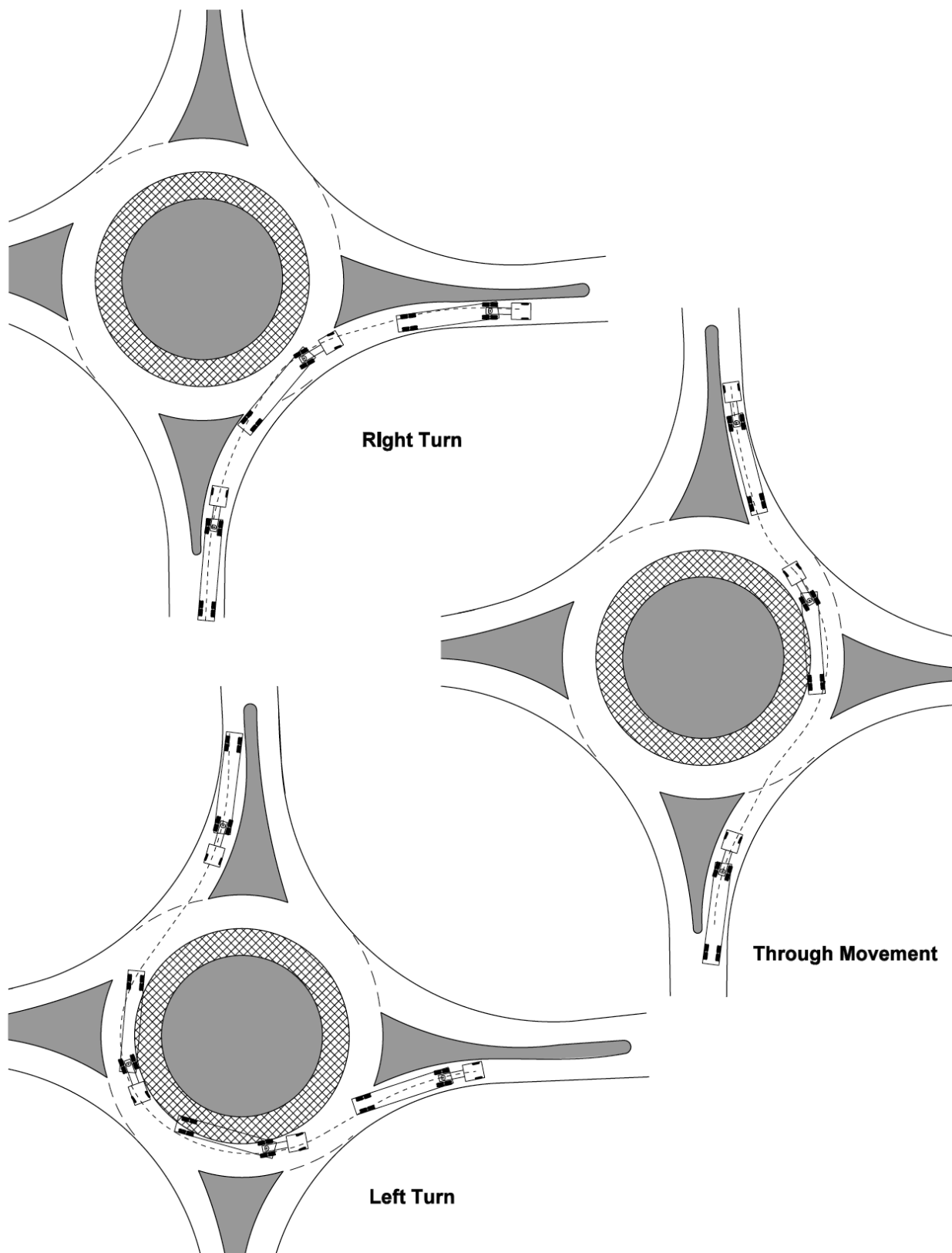
Truck Turning Paths Exhibit 1320-14a
