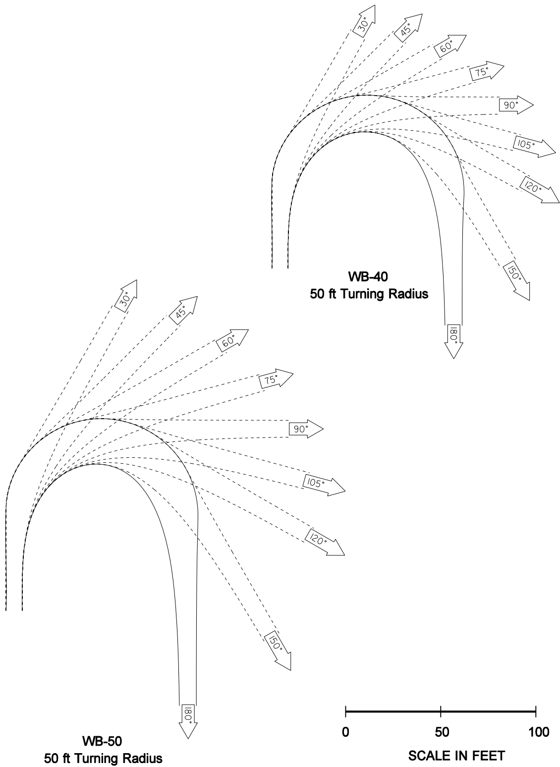
Turning Path Template Exhibit 1310-20b
