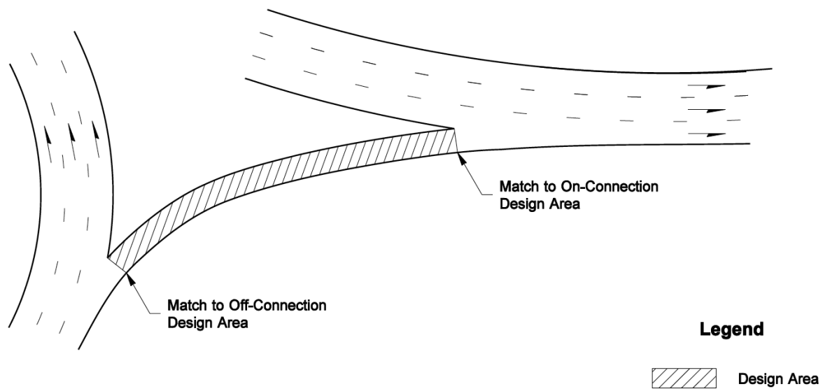
Freeway-to-Freeway Connection Exhibit 1040-4
