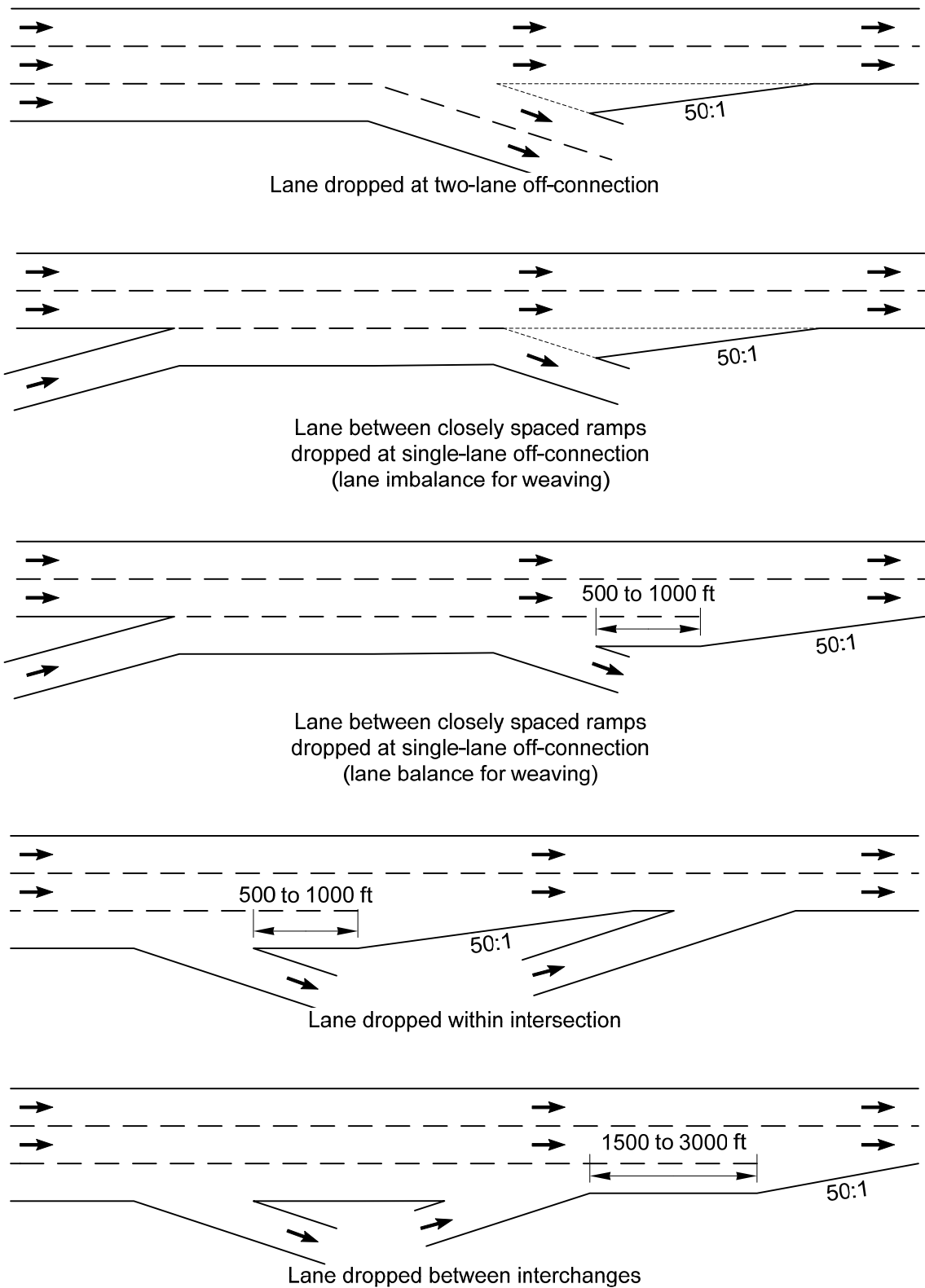
Main Line Lane Reduction Alternatives Exhibit 1360-8
