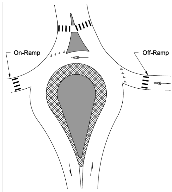
Teardrop Roundabout at Ramp Terminals
