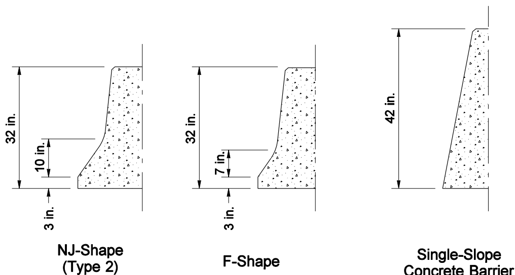
Concrete Barrier Shapes Exhibit 1610-7
