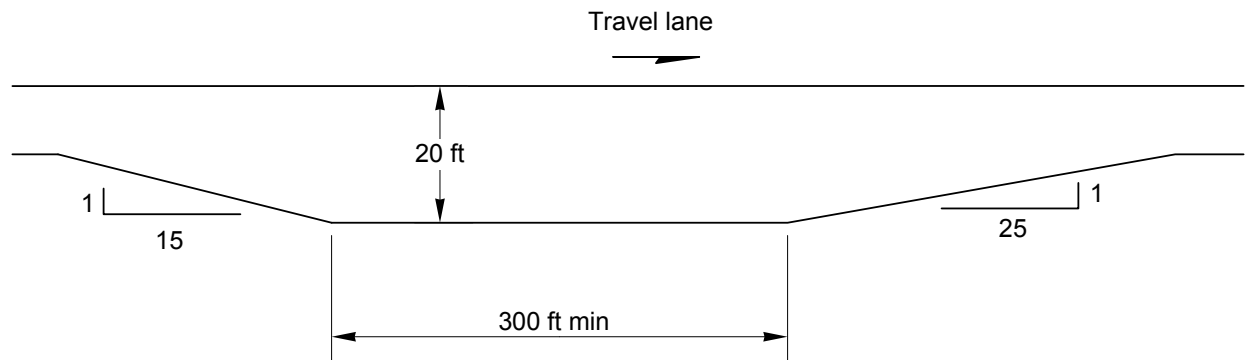
Large Shoulder Site Exhibit 1720-7
