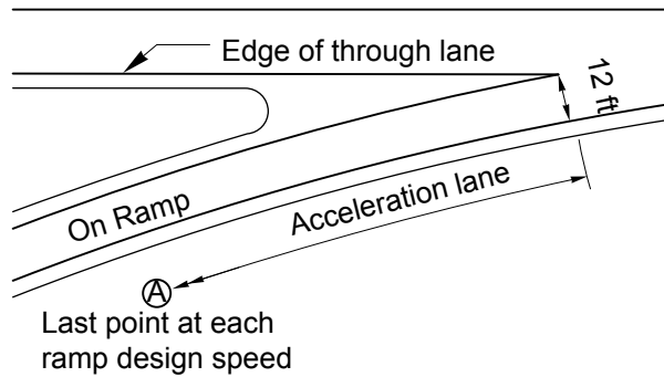
Tapered On-Connection
