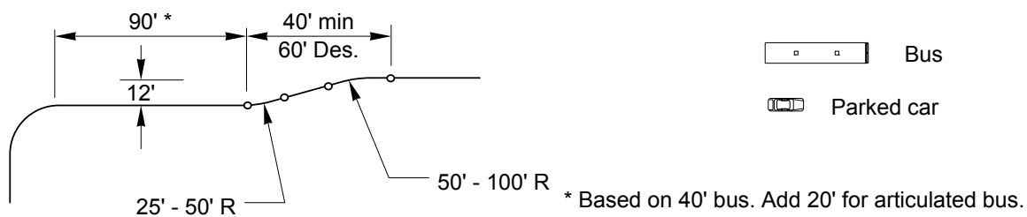
Far-Side Bus Pullout After Right Turn
