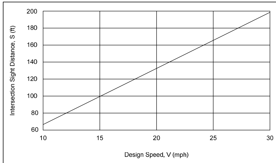
Speed vs. Intersection Sight Distance Exhibit 1320-12
