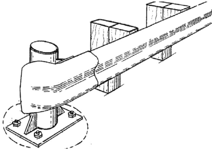
Old Type 3 Anchor Exhibit 1610-5
