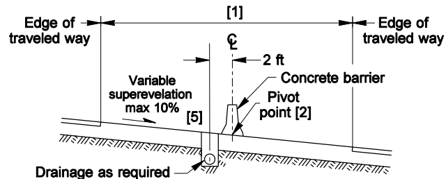
Alternate Design 1: Treatment on Curves
