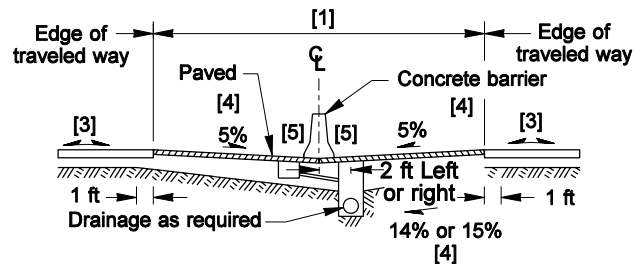
Design: B Depressed Median
