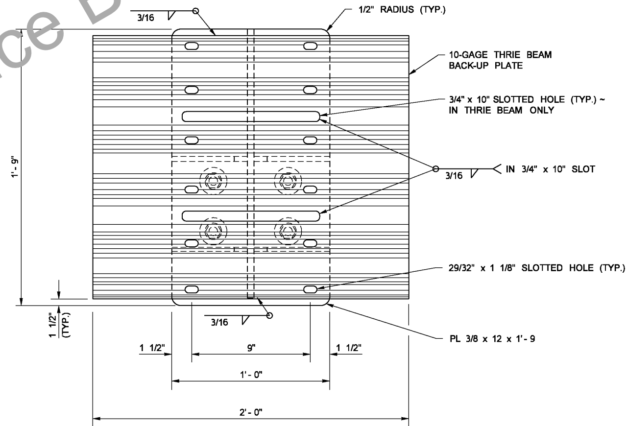
SECTION B
