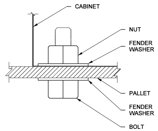
BOLT ASSEMBLY DETAIL
