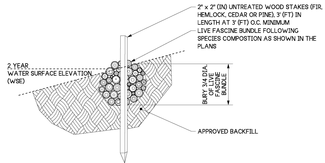
LIVE FASCINE BUNDLE TYPICAL
