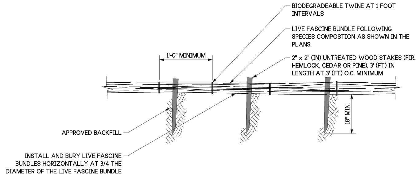
LIVE FASCINE BUNDLE SECTION
