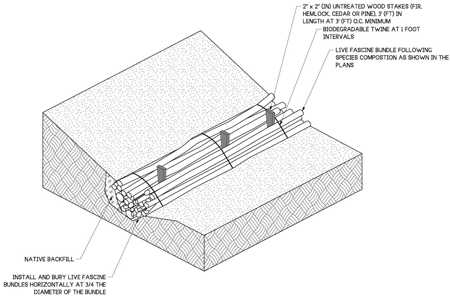
LIVE FASCINE BUNDLE ISOMETRIC
