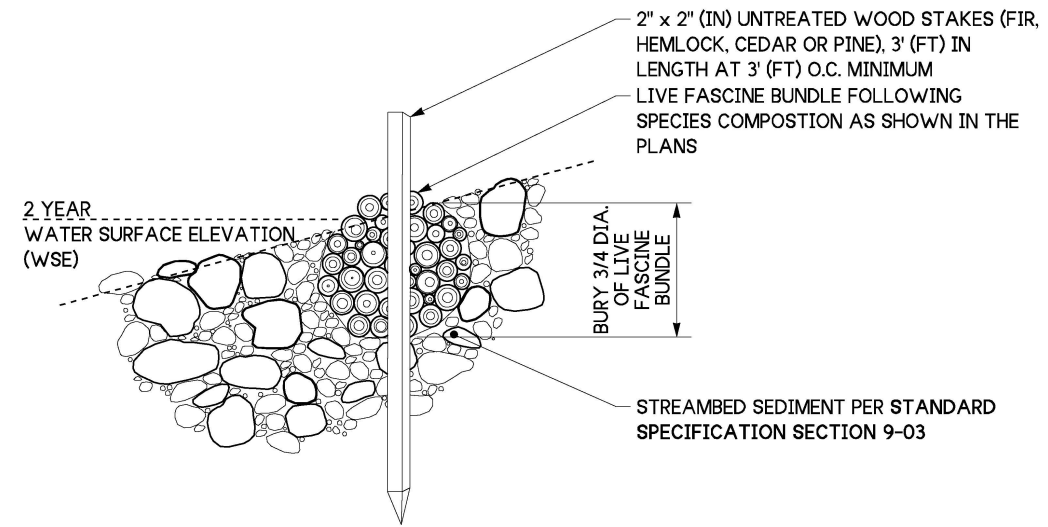
LIVE FASCINE BUNDLE IN STREAMBED SEDIMENT
