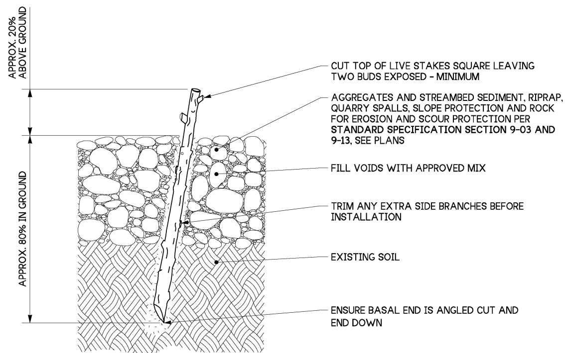
LIVE STAKE INSTALLATION IN ROCK
