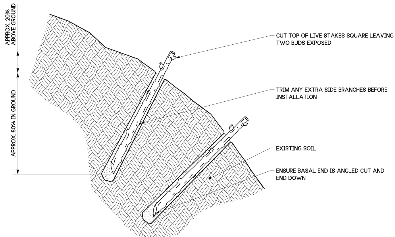
LIVE STAKE INSTALLATION ON SLOPES
