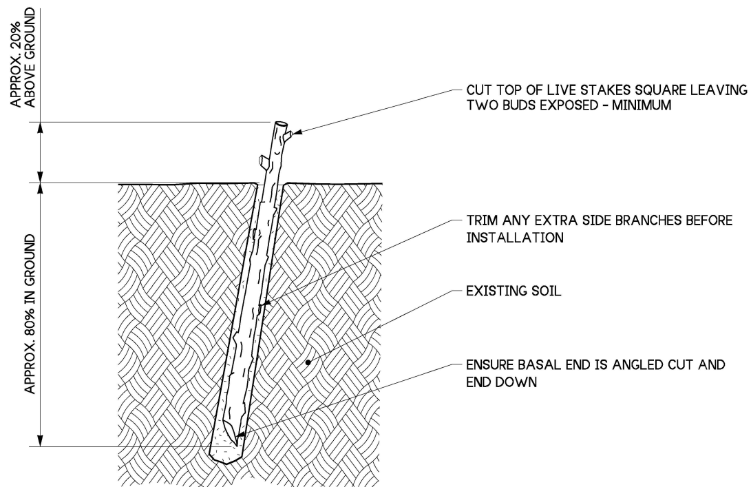
TYPICAL LIVE STAKE INSTALLATION
