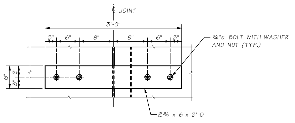
VIEW C LONGITUDINAL TIE
