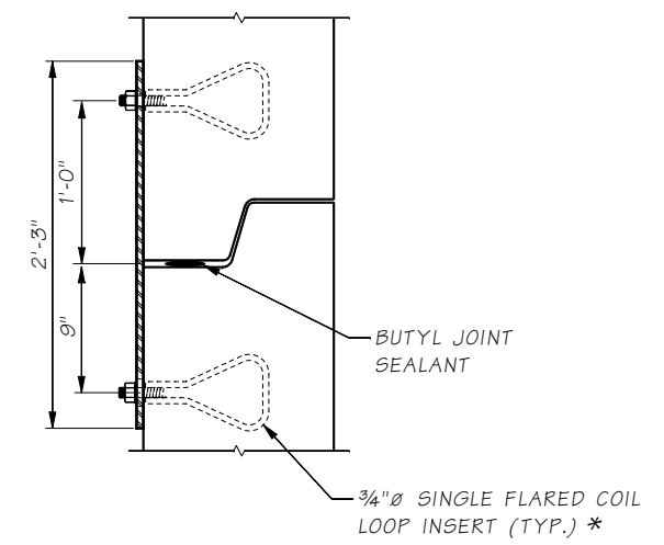
SECTION B REINFORCING NOT SHOWN FOR CLARITY.
