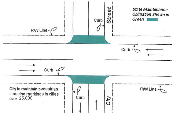
NORMAL INTERSECTION EXISTING STATE HIGHWAY Figure 1
