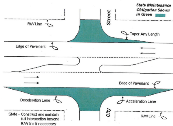
EXISTING CITY STREET CROSSED AT GRADE BY NEW STATE HIGHWAY Figure 4
