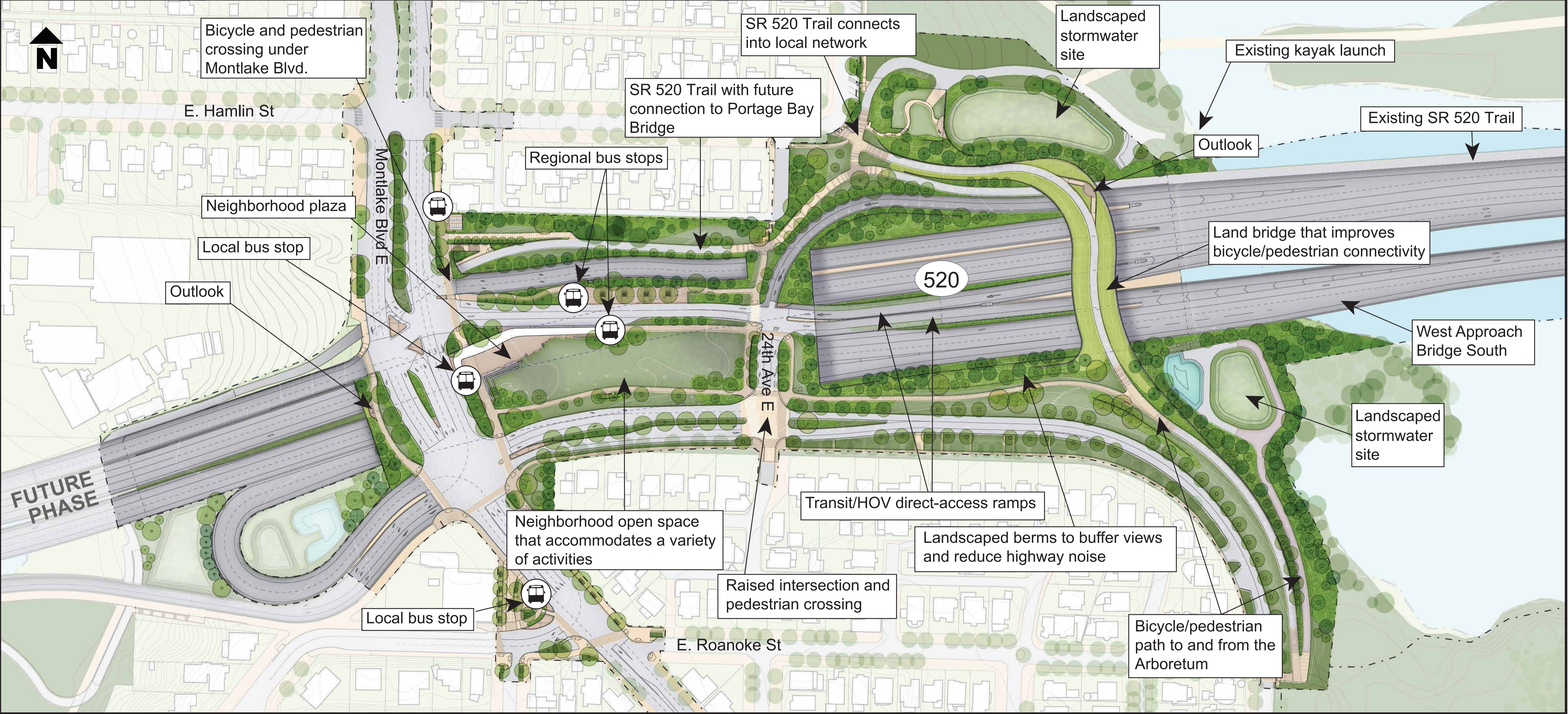
Note: Graphic depicts SR 520 corridor elements at completion. Major elements of the Montlake Project are labeled above.
