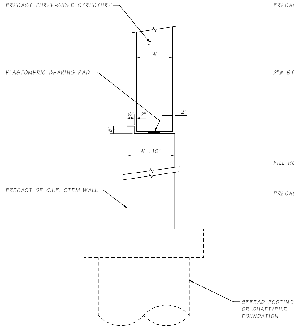
BEARING
