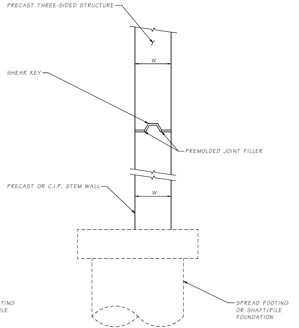
SHEAR KEY
