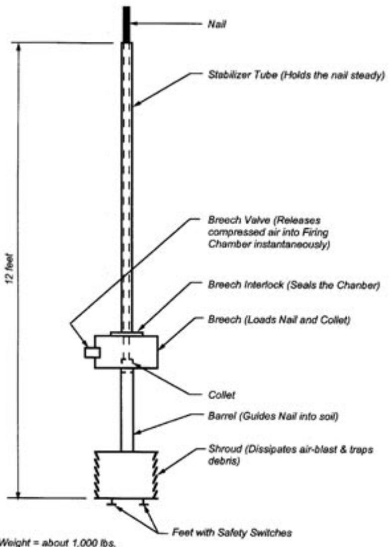
SCHEMATIC OF SOIL NAIL LAUNCHER Source: Application Guide for Launched Nails-Volume 1, FHWA-FPL-93-003, July 1994
