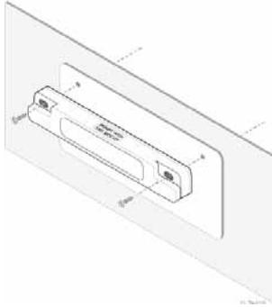
Figure 2: Transponder Placement on License Plate and Bumper
