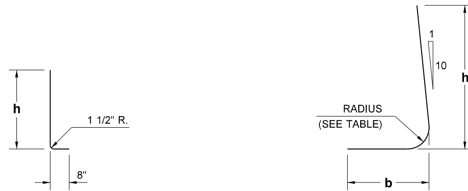
BAR (E) @ 1' - 6" CENTERS
