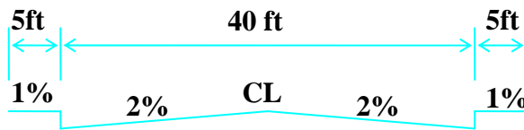
Figure 2 - CROSS SECTION
